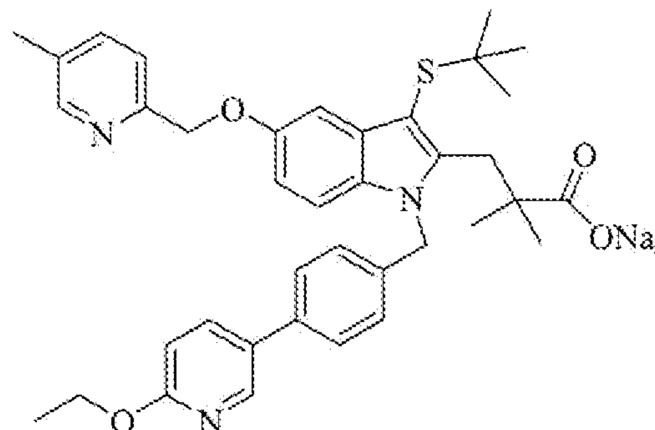
Compound 2.
