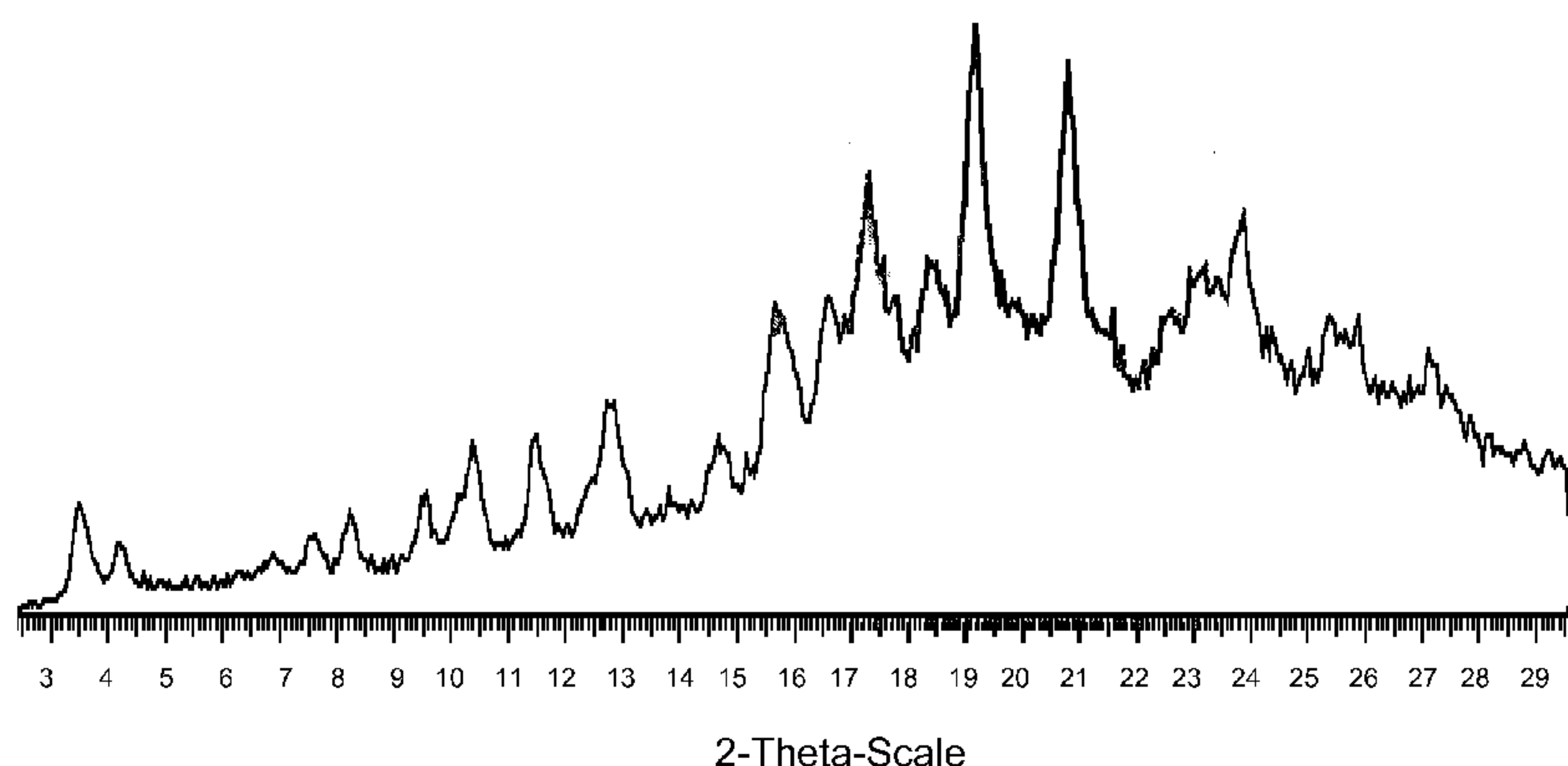
Figure 1. Polymorph Form C
