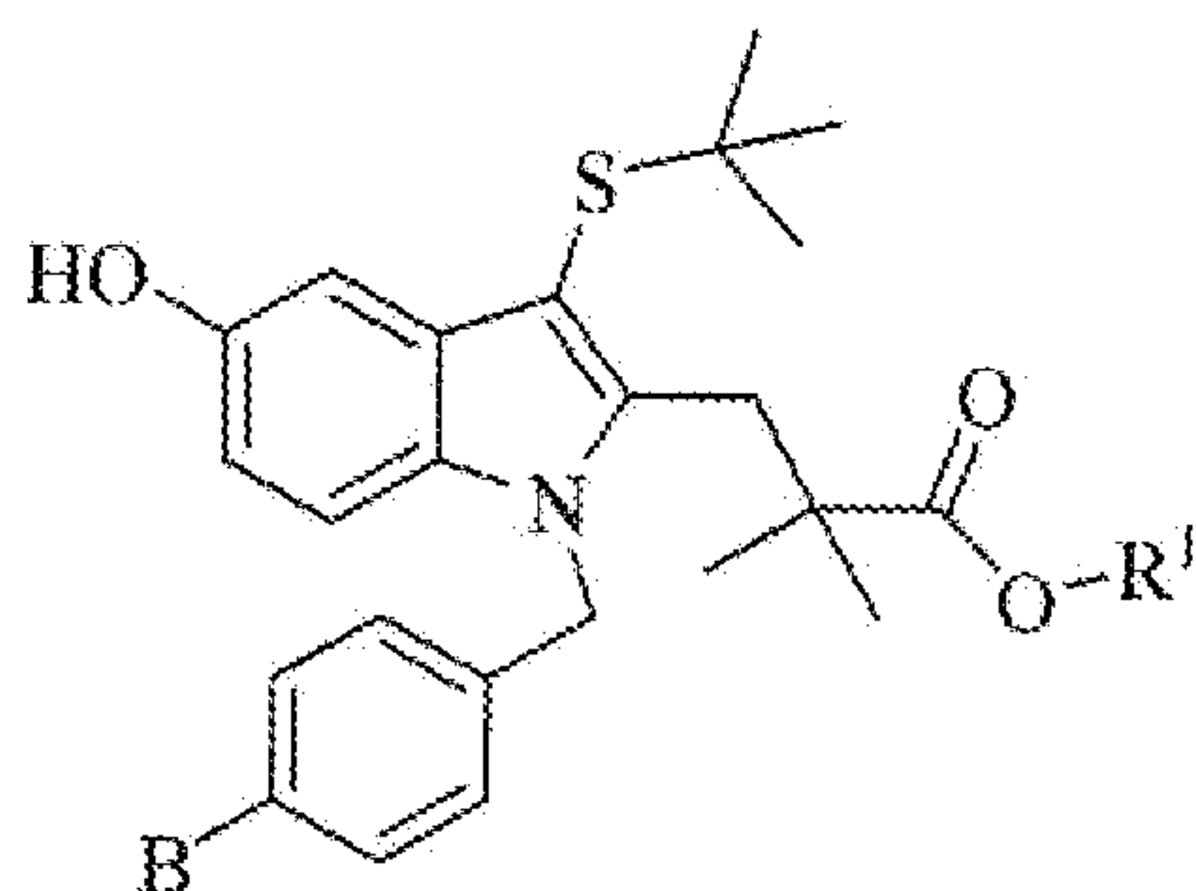
Formula (IV),
