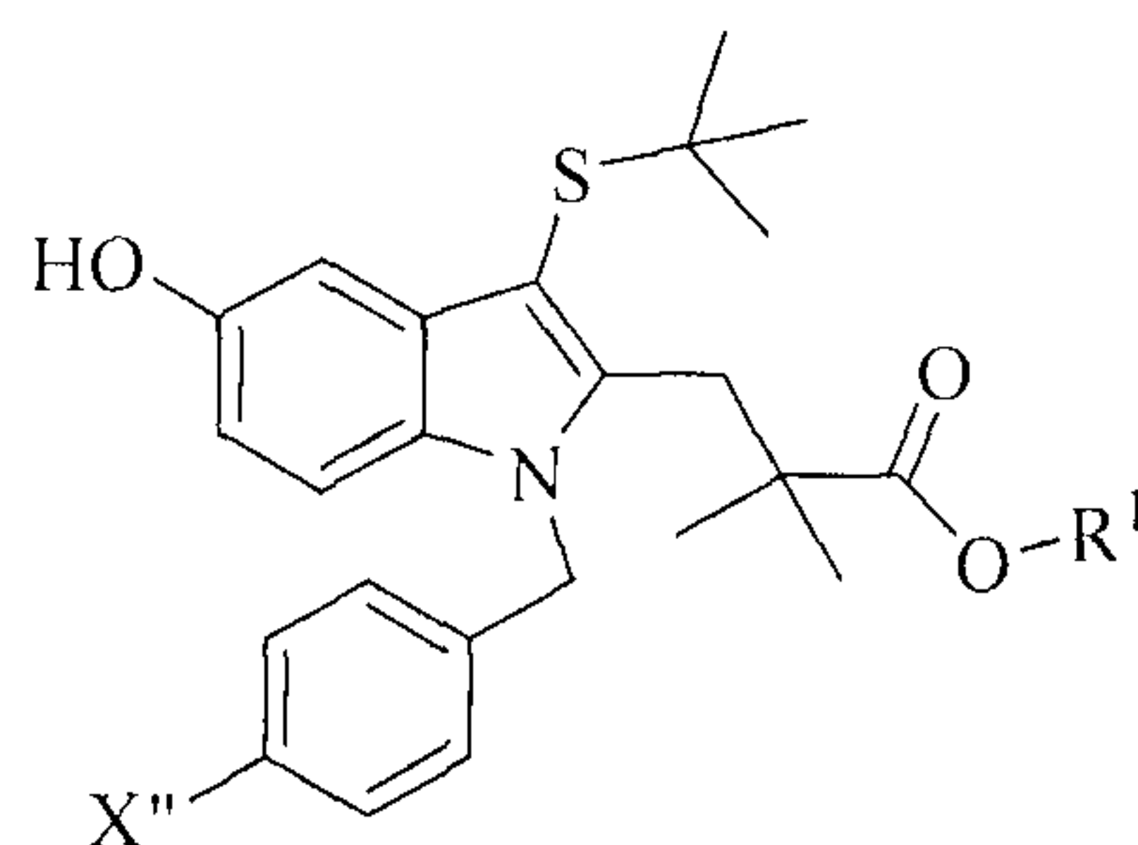
Formula (VI).
