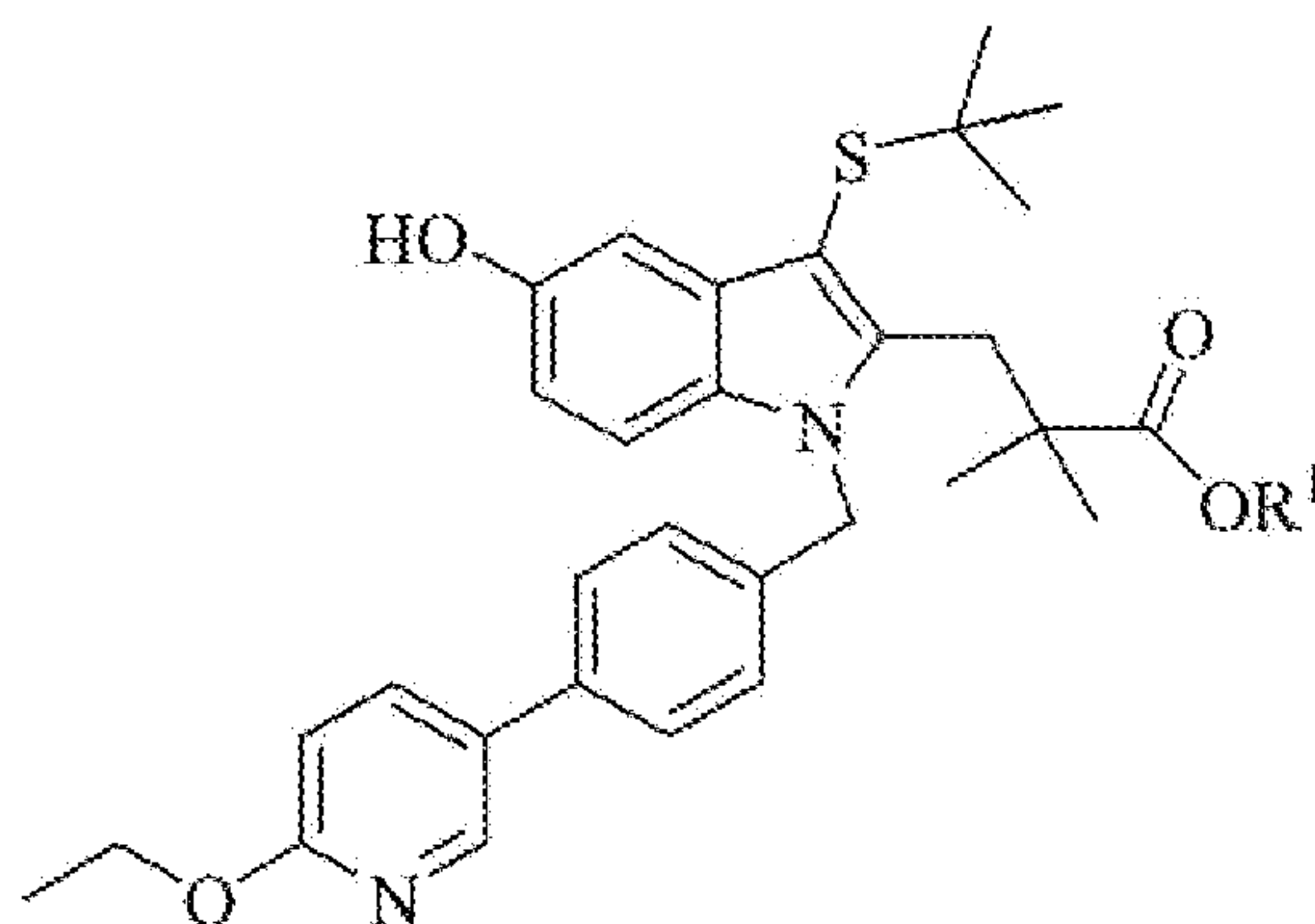
Formula (III).
