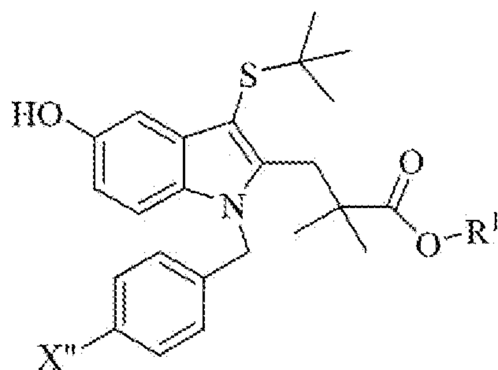
Formula (VI).
