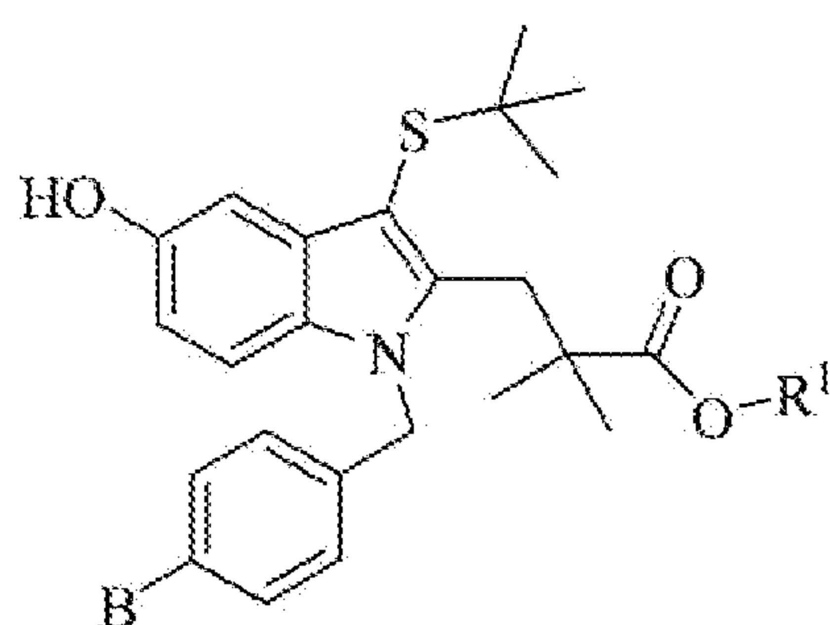
Formula (IV).
