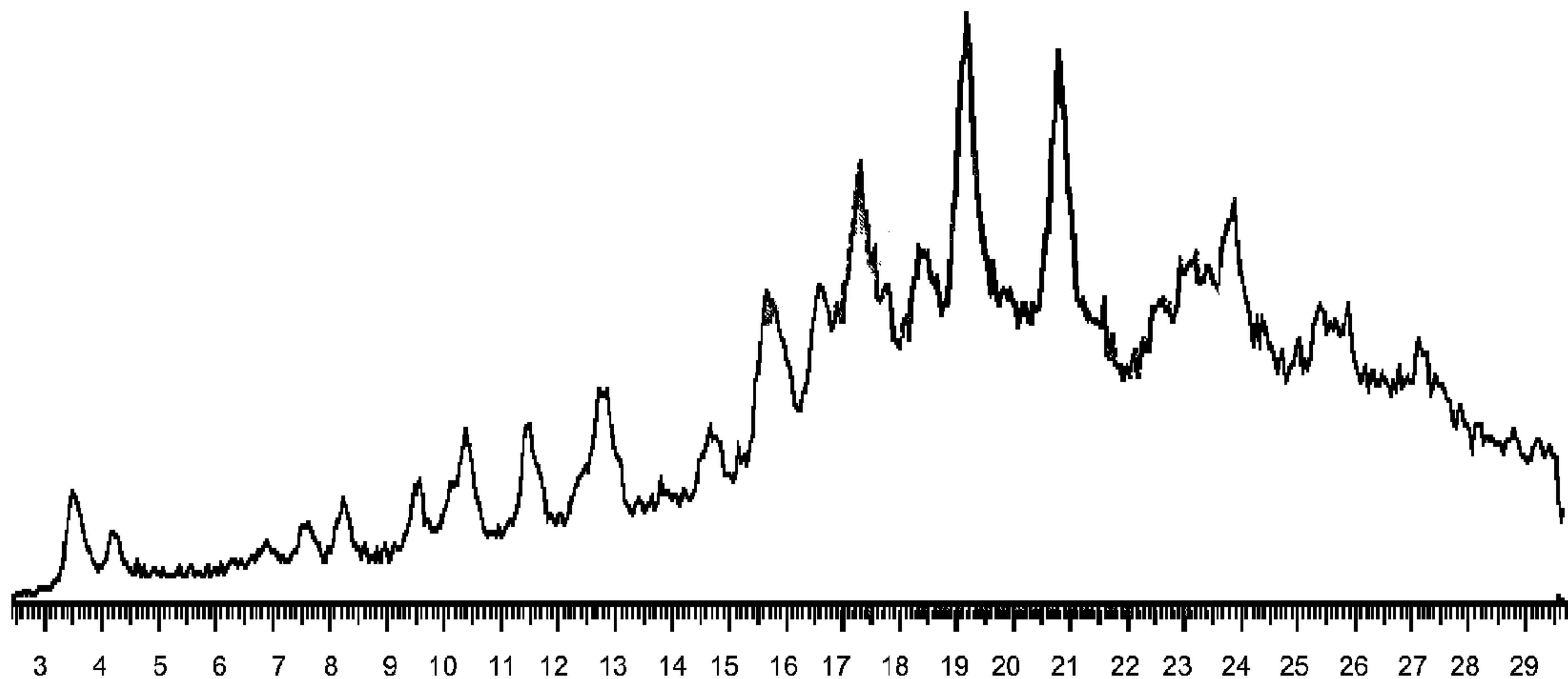
2-Theta-Scale Polymorph Form C
