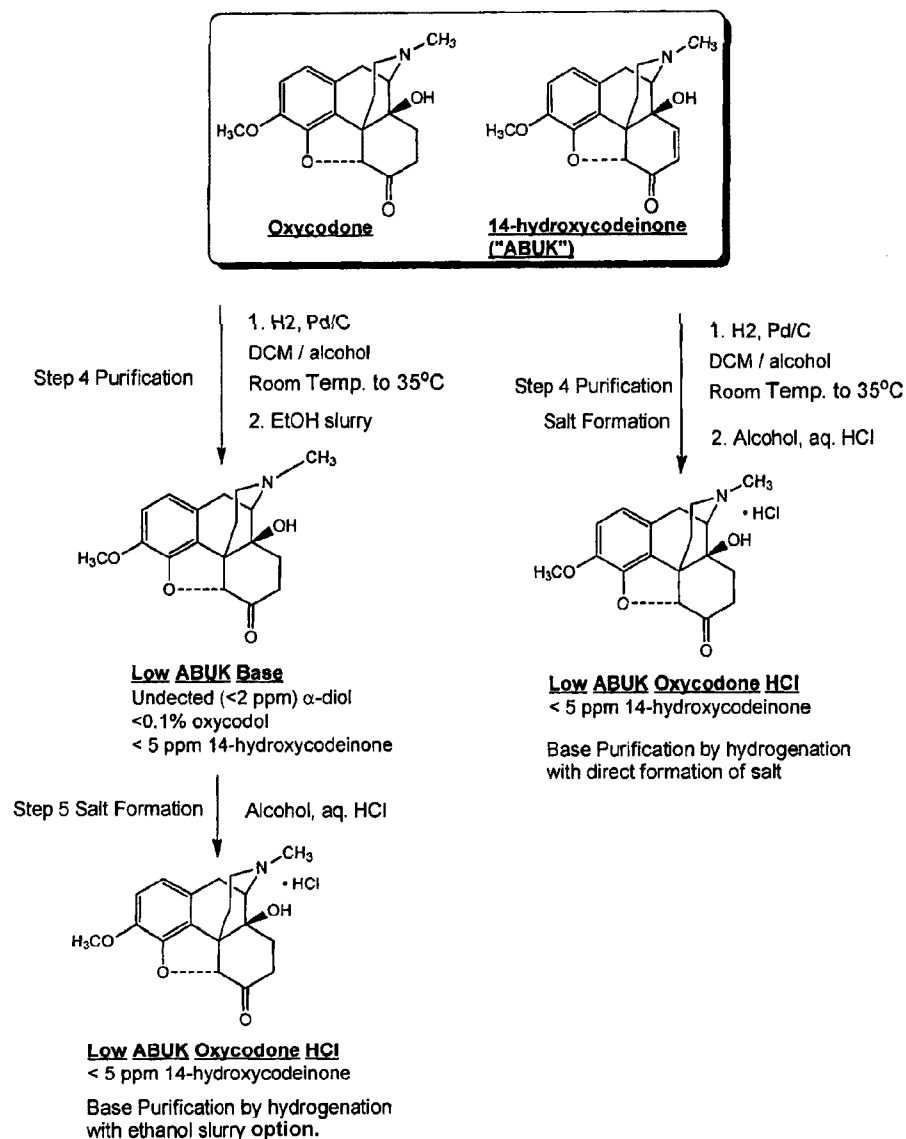
Scheme 2: Alternative Routes from Crude Oxycodone Base to Low ABUG Oxycodone HCl
