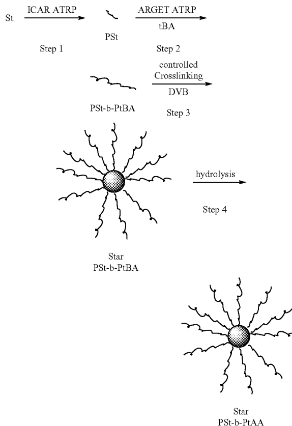
Scheme 3. Multistep synthesis of PSt-b-PAA block copolymer stars
