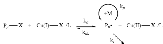
Atom transfer radical polymerization (ATRP)
