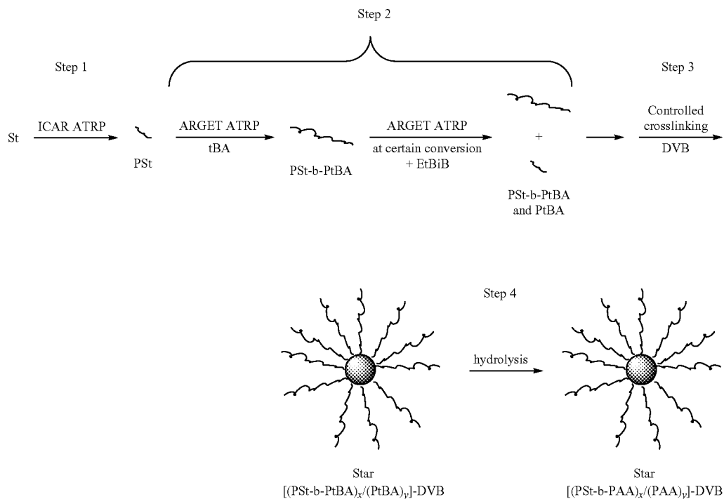
Scheme 4. Multistep synthesis of [PSt-b-PAA/PAA] miktoarm stars copolymers
