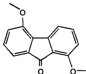
1,5-isomer (minor product)
