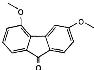
3,5-isomer (major product)
