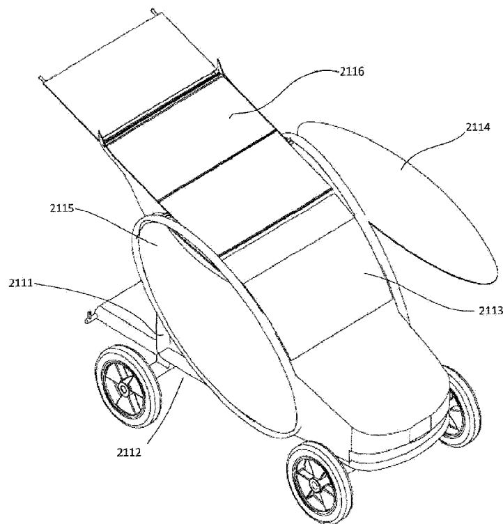
Figure 8 Early Embodiment of Monarch EV with Flexible Chassis and Foldable Sides
