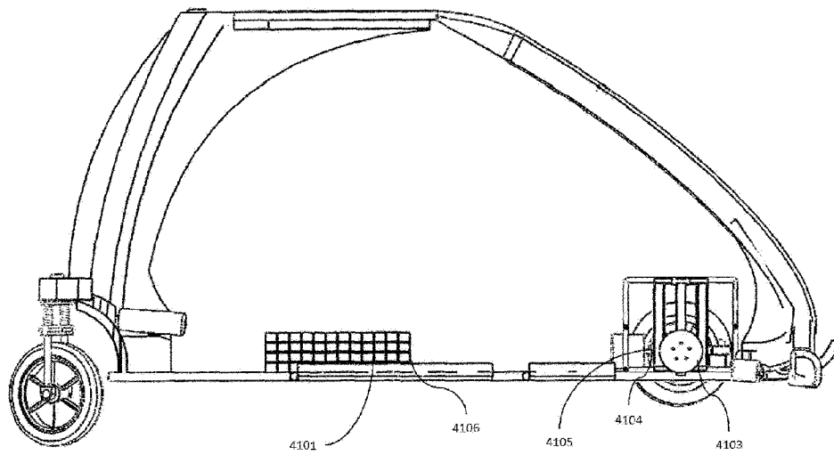
Figure 17 Electrical component locations in an EV
