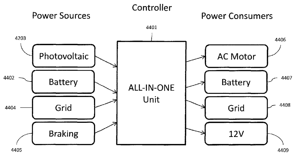
Figure 18 All-in-one Power Unit
