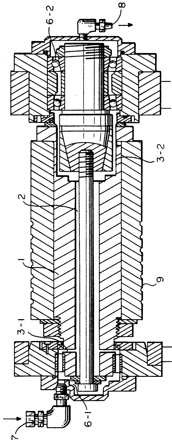
FIG. 7 PRIOR ART
