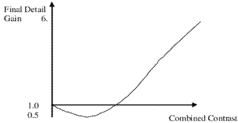
Fig. 6 (Combined Contrast to Watermark Gain Mapping Function)
