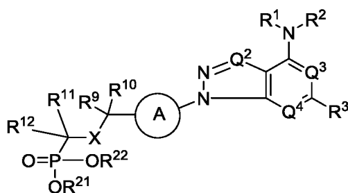
Formula (IV);
