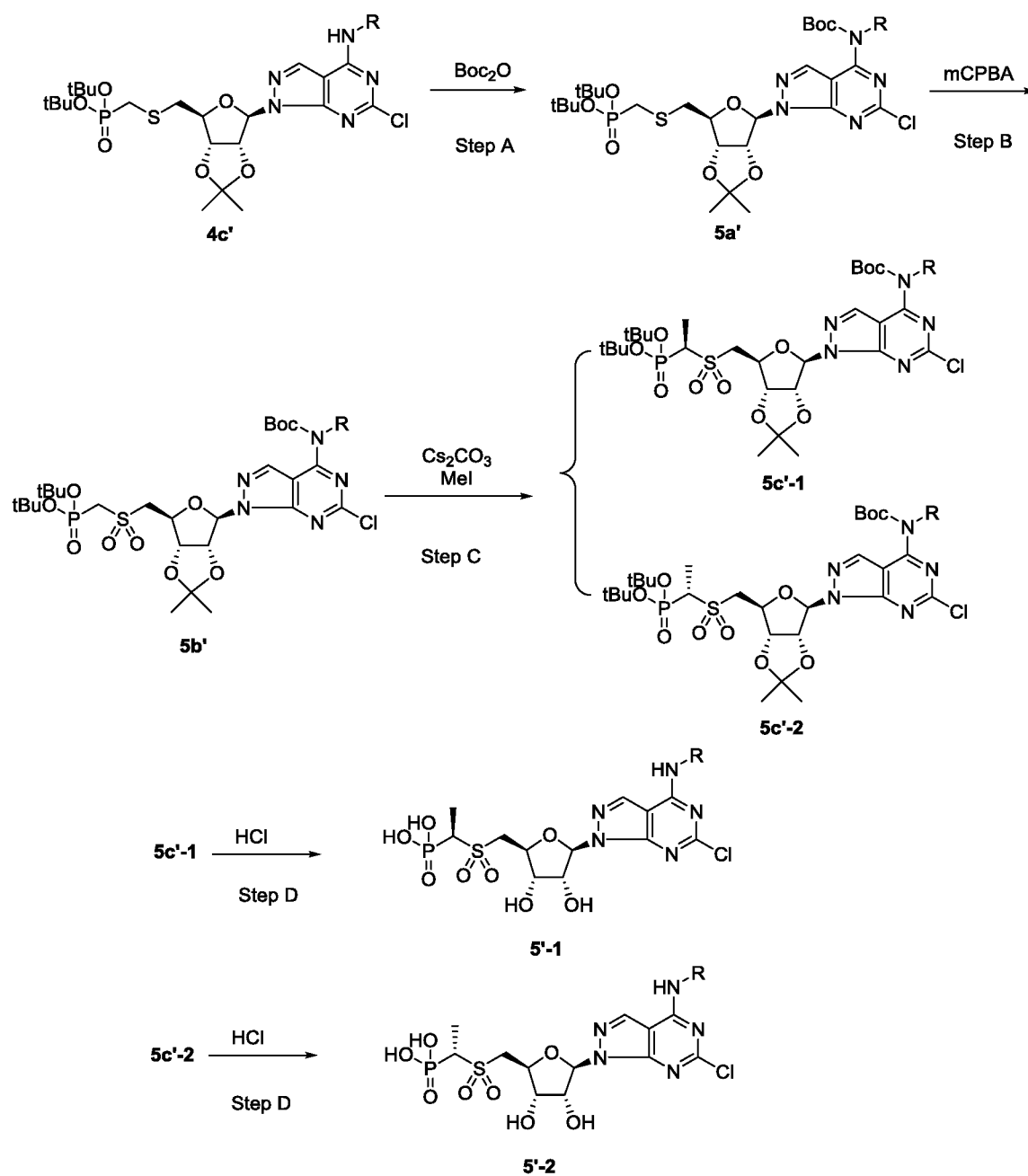
Scheme 6
