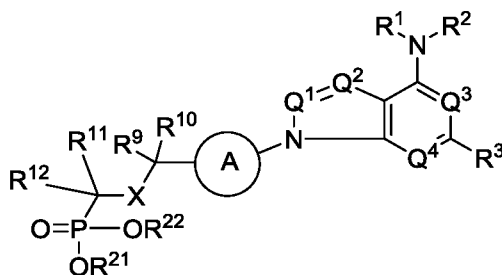
Formula (III);
