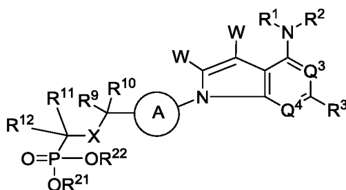
Formula (V);
