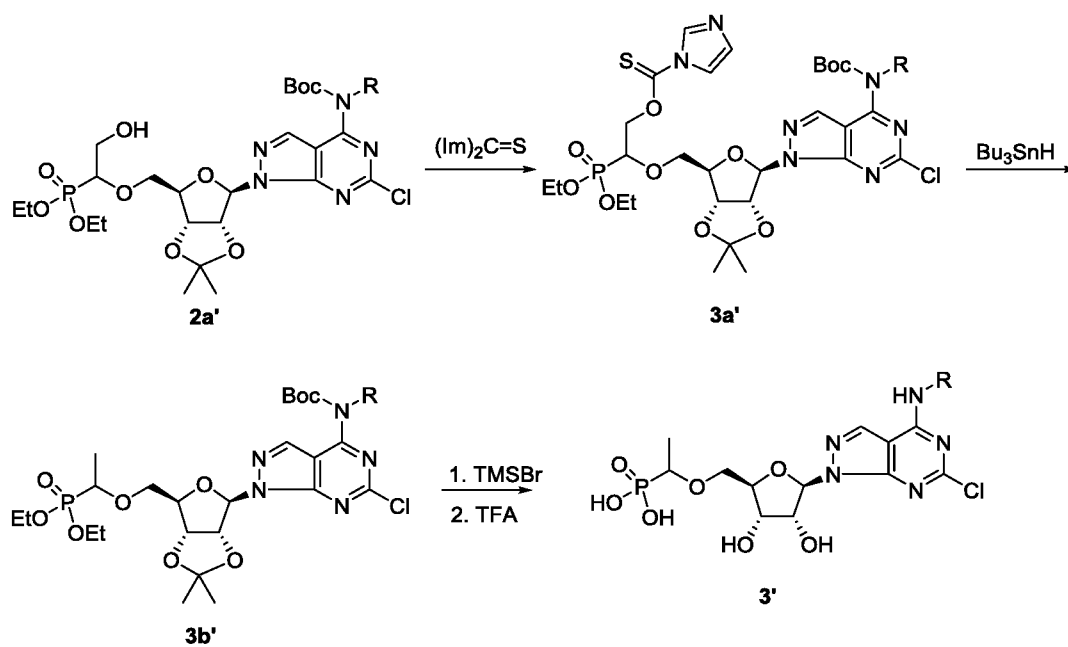
Scheme 4
