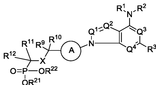
Formula (I);
