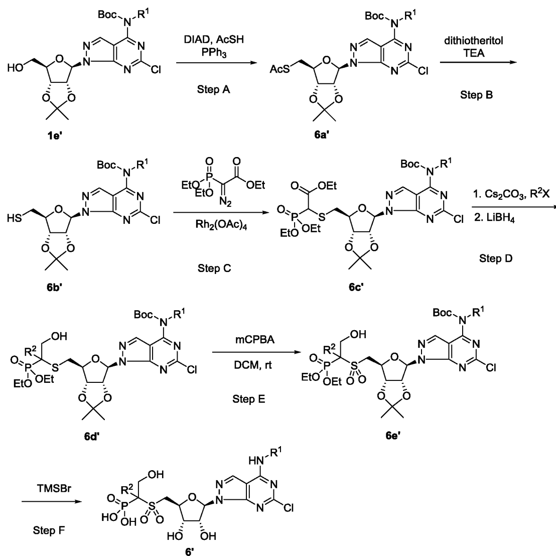
Scheme 7
