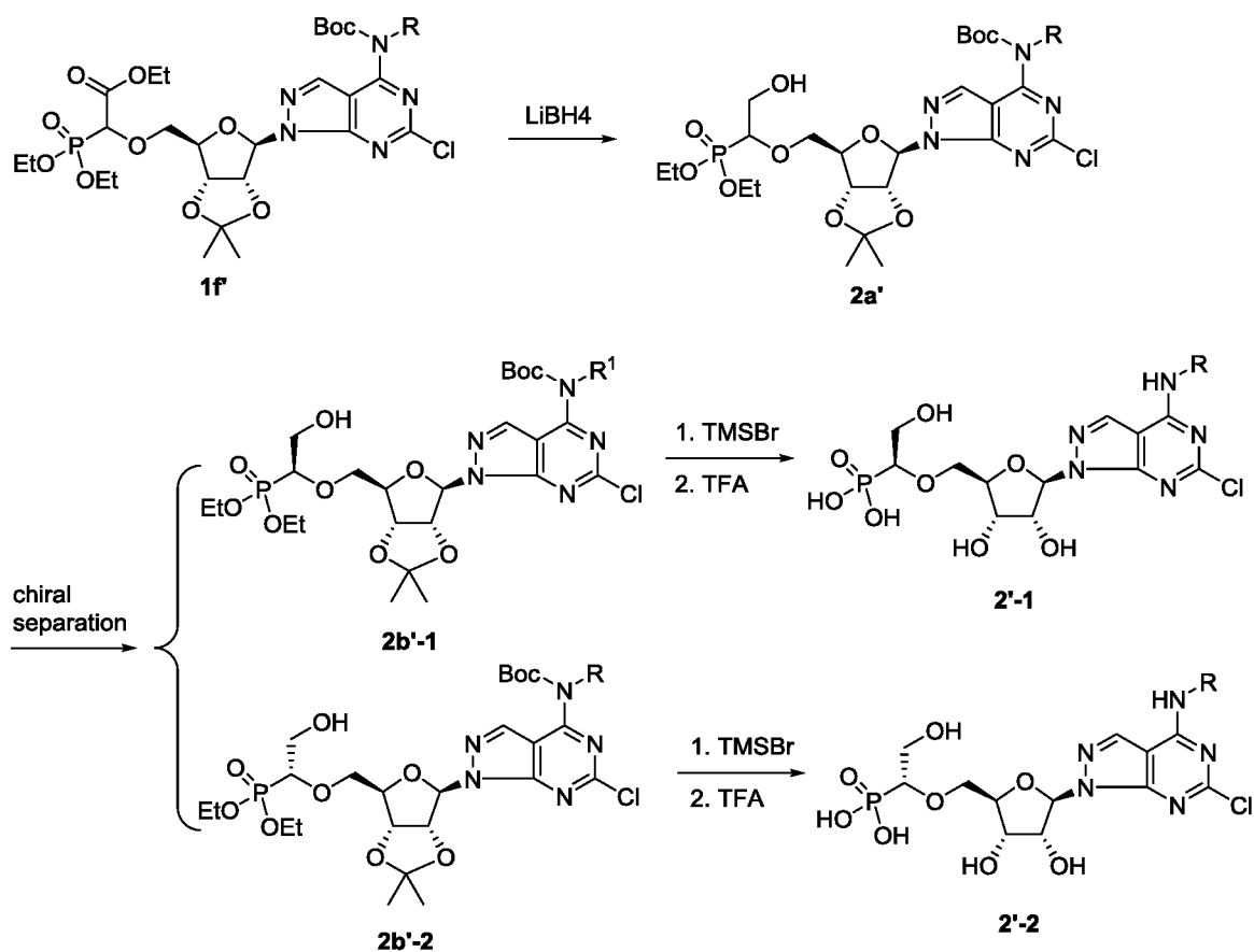
Scheme 3
