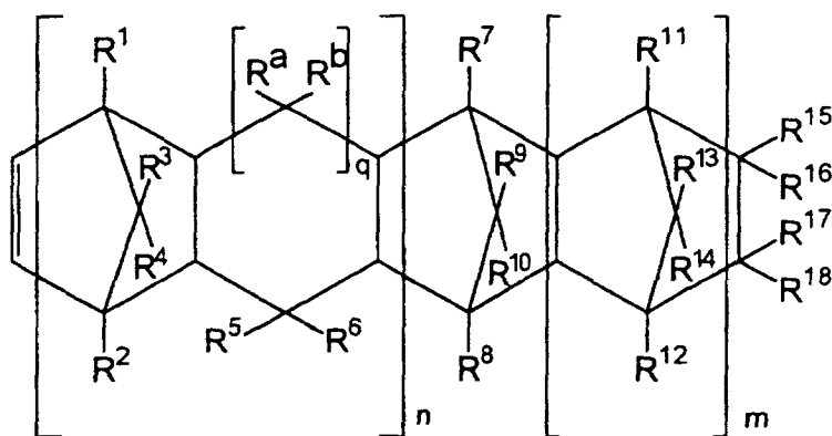
Formel (II)
