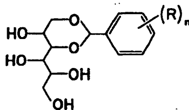
Formula (I-c)
