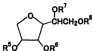
Formula (I-e)
