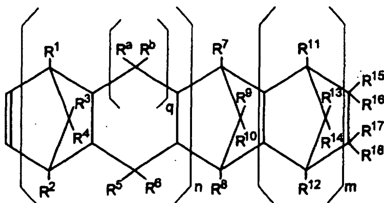
Formula (II)
