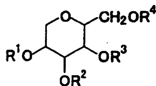
Formula (I-d)
