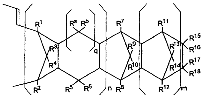
Formula (VI)
