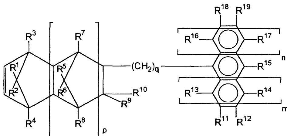
Formel (III)
