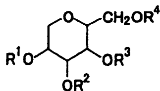
Formula (I-d)
