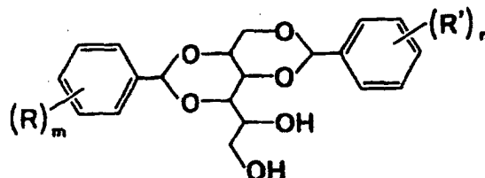
Formula (I-a)
