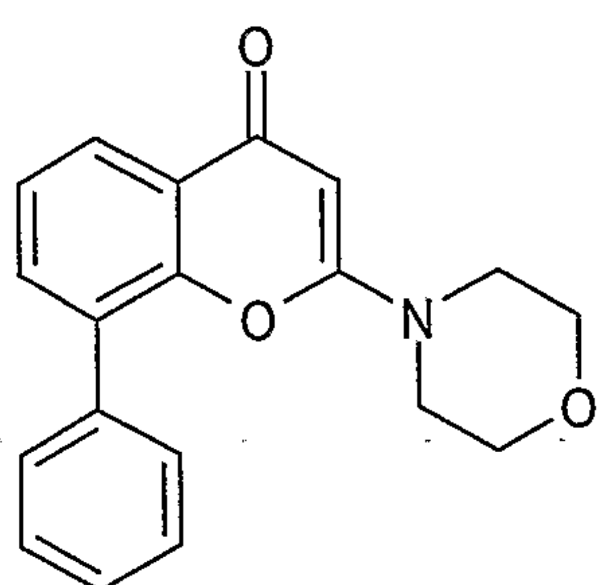
LY 294002
