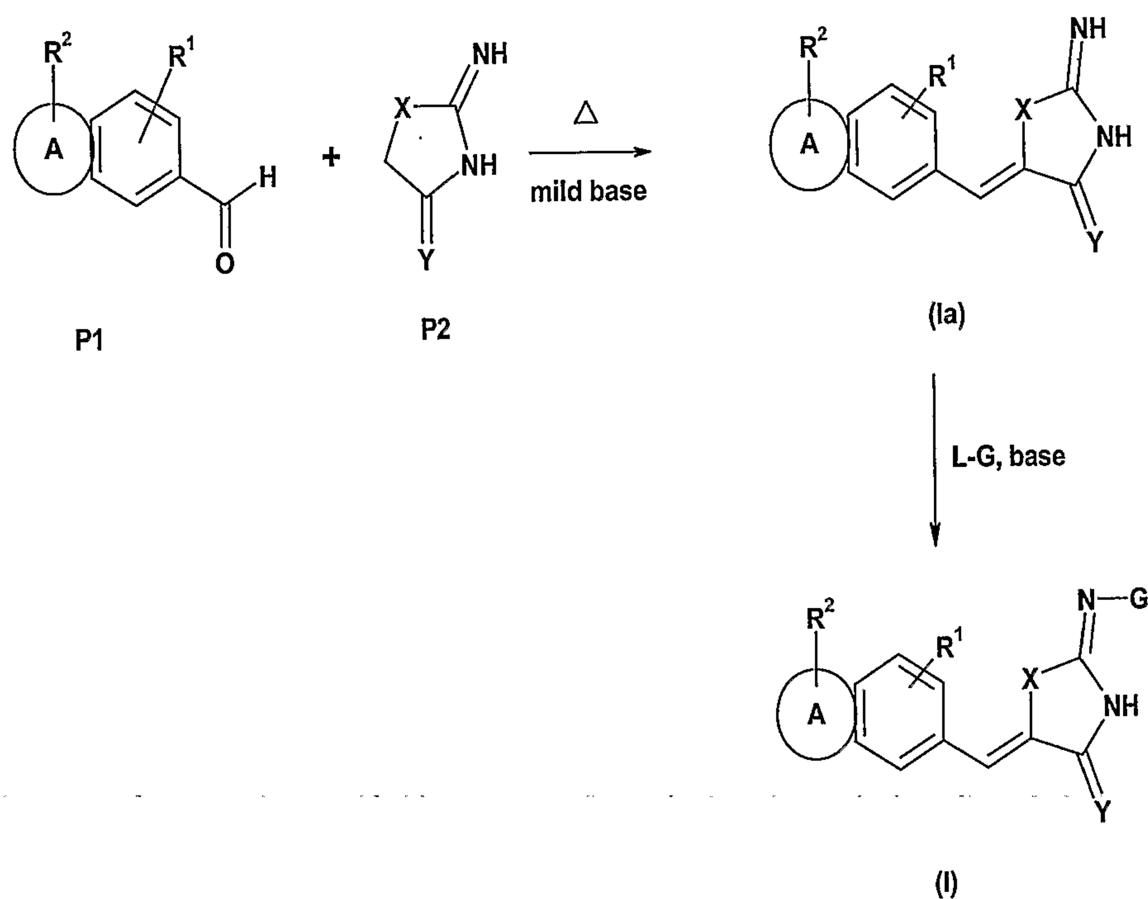
Scheme 1
