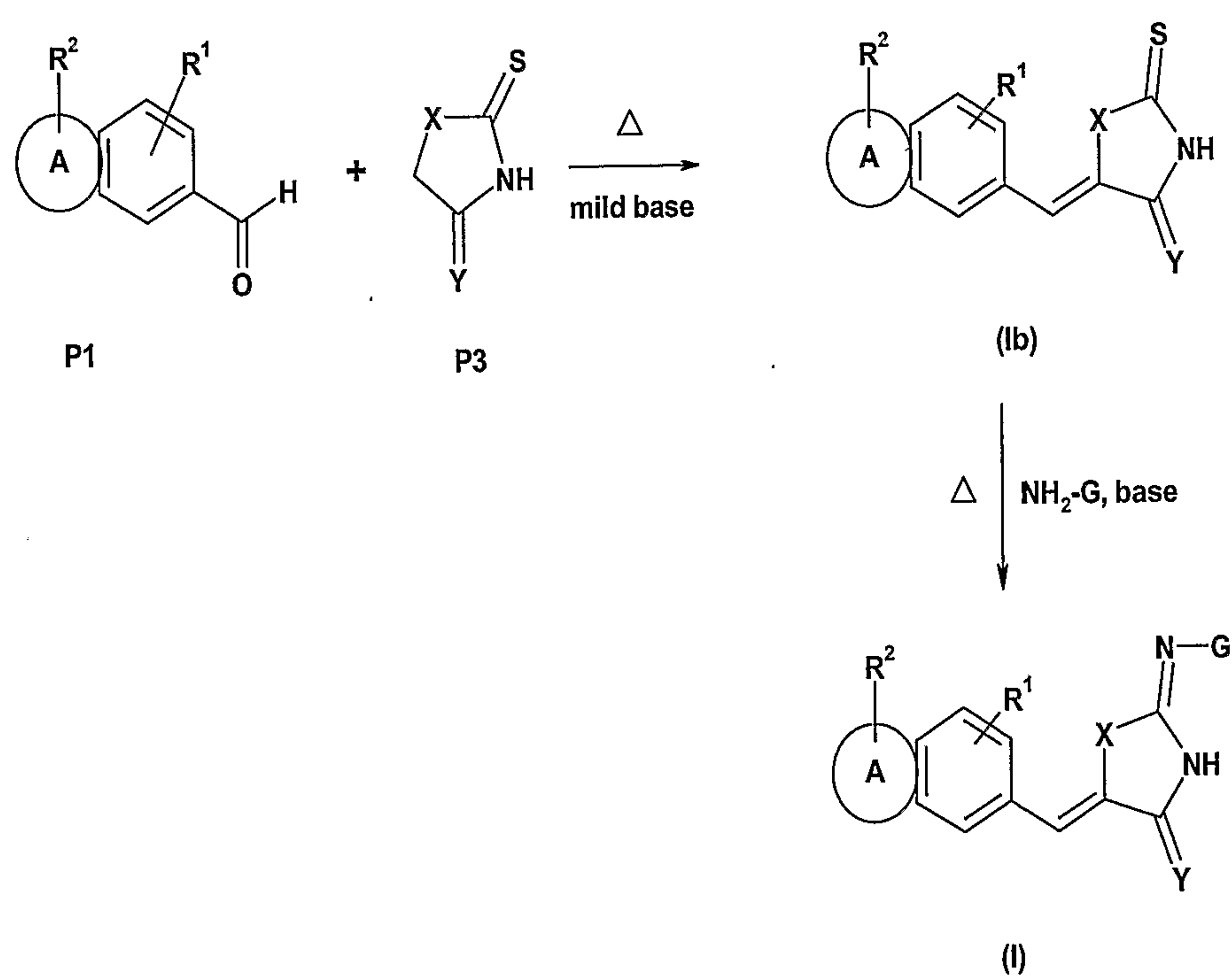
Scheme 2
