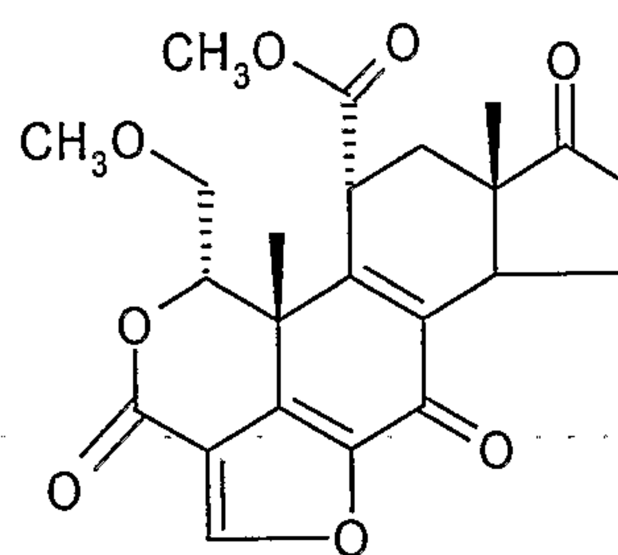
Wortmannin
