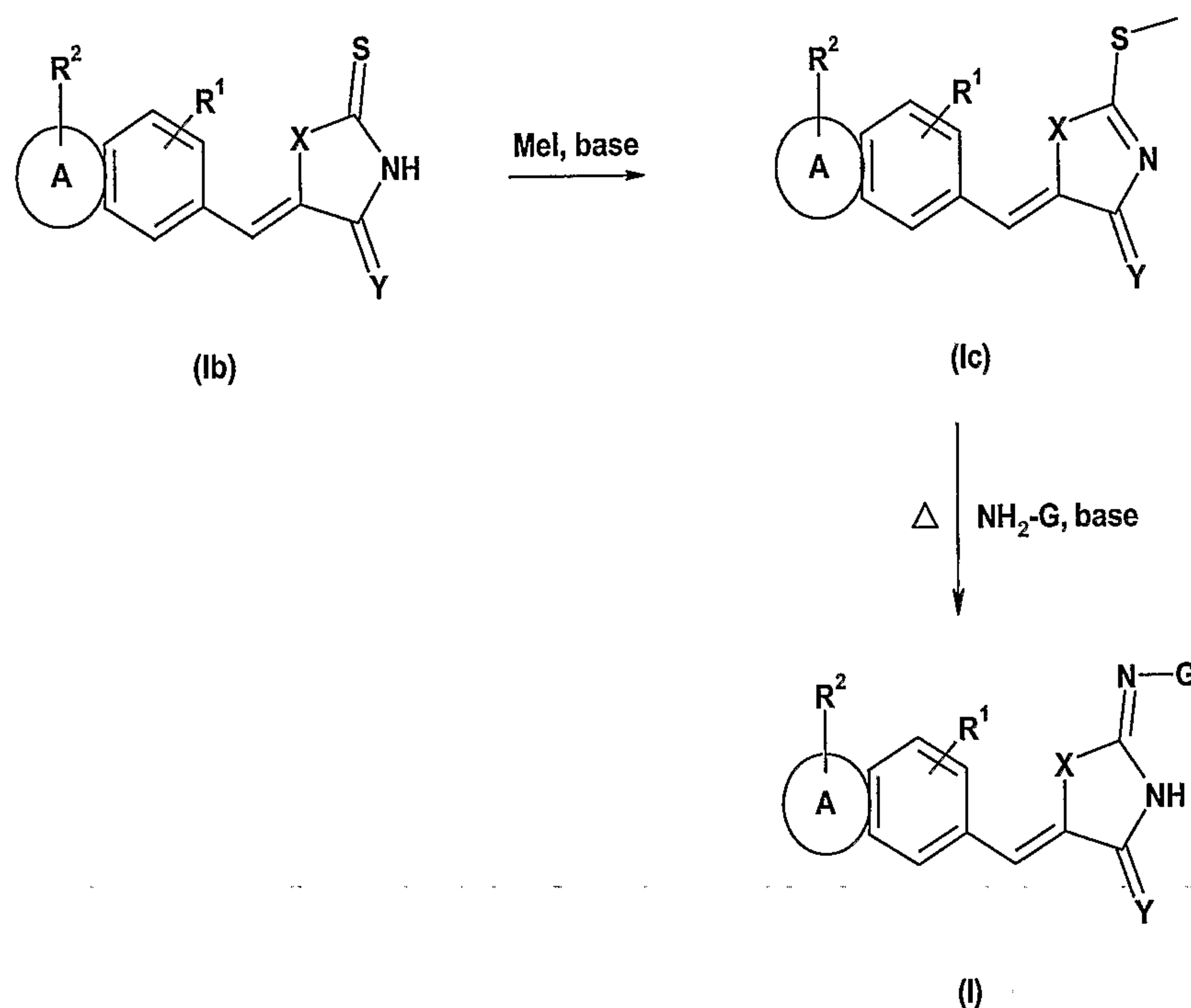
Scheme 3
