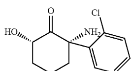
2S,6S-hydroxynorketamine
