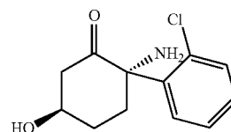
2S,5R-hydroxynorketamine,
