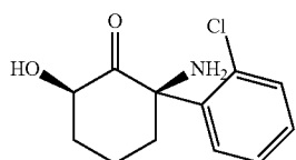
2R,6R-hydroxynorketamine,
