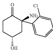
2R,4S-hydroxynorketamine,
