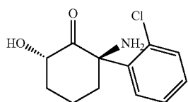
2R,6S-hydroxynorketamine,
