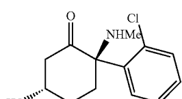
2R,5S-hydroxyketamine,
