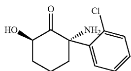
2S,6R-hydroxynorketamine,
