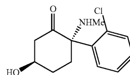
2S,5R-hydroxyketamine,
