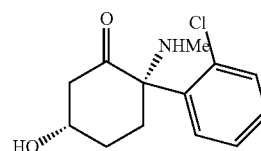
2S,5S-hydroxyketamine
