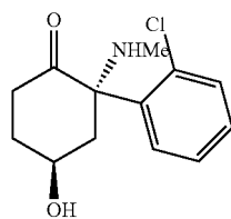
2S,4R-hydroxyketamine,
