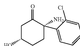
2S,5S-hydroxynorketamine
