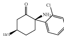
2R,5R-hydroxynorketamine,
