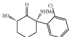
2S,6S-hydroxyketamine
