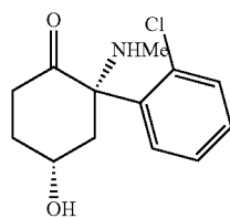
2S,4S-hydroxyketamine
