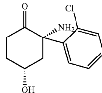
2S,4S-hydroxynorketamine
