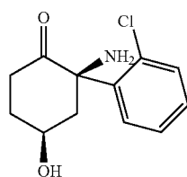
2R,4R-hydroxynorketamine,
