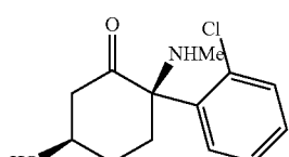
2R,5R-hydroxyketamine,
