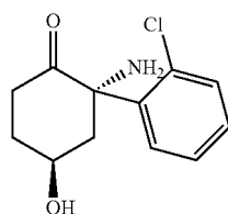
2S,4R-hydroxynorketamine,
