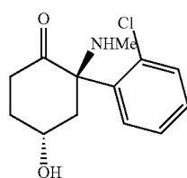
2R,4S-hydroxyketamine,
