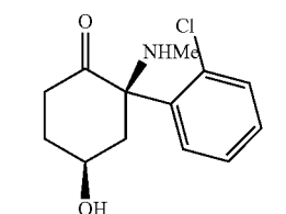
2R,4R-hydroxyketamine,
