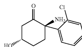
2R,5S-hydroxynorketamine,
