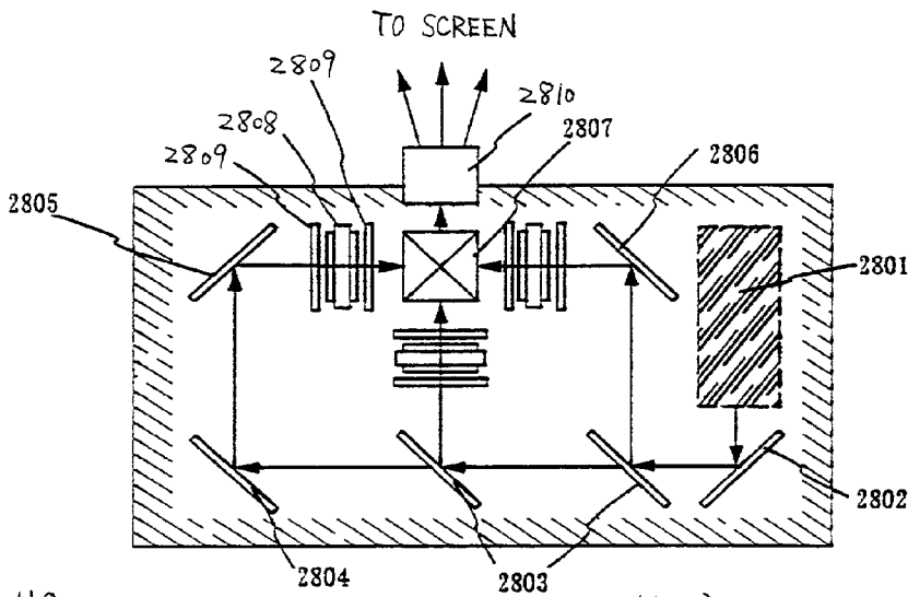
FIG. 11C PROJECTION SYSTEM (3-PLATE TYPE)
