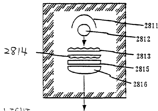
FIG. 11C PROJECTION SYSTEM (3-PLATE TYPE)
