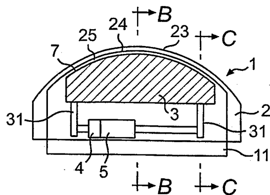
FIG. 5 PRIOR ART
