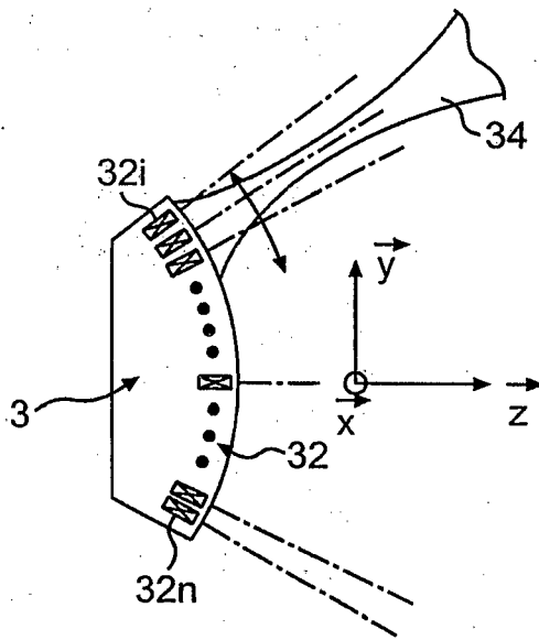
FIG. 3 PRIOR ART
