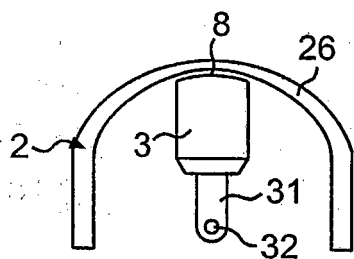
FIG. 6 PRIOR ART
