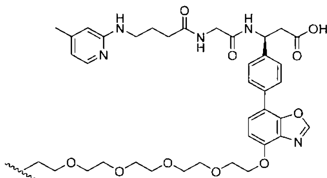
(Structure 12)
