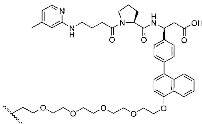
(Structure 11)
