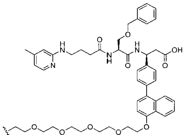
(Structure 25);
