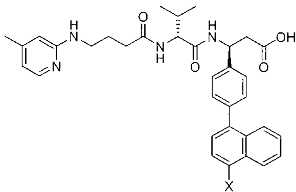
(Structure 37a),
