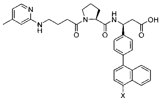
(Structure 11a),
