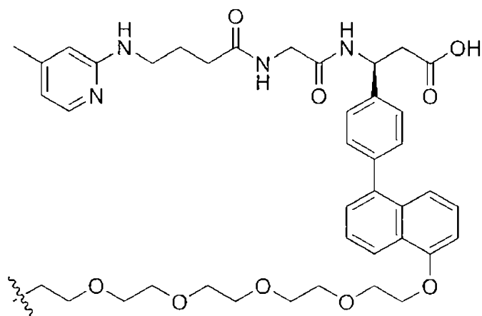
(Structure 10);
