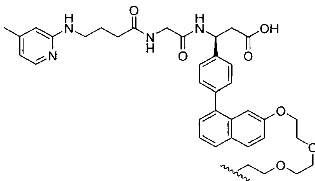
(Structure 8)
