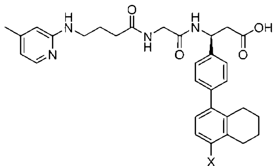
(Structure 13a),
