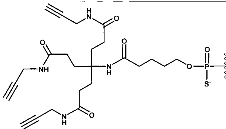
(TriAlk3)s
