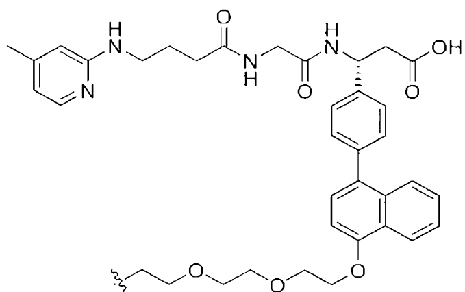
(Structure 7);
