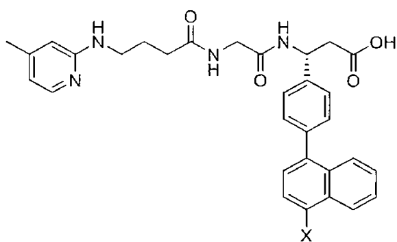
(Structure 7a),
