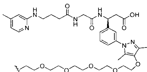
(Structure 27);
