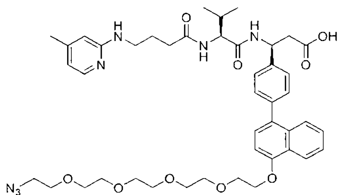
(Structure 23b),
