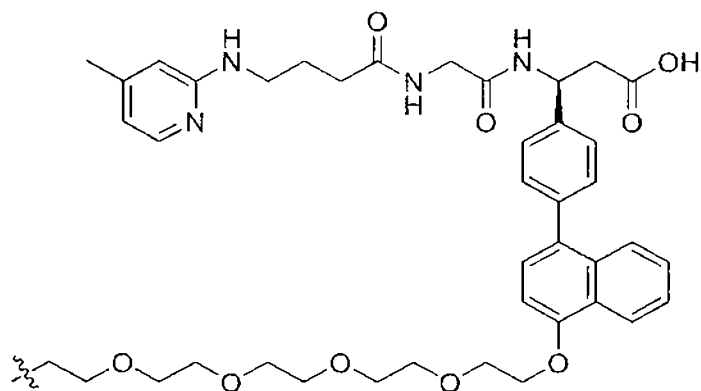
(Structure 6.1);
