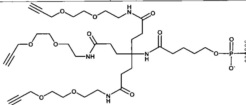
(TriAlk6)
