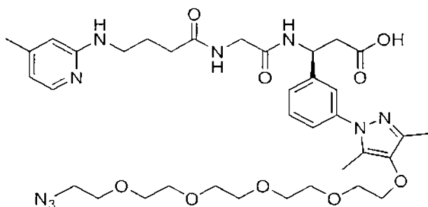
(Structure 27b),
