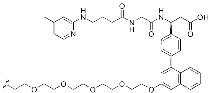
(Structure 29);
