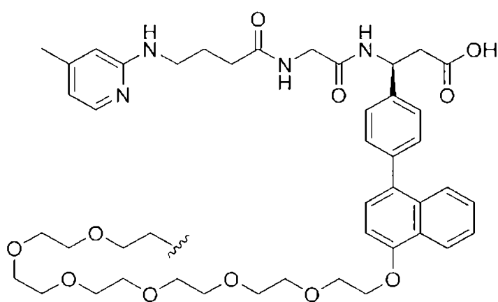
(Structure 6.3);
