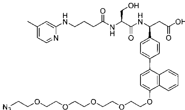
(Structure 31b)
