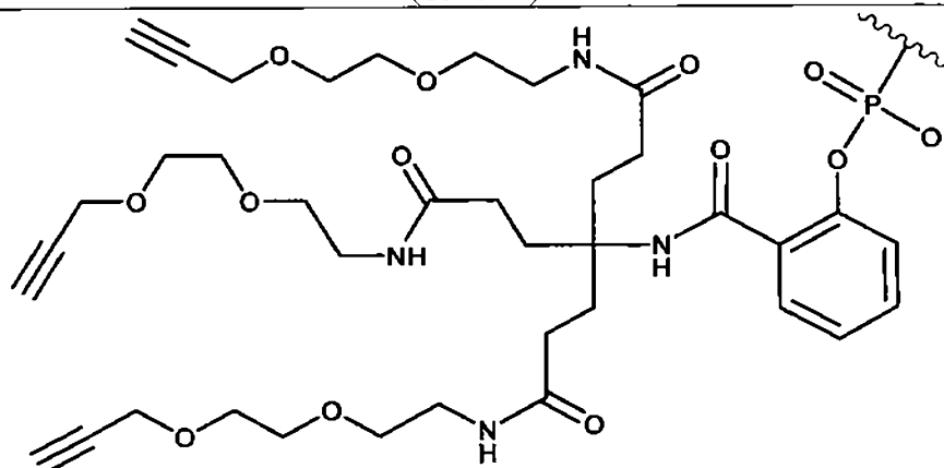
(TriAlk9)
