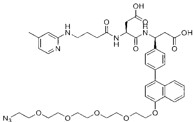
(Structure 32b),
