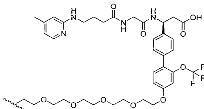
(Structure 14)
