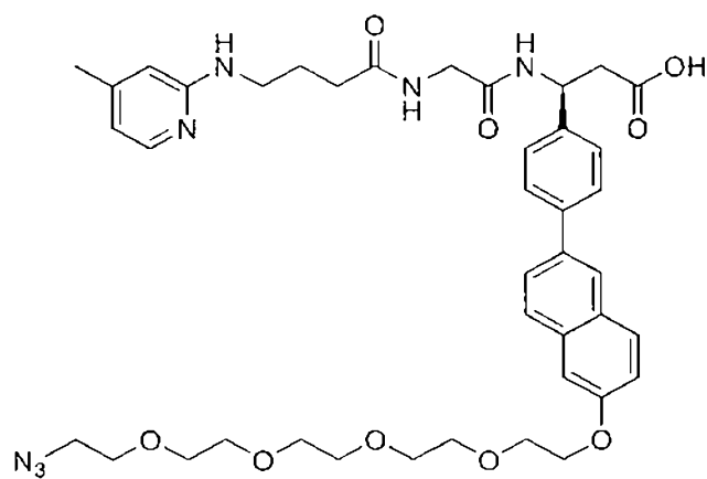
(Structure 18b),
