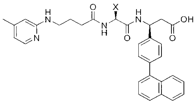
(Structure 2a),
