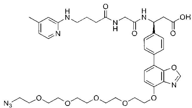
(Structure 12b),
