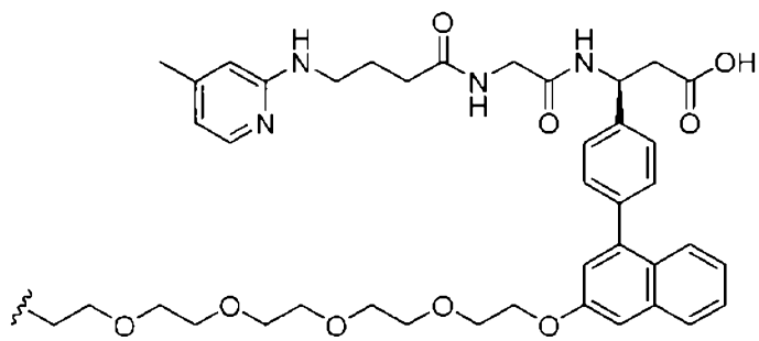
(Structure 29);
