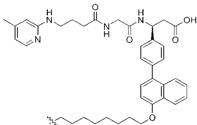
(Structure 6.2);
