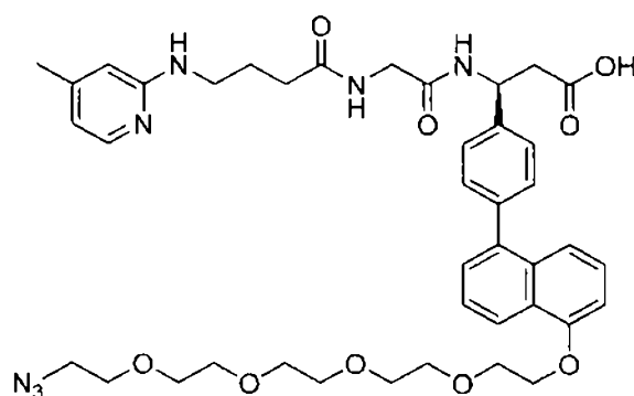
(Structure 10b)
