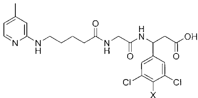
(Structure 5a),
