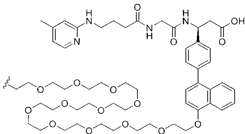
(Structure 6.3);
