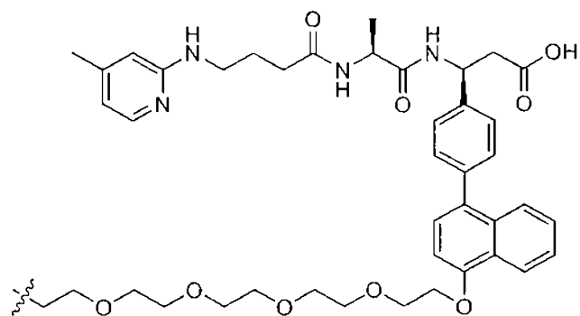
(Structure 22);
