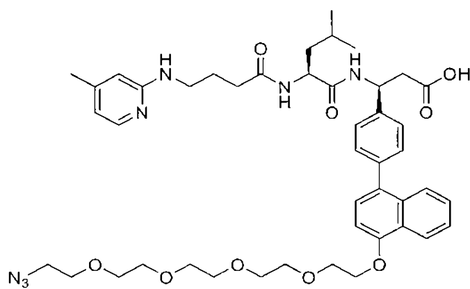
(Structure 34b),
