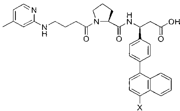
(Structure 11a),
