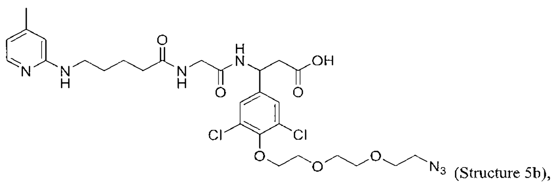
(Structure 2b),
