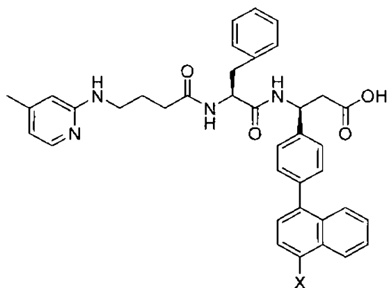
(Structure 24a),
