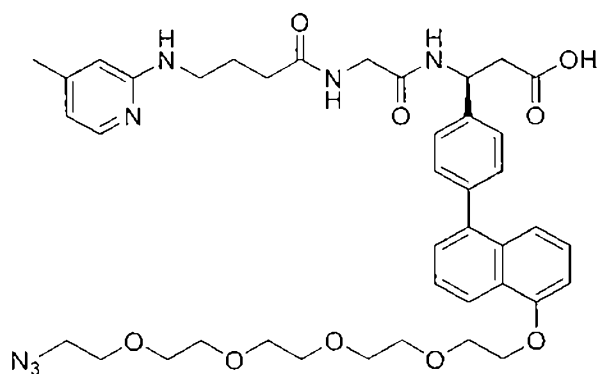
(Structure 10b),
