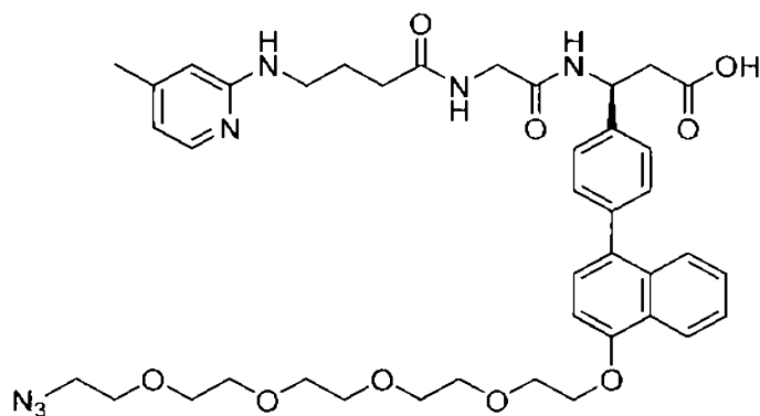
(Structure 6.1b)
