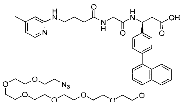
(Structure 6.3b)
