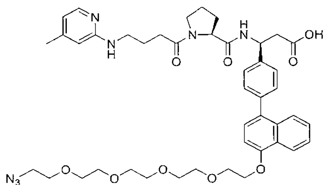
(Structure 11b),
