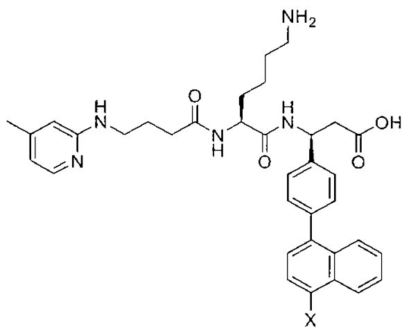
(Structure 33a),
