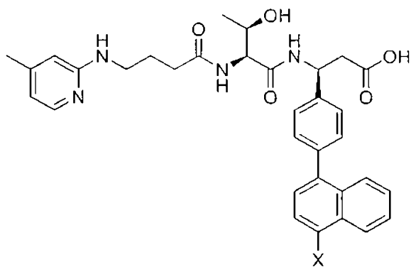
(Structure 35a),
