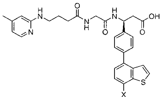
(Structure 17a),
