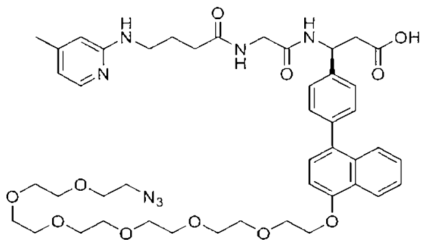
(Structure 6.3b),
