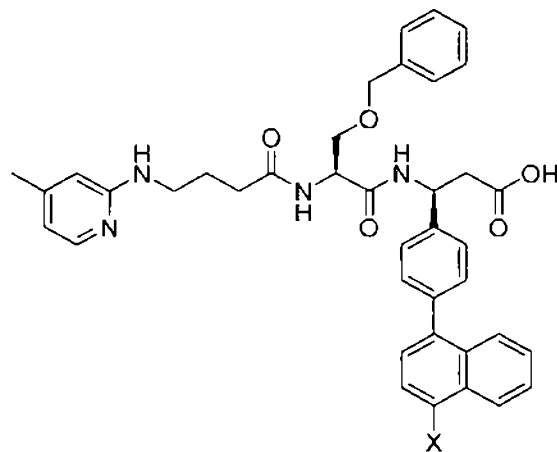
(Structure 25a),
