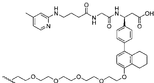
(Structure 13)
