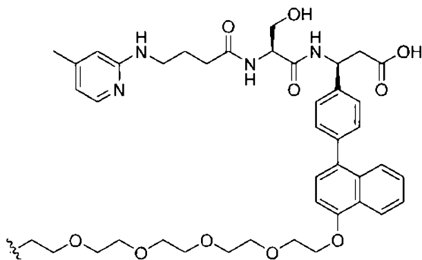
(Structure 31)
