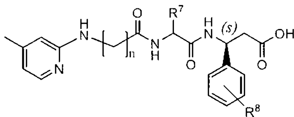
(Formula III),
