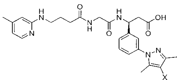
(Structure 27a),
