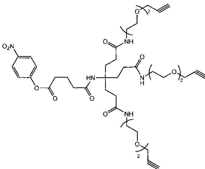
(Scaffold 1)
