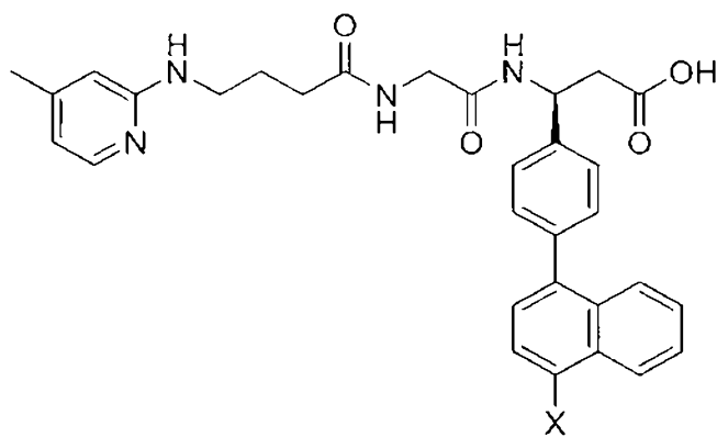
(Structure 6a),
