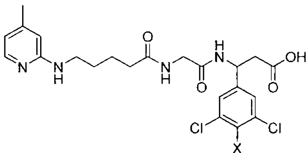
(Structure 5a),
