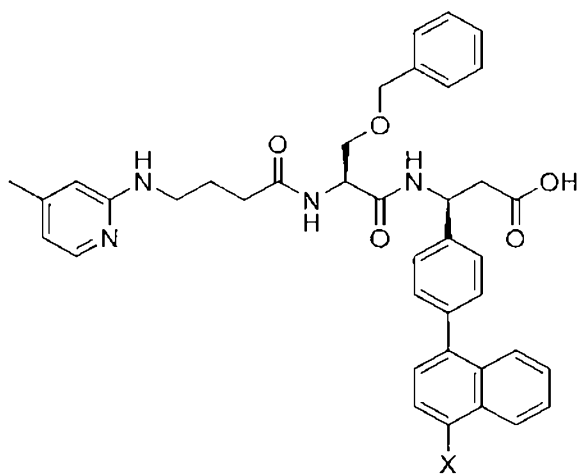
(Structure 25a),
