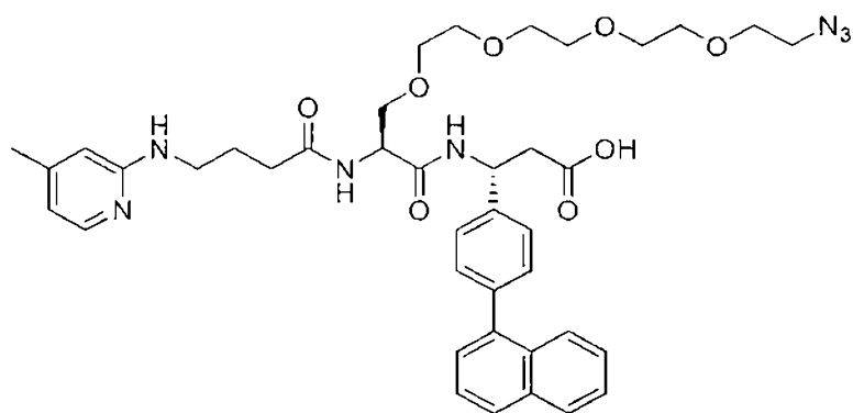
(Structure 9b),
