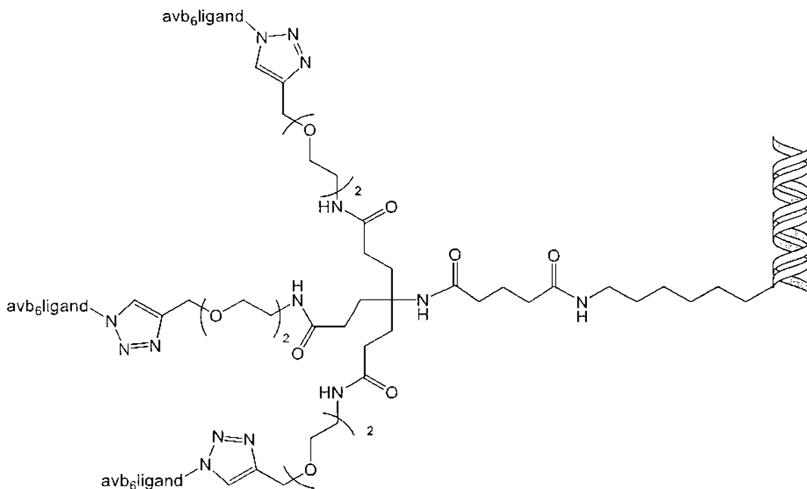
(Structure 300a),
