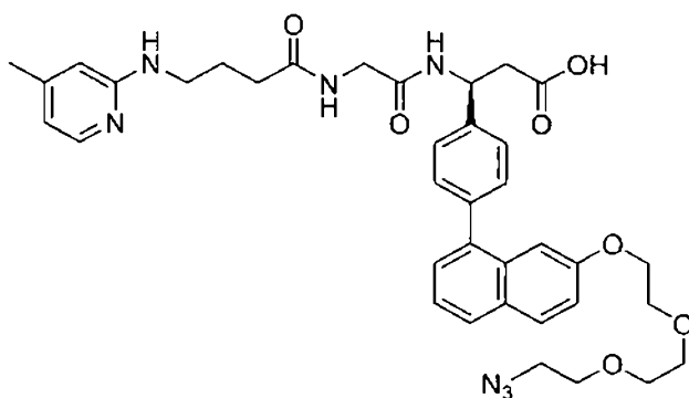
(Structure 8b)
