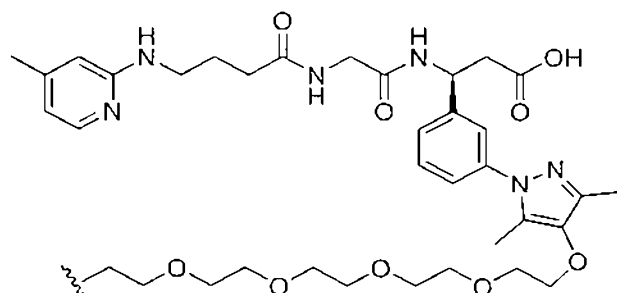
(Structure 27);
