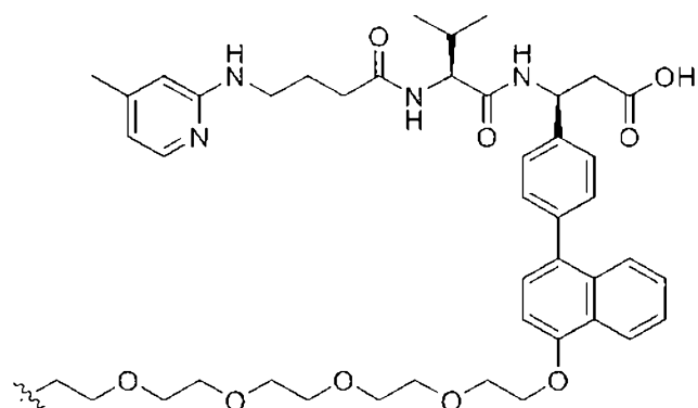
(Structure 23);
