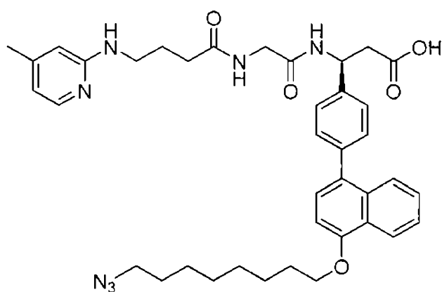
(Structure 6.2b)
