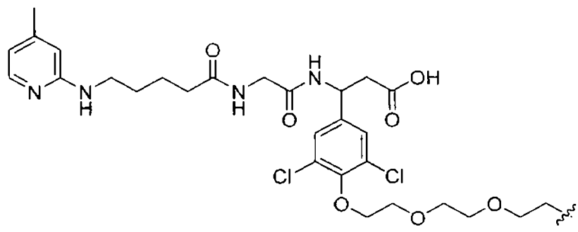
(Structure 5);
