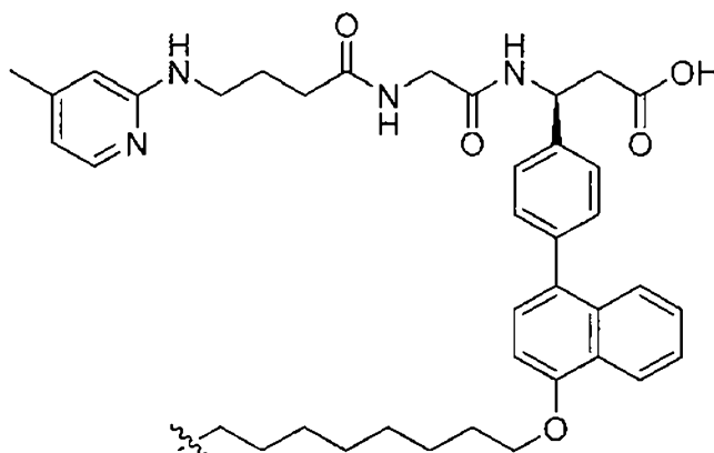
(Structure 6.2)
