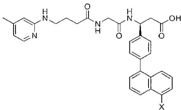
(Structure 10a),
