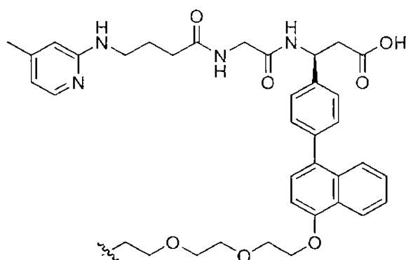
(Structure 6);
