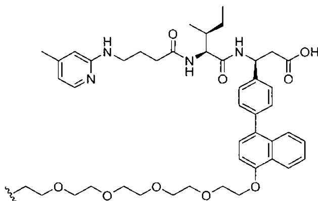
(Structure 36); and
