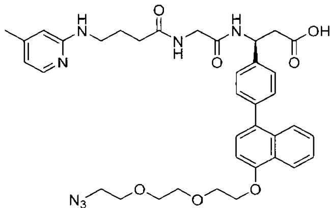
(Structure 6b)
