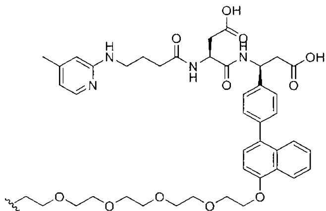
(Structure 32);
