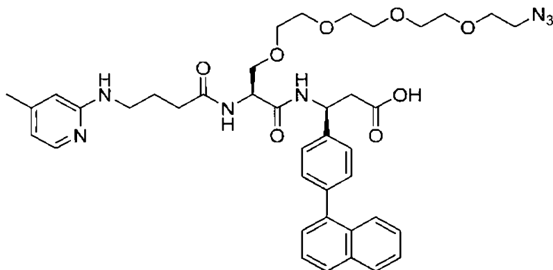
(Structure 2b).
