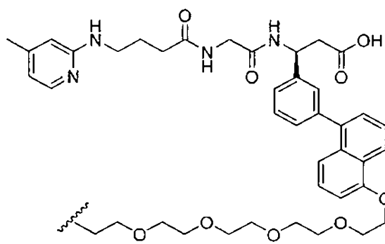
(Structure 15)
