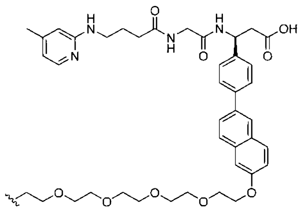
(Structure 18);
