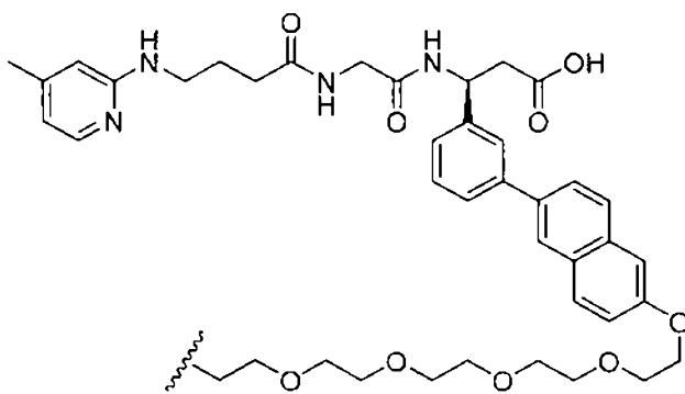
(Structure 19)
