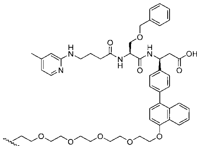
(Structure 25)
