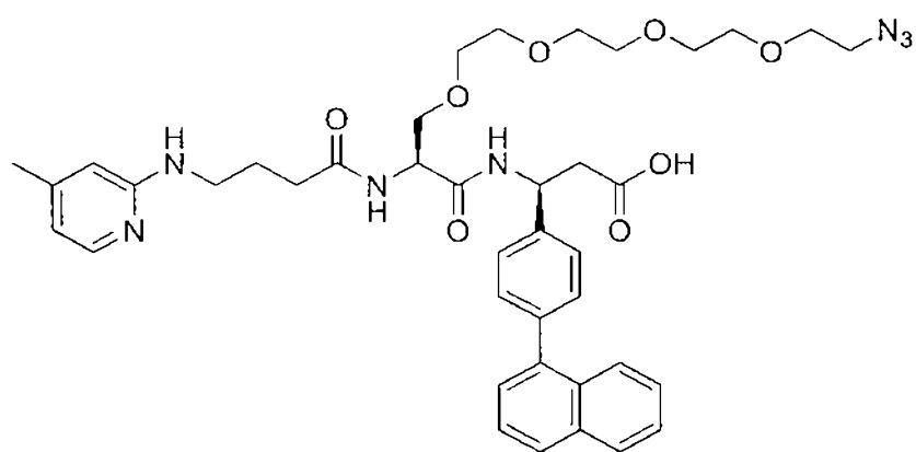
(Structure 1b),
