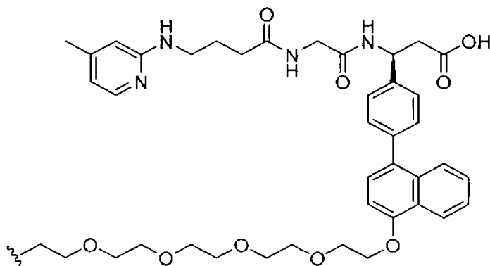
(Structure 6.1)
