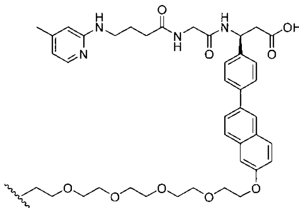
(Structure 18)
