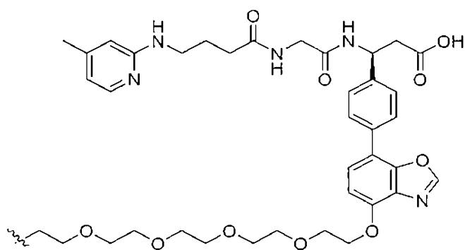
(Structure 12);
