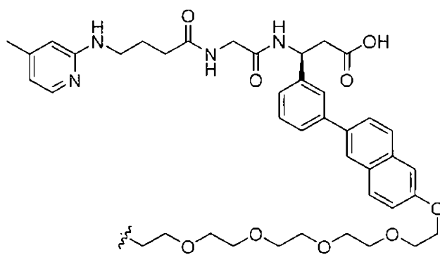
(Structure 19);
