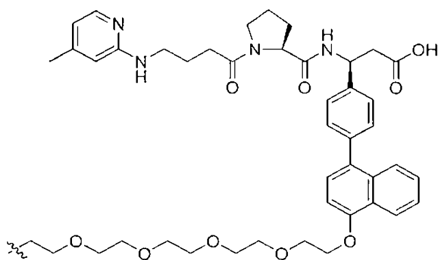
(Structure 11);
