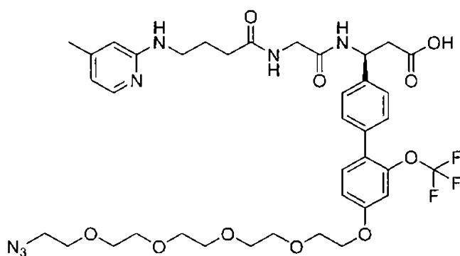
(Structure 14b)
