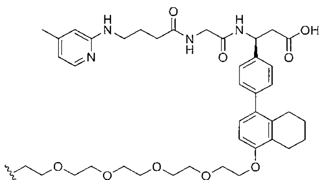
(Structure 13);
