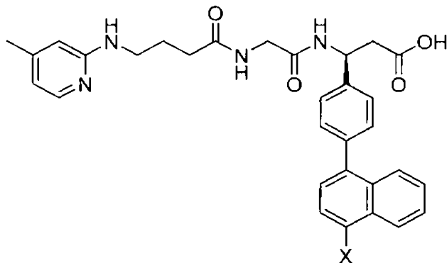
(Structure 6a),
