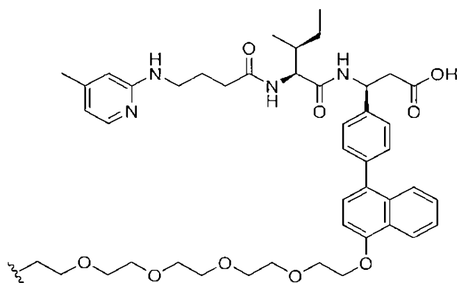
(Structure 36); and
