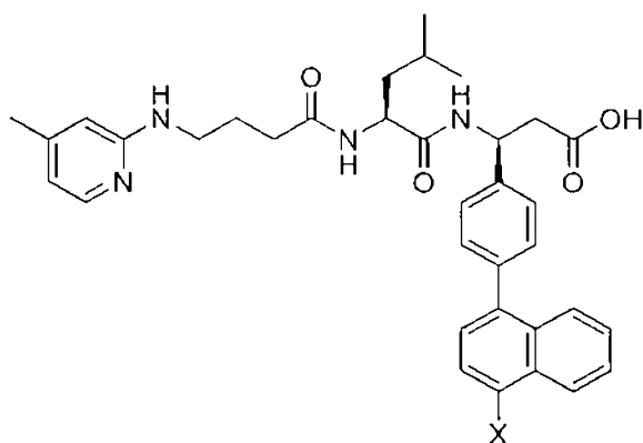
(Structure 34a),
