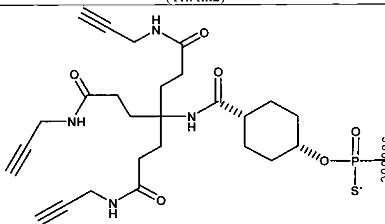
(TriAlk2)s
