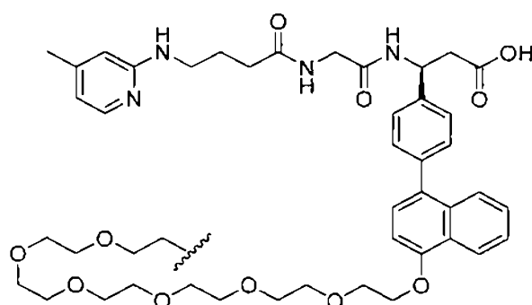
(Structure 6.3)
