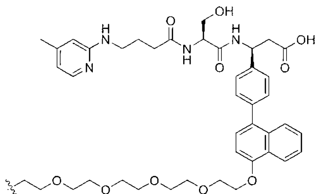
(Structure 31);
