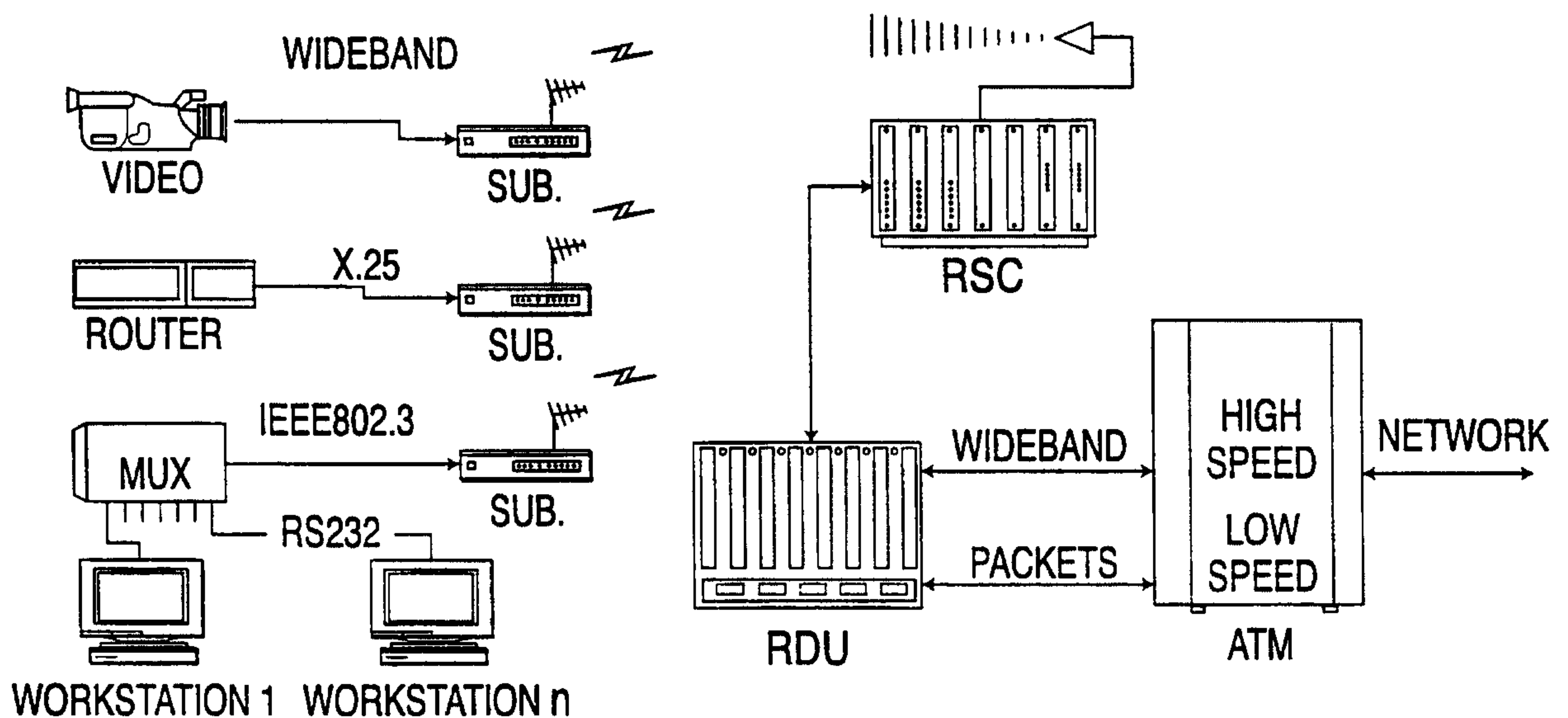
WIDEBAND AND PACKET NETWORK INTERFACE
