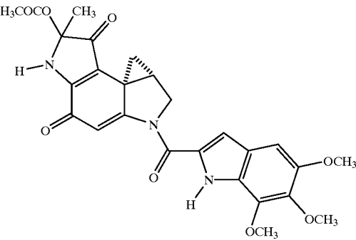
Duocarmycin A
