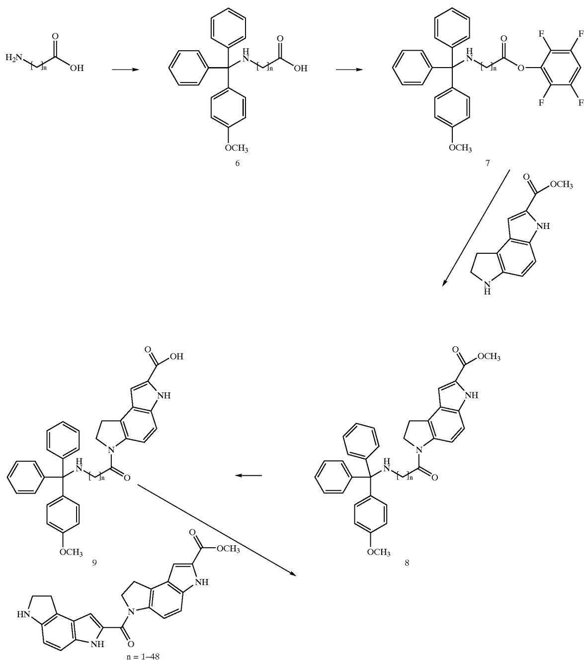
Reaction Scheme 4
