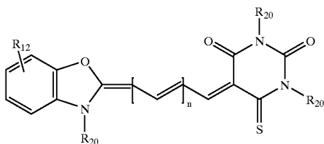
Formula 10
