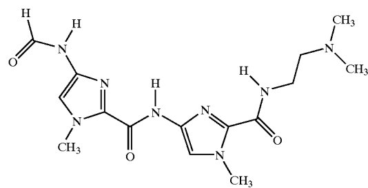
Lexitropsin
