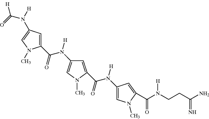
Distamycin
