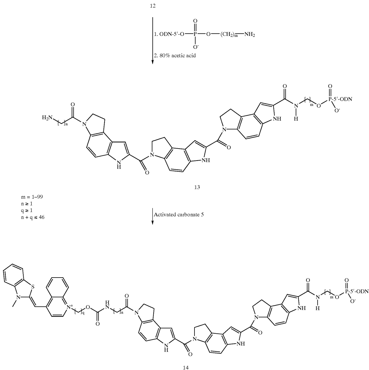
Reaction Scheme 5
