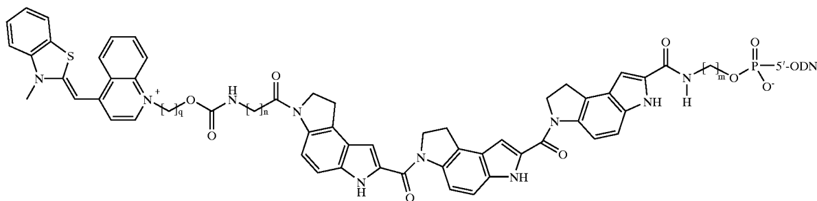
Formula 12
