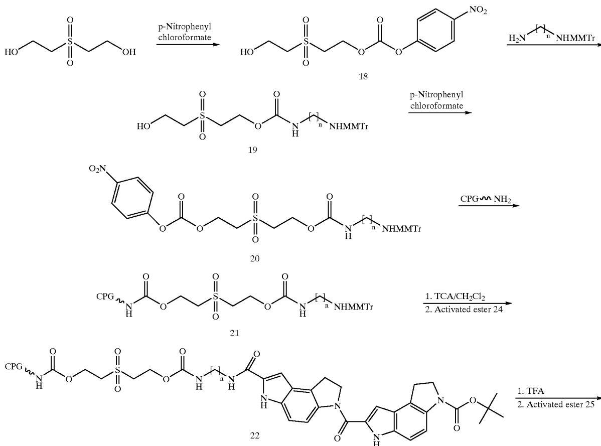
Reaction Scheme 7
