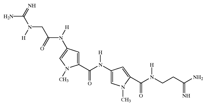
Netropsin
