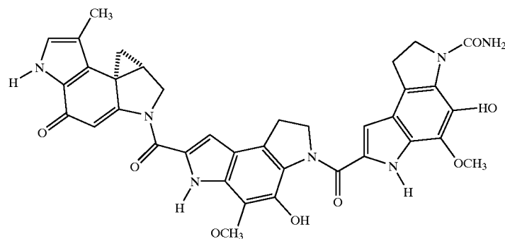
CC-1065
