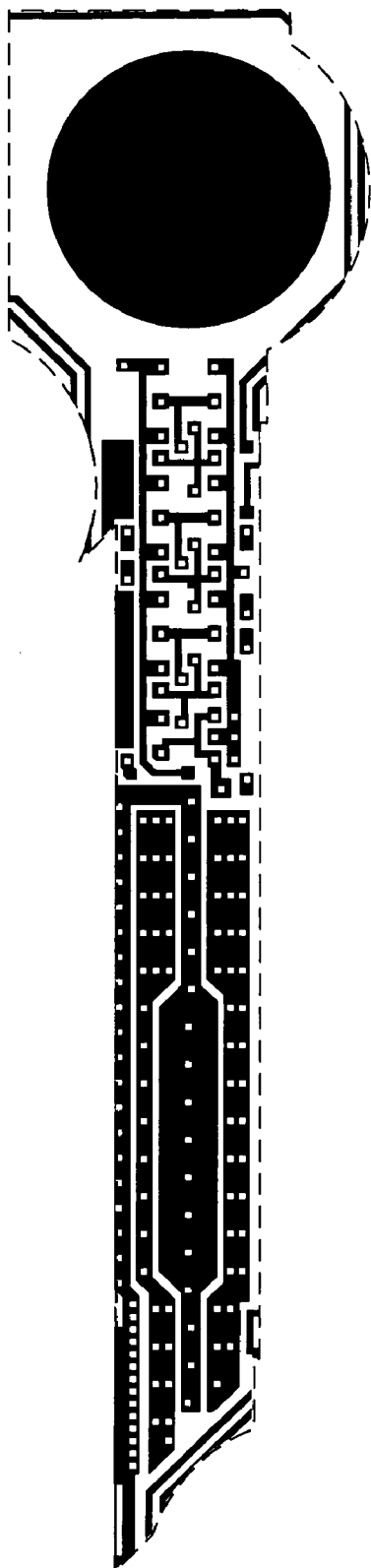
Metal 1 mask
