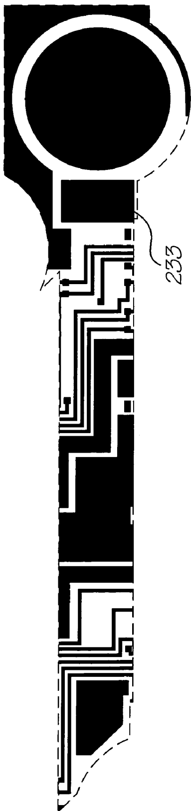
Metal 2 mask
