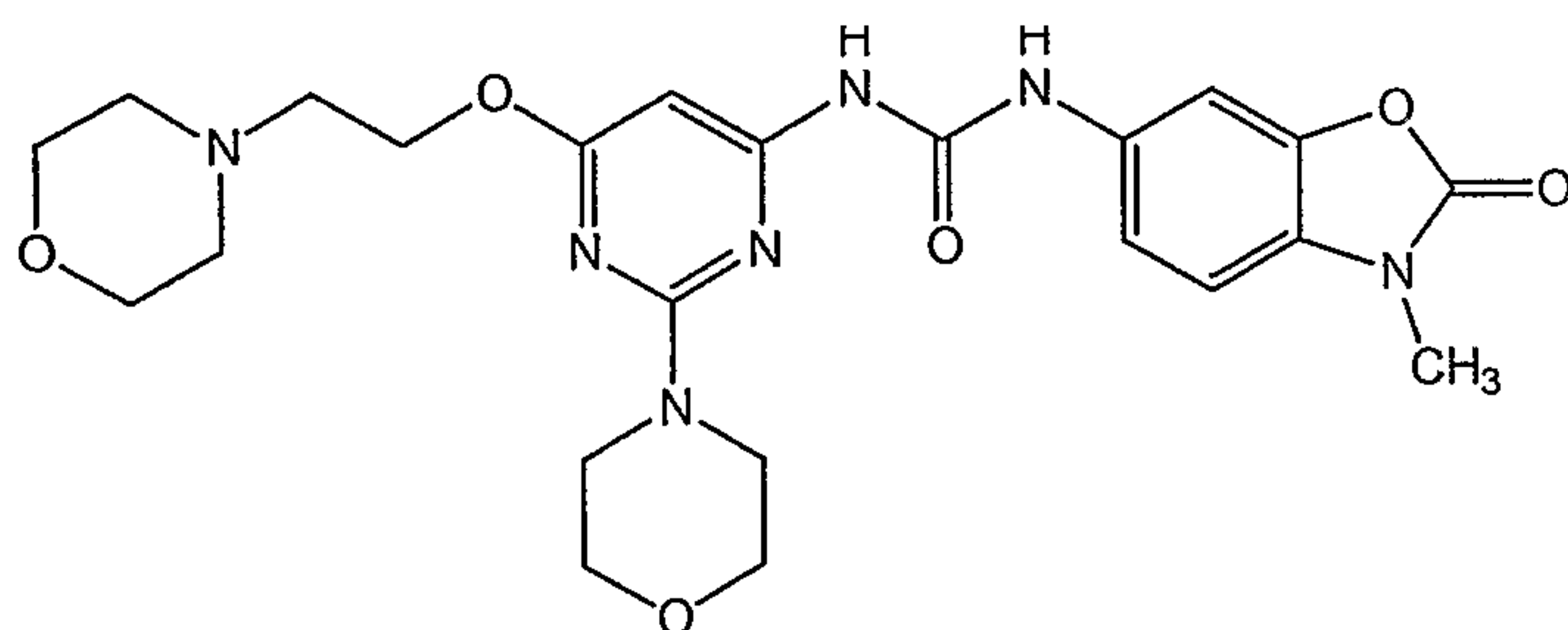
1-(3-Methyl-2-oxo-2,3-dihydro-benzooxazol-6-yl)-3-[2-morpholin-4-yl-6-(2-morpholin-4-yl-ethoxy)-pyrimidin-4-yl]-urea
