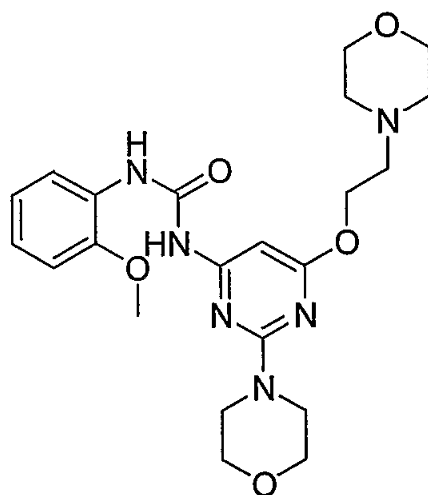
1-(2-Methoxy-phenyl)-3-[2-morpholin-4-yl-6-(2-morpholin-4-yl-ethoxy)-pyrimidin-4-yl]-urea
