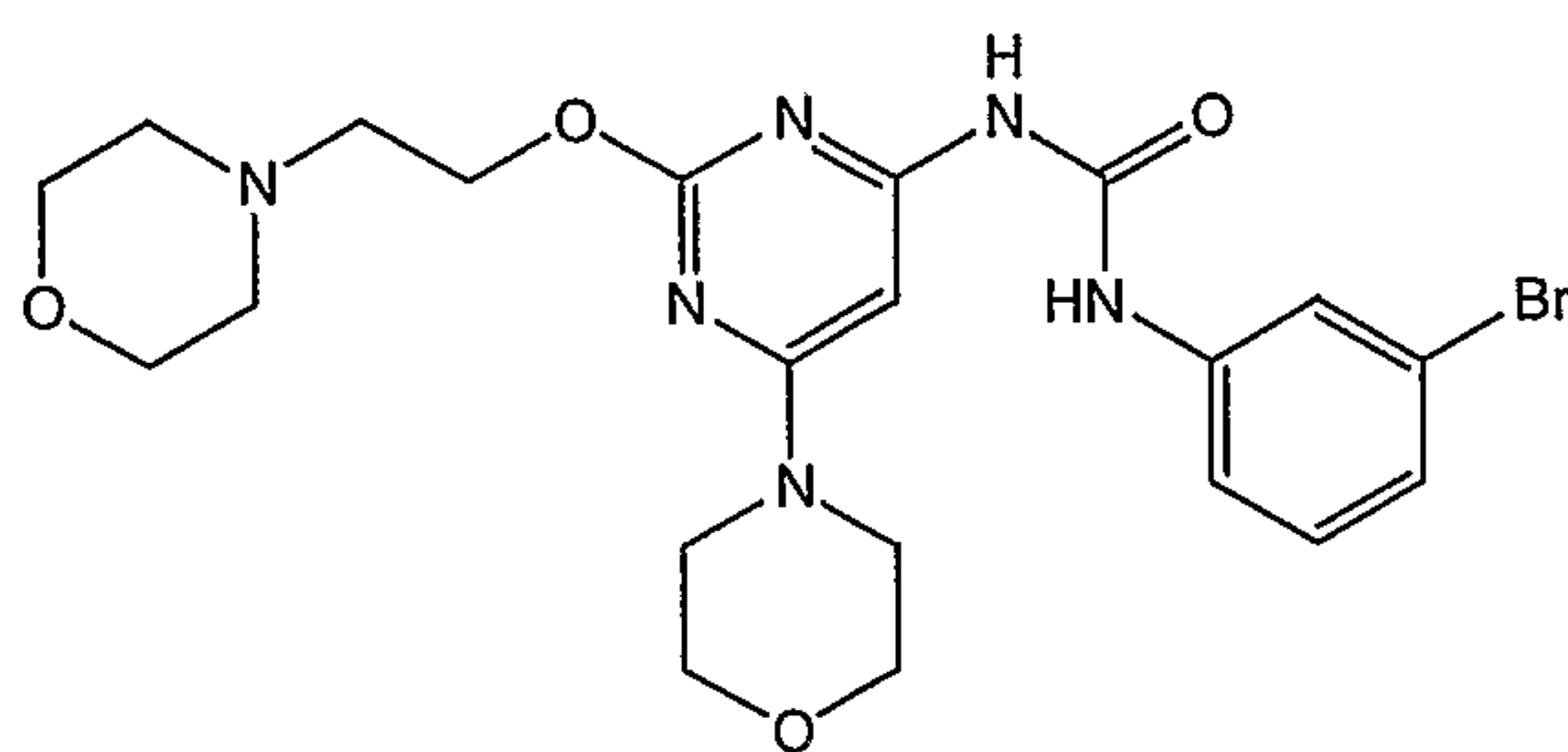
1-(3-Bromo-phenyl)-3-[6-morpholin-4-yl-2-(2-morpholin-4-yl-ethoxy)-pyrimidin-4-yl]-urea
