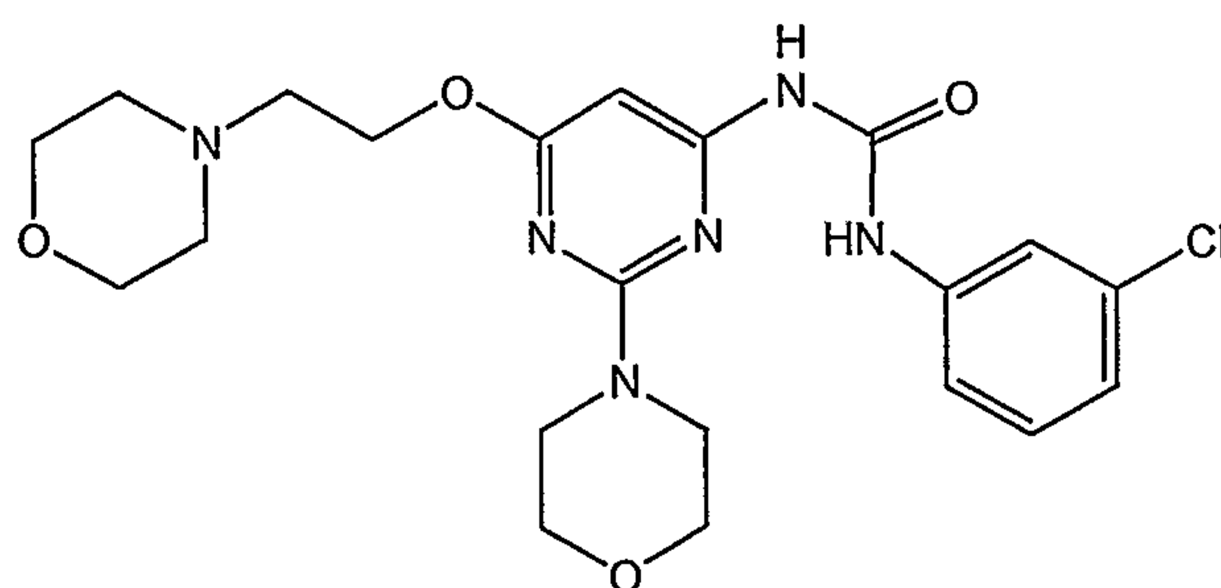
1-(3-Chloro-phenyl)-3-[2-morpholin-4-yl-6-(2-morpholin-4-yl-ethoxy)-pyrimidin-4-yl]-urea
