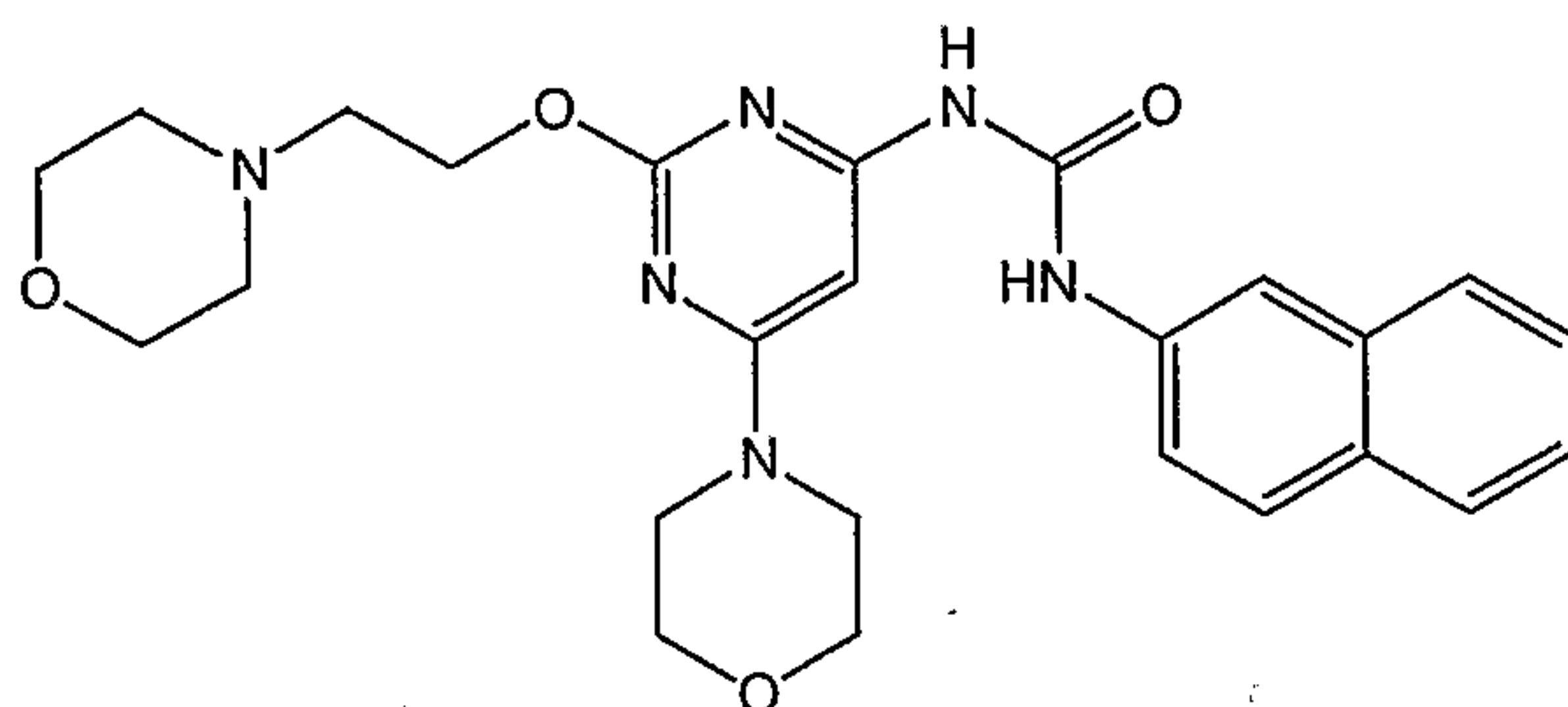
1-[6-Morpholin-4-yl-2-(2-morpholin-4-yl-ethoxy)-pyrimidin-4-yl]-3-naphthalen-2-yl-urea
