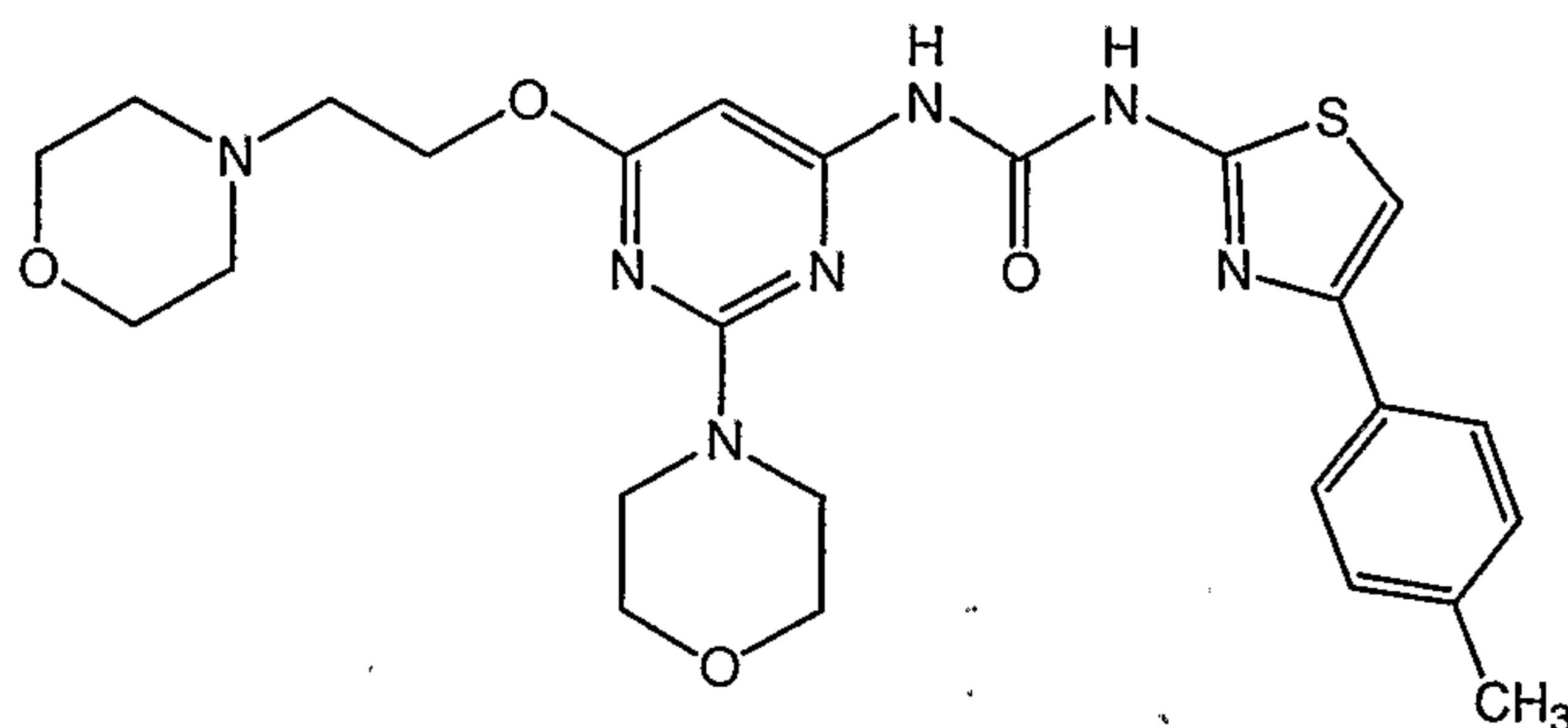
1-[2-Morpholin-4-yl-6-(2-morpholin-4-yl-ethoxy)-pyrimidin-4-yl]-3-(4-p-tolyl-thiazol-2-yl)-urea
