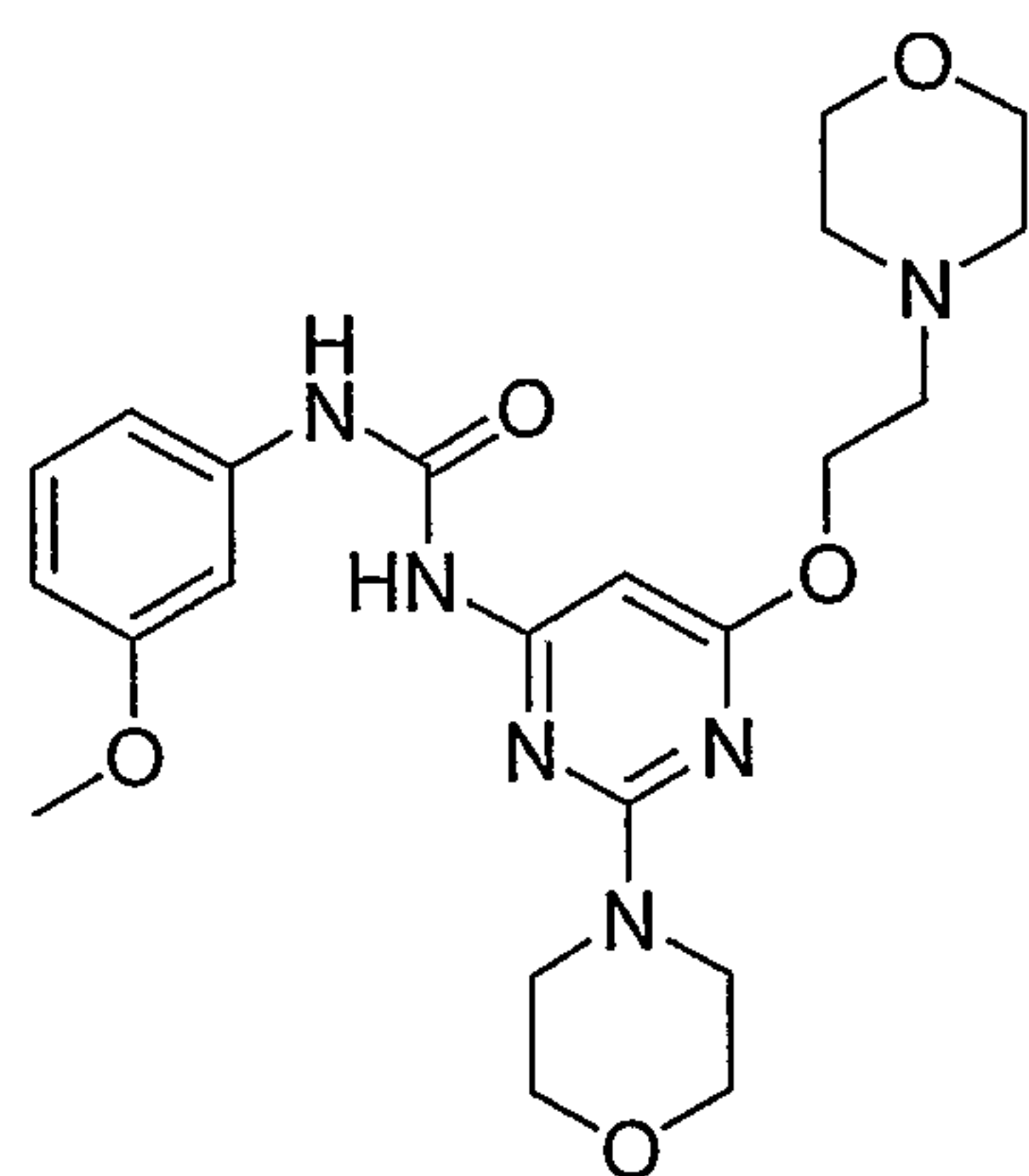
1-(3-Methoxy-phenyl)-3-[2-morpholin-4-yl-6-(2-morpholin-4-yl-ethoxy)-pyrimidin-4-yl]-urea
