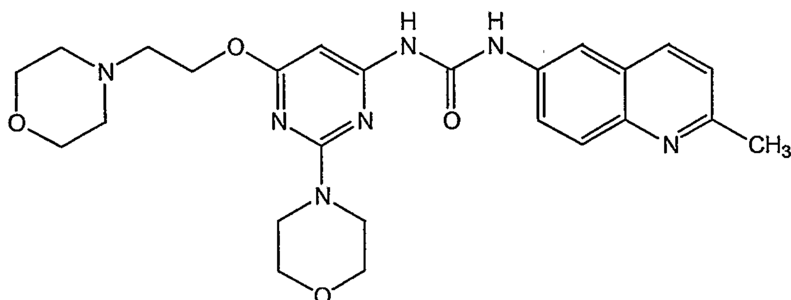
1-(2-Methyl-quinolin-6-yl)-3-[2-morpholin-4-yl-6-(2-morpholin-4-yl-ethoxy)-pyrimidin-4-yl]-urea
