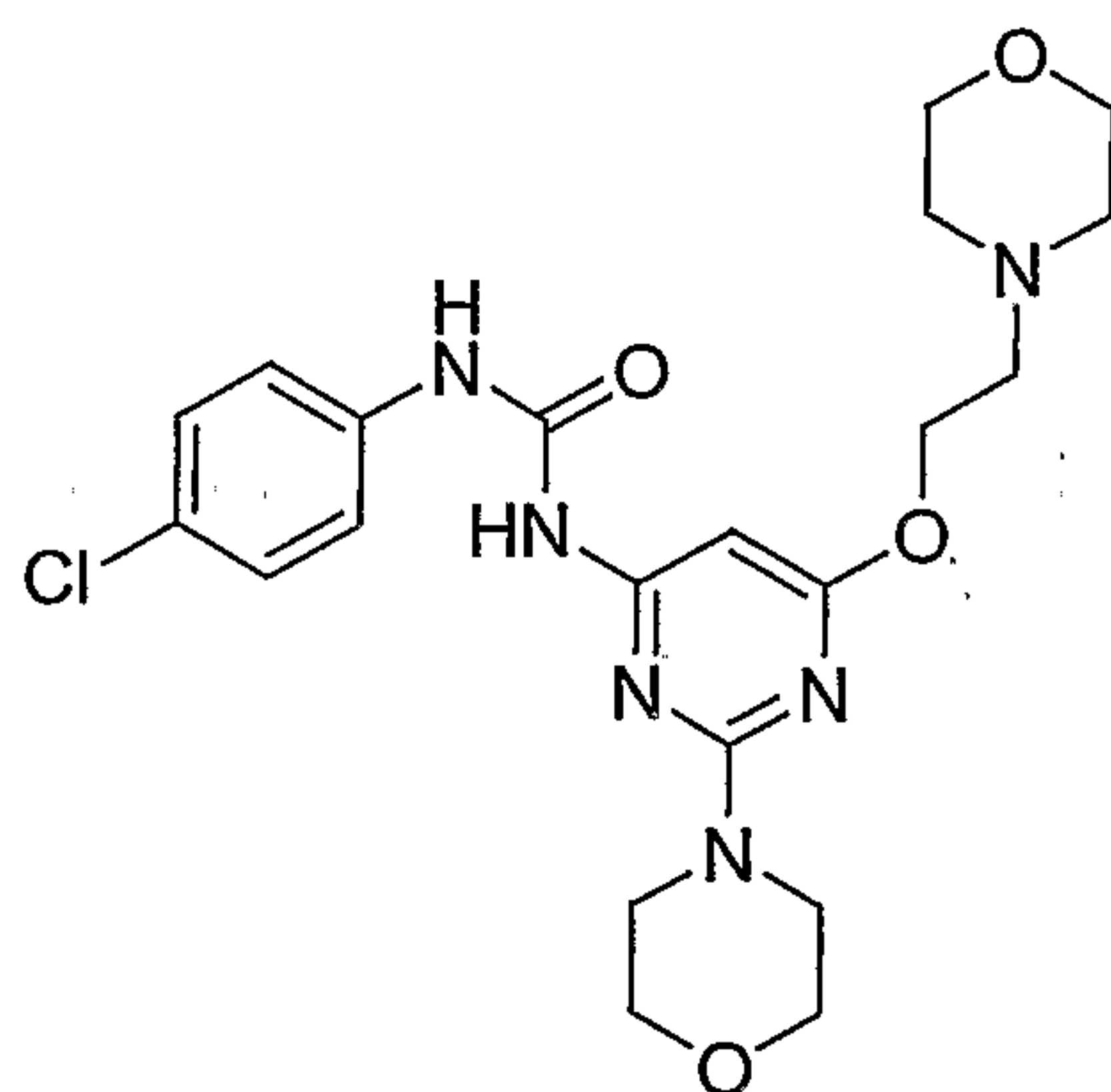
1-(4-Chloro-phenyl)-3-[2-morpholin-4-yl-6-(2-morpholin-4-yl-ethoxy)-pyrimidin-4-yl]-urea
