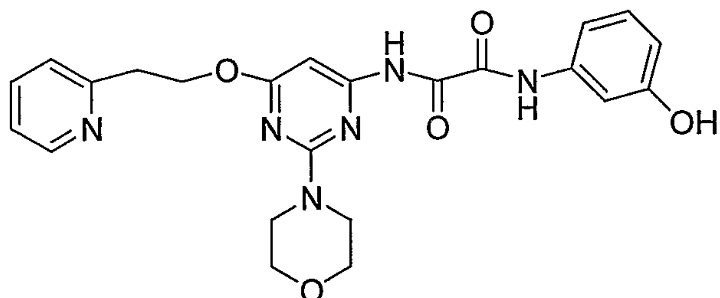
N-(3-Hydroxy-phenyl)-N'-[2-morpholin-4-yl-6-(2-pyridin-2-yl-ethoxy)-pyrimidin-4-yl]-oxalamide
