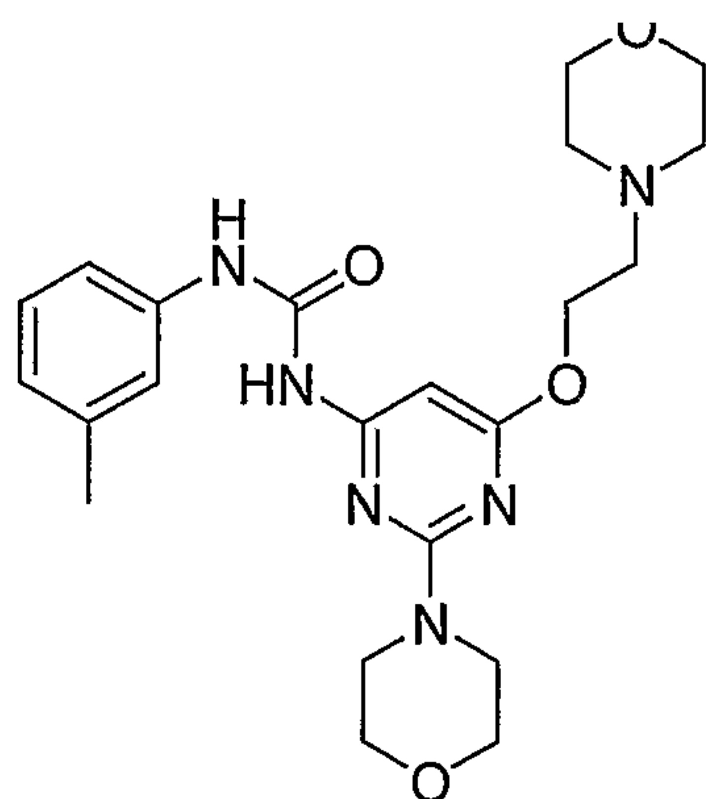
1-[2-Morpholin-4-yl-6-(2-morpholin-4-yl-ethoxy)-pyrimidin-4-yl]-3-m-tolyl-urea
