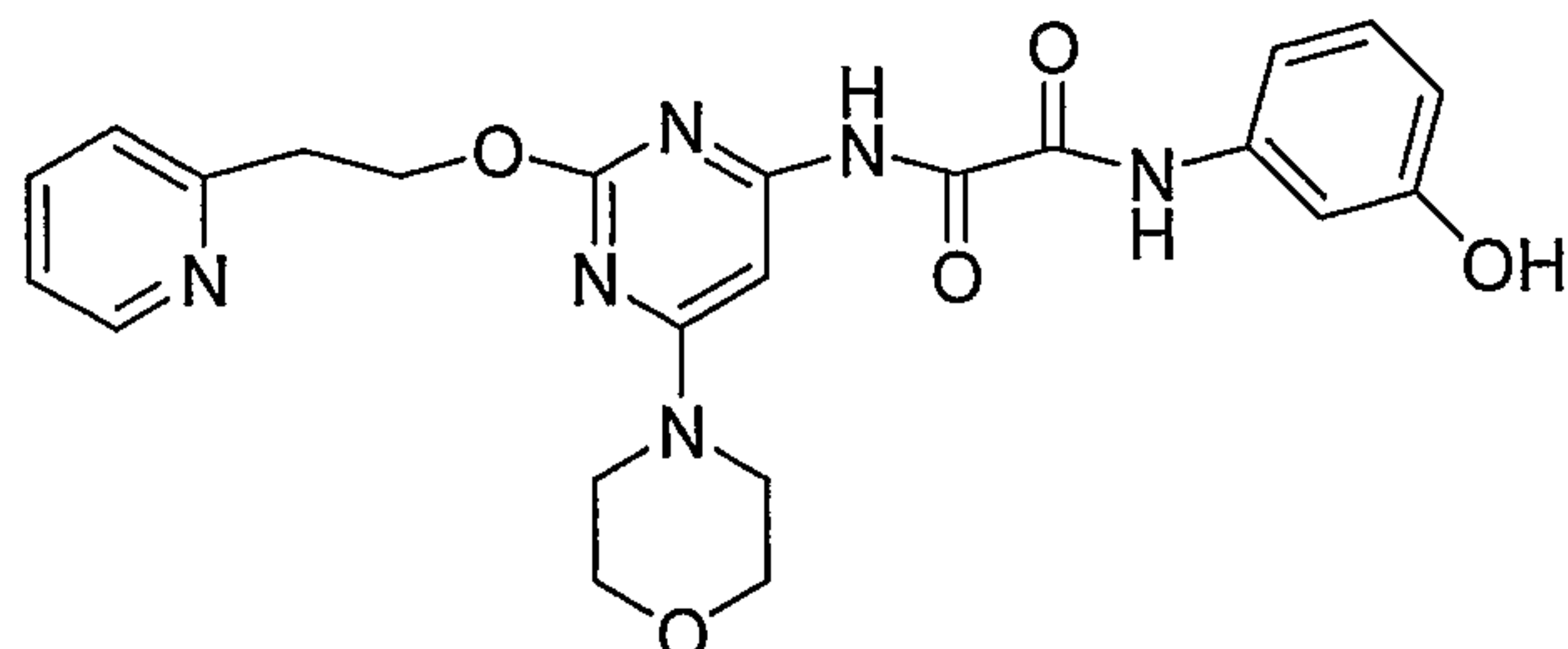
N-(3-Hydroxy-phenyl)-N'-[6-morpholin-4-yl-2-(2-pyridin-2-yl-ethoxy)-pyrimidin-4-yl]-oxalamide
