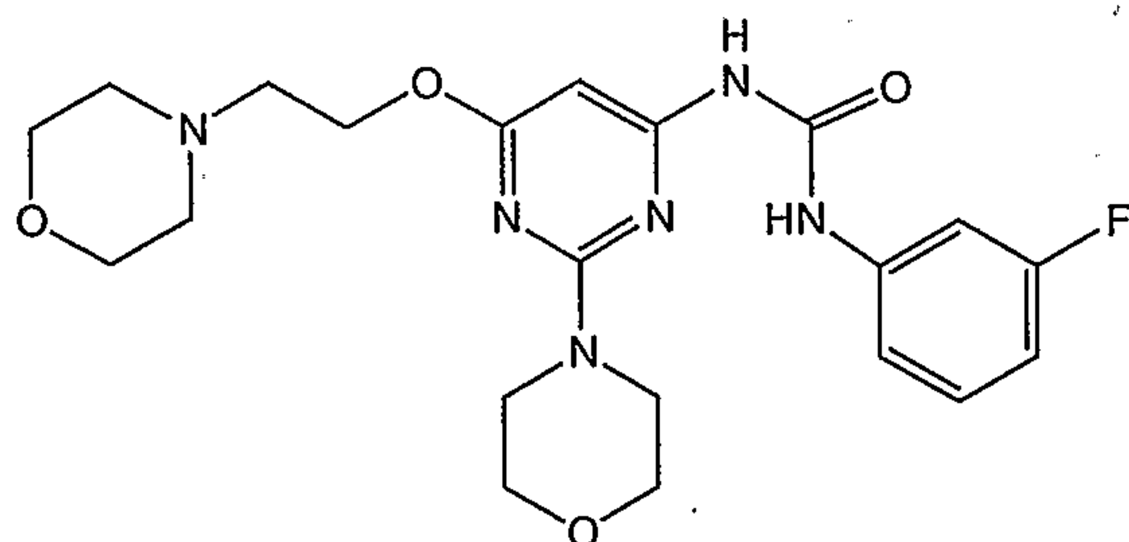
1-(3-Fluoro-phenyl)-3-[2-morpholin-4-yl-6-(2-morpholin-4-yl-ethoxy)-pyrimidin-4-yl]-urea
