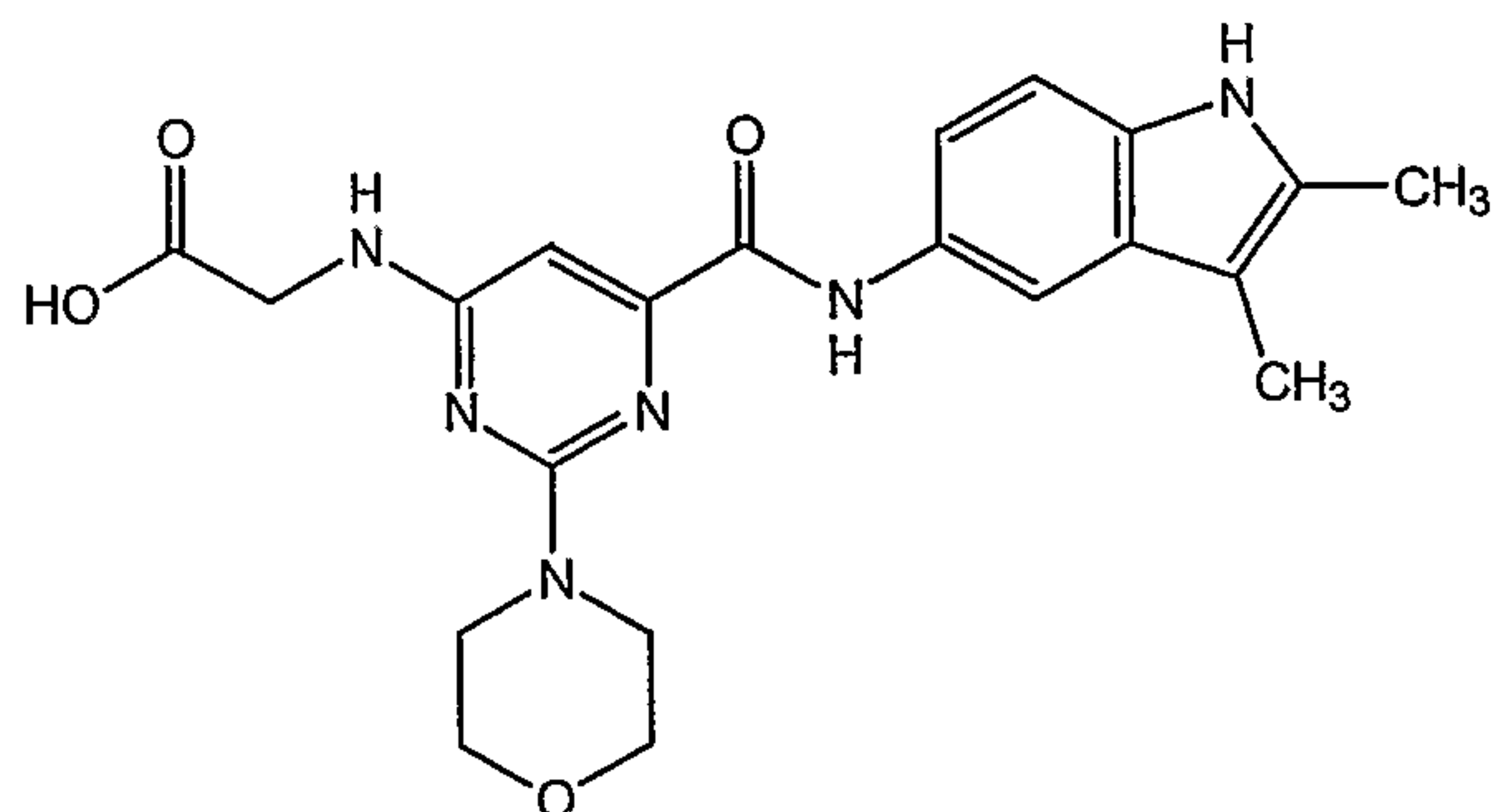
[6-(2,3-Dimethyl-1H-indol-5-ylcarbamoyl)-2-morpholin-4-yl-pyrimidin-4-ylamino]-acetic acid
