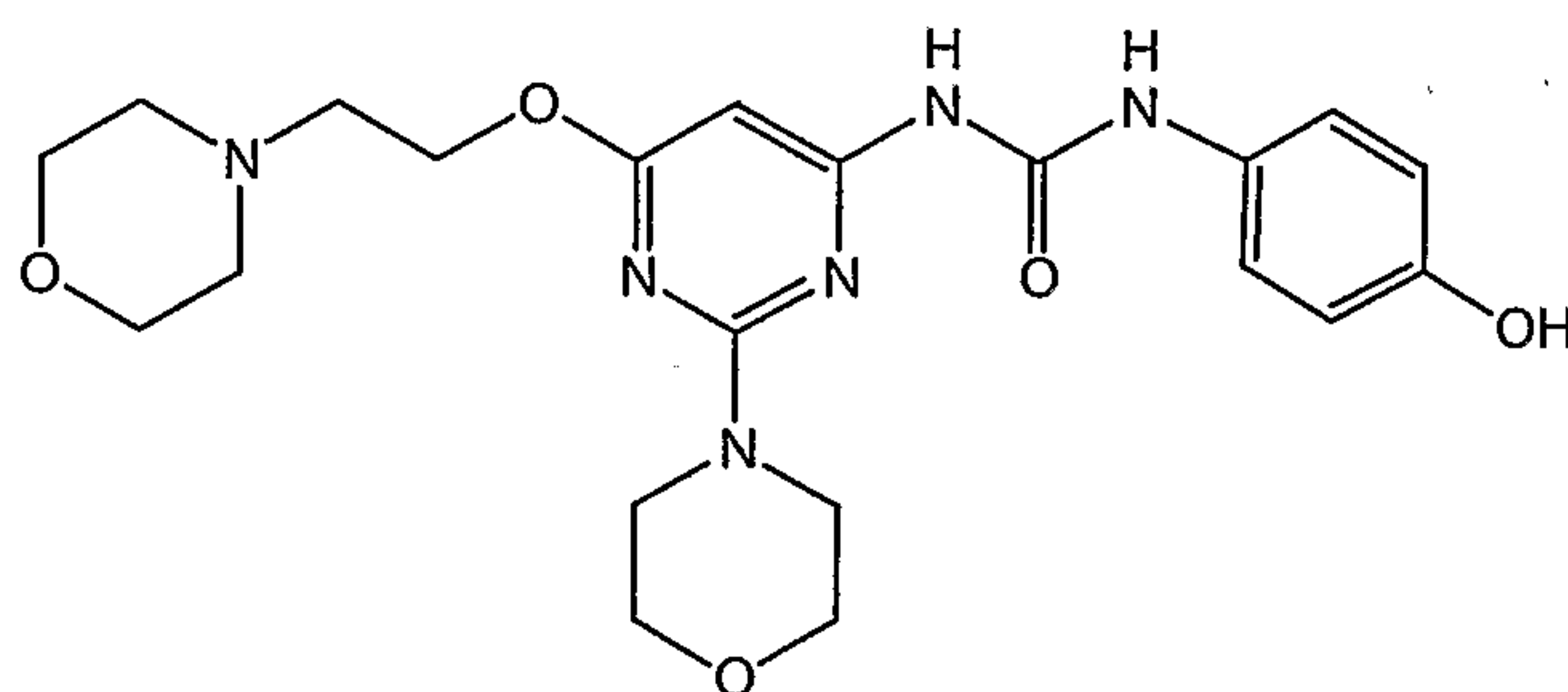
1-(4-Hydroxy-phenyl)-3-[2-morpholin-4-yl-6-(2-morpholin-4-yl-ethoxy)-pyrimidin-4-yl]-urea
