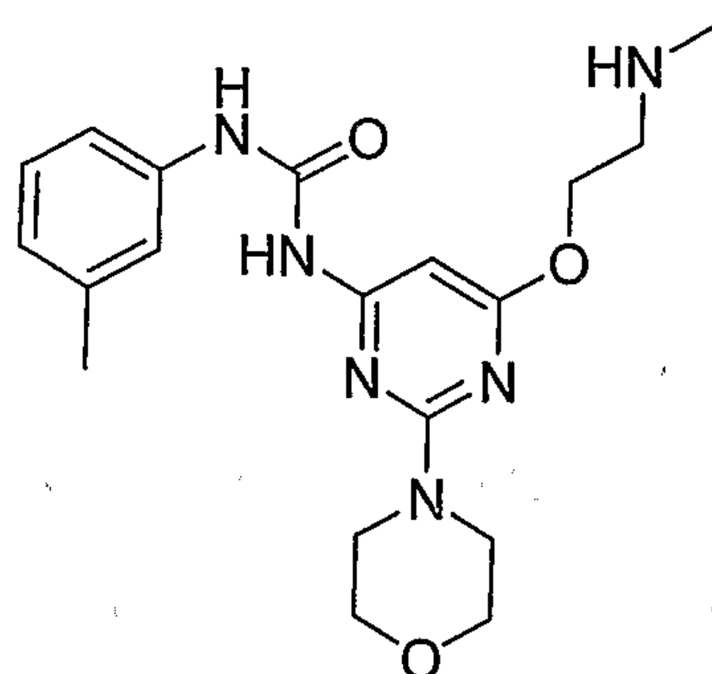
1-[6-(2-Methylamino-ethoxy)-2-morpholin-4-yl-pyrimidin-4-yl]-3-m-tolyl-urea
