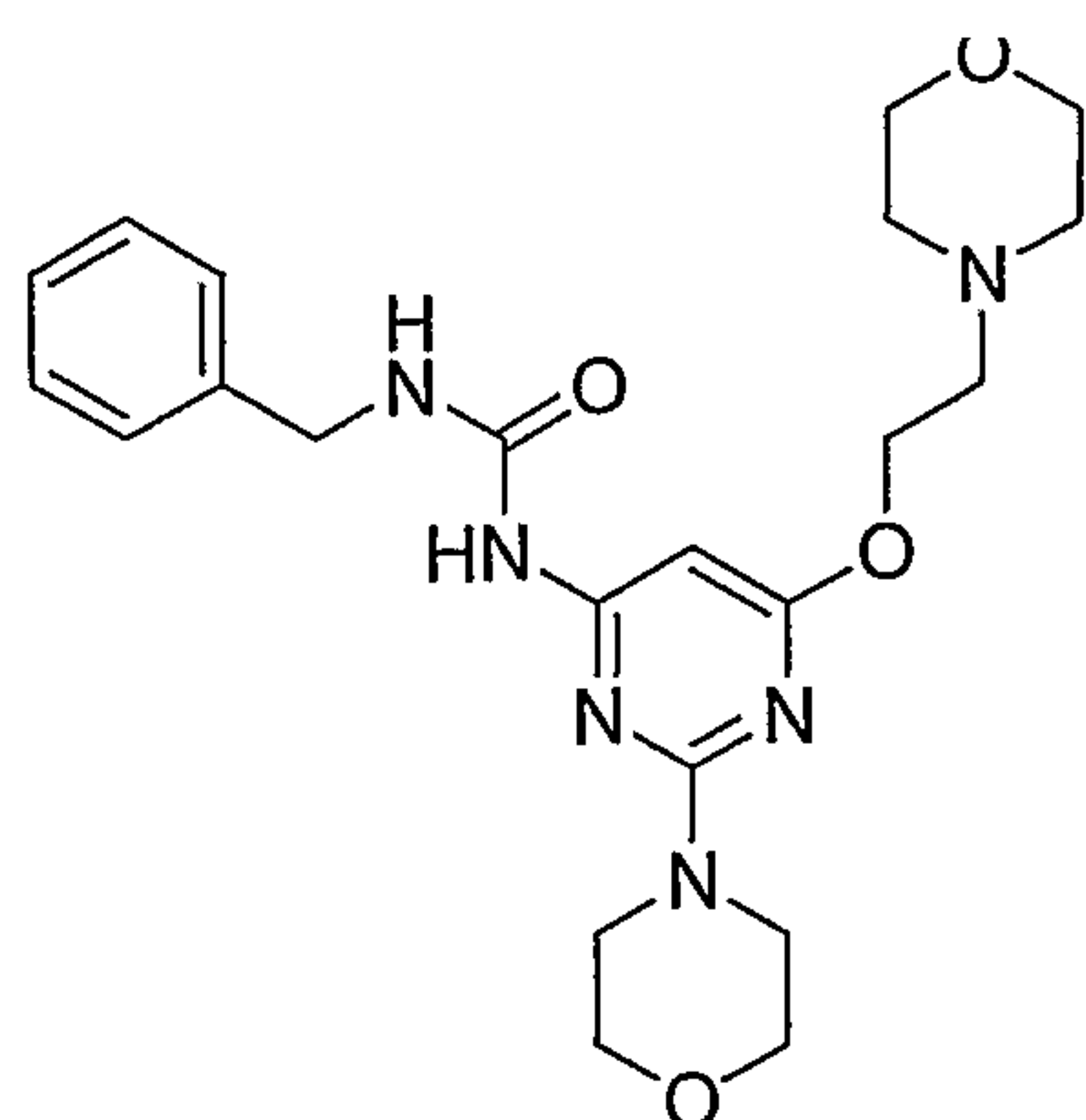
1-Benzyl-3-[2-morpholin-4-yl-6-(2-morpholin-4-yl-ethoxy)-pyrimidin-4-yl]-urea
