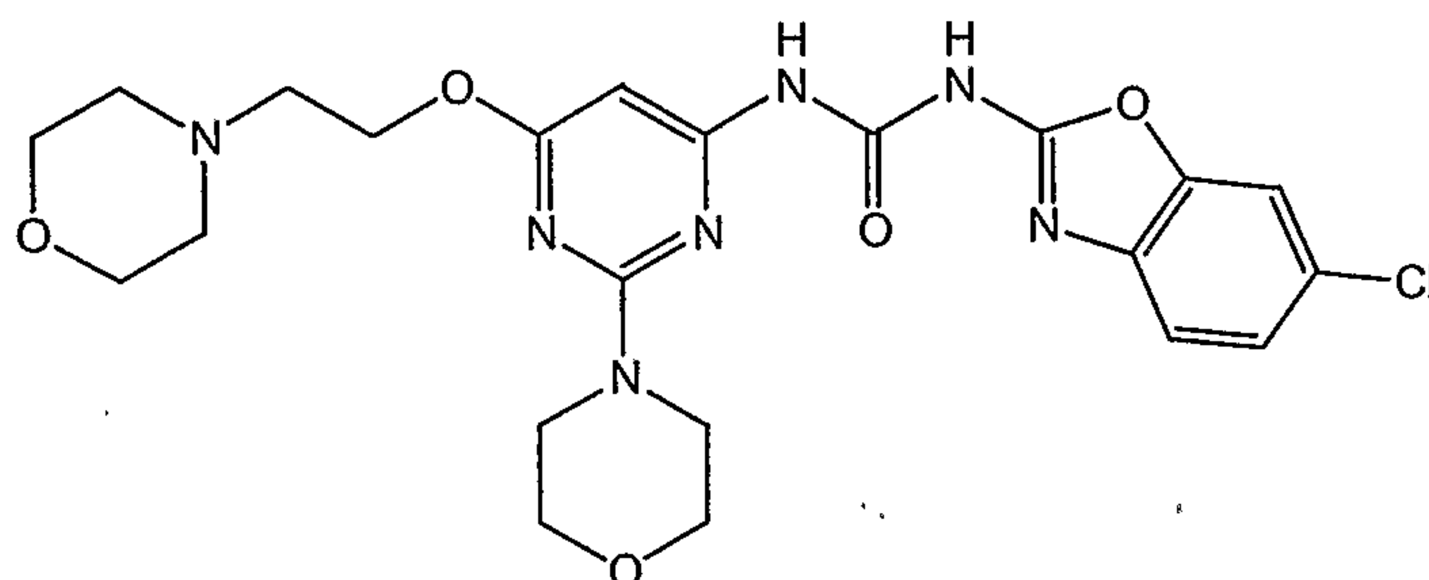
1-(6-Chloro-benzooxazol-2-yl)-3-[2-morpholin-4-yl-6-(2-morpholin-4-yl-ethoxy)-pyrimidin-4-yl]-urea
