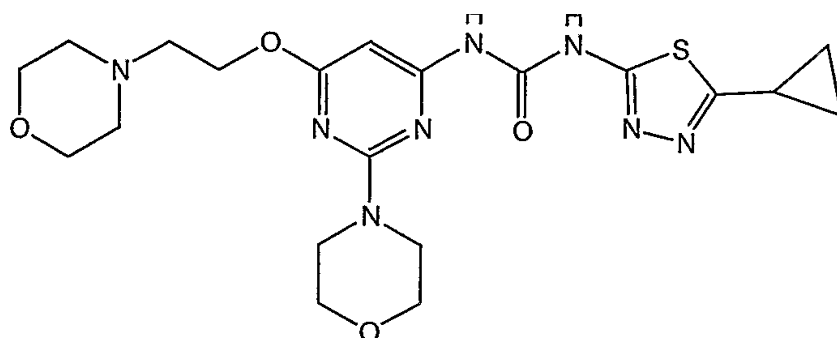
1-(5-Cyclopropyl-[1,3,4]thiadiazol-2-yl)-3-[2-morpholin-4-yl-6-(2-morpholin-4-yl-ethoxy)-pyrimidin-4-yl]-urea
