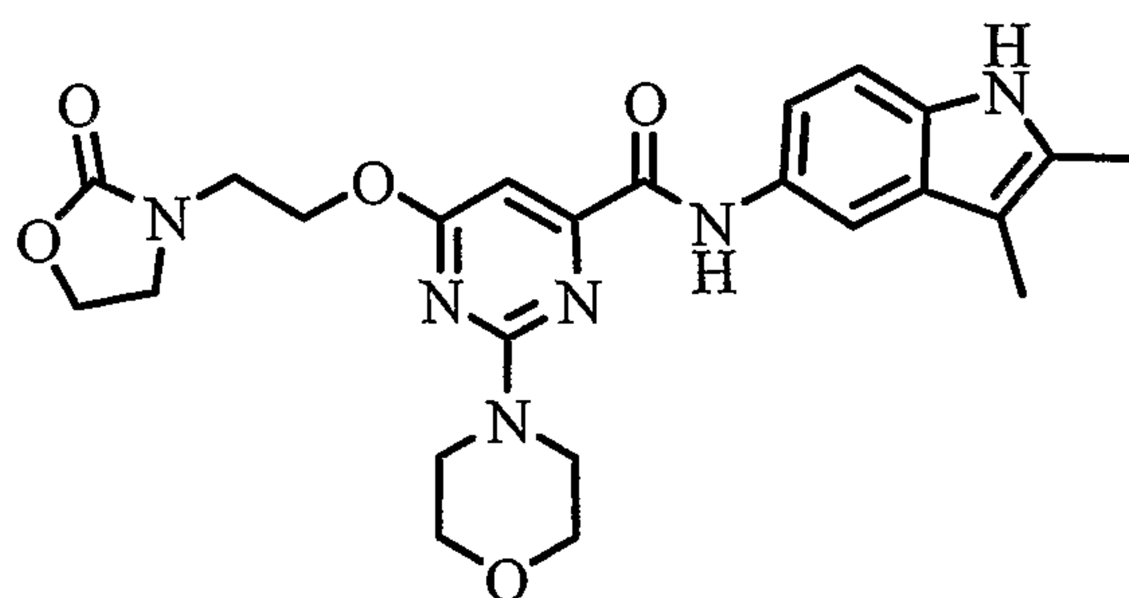
2-Morpholin-4-yl-6-[2-(2-oxo-oxazolidin-3-yl)-ethoxy]-pyrimidine-4-carboxylic acid
