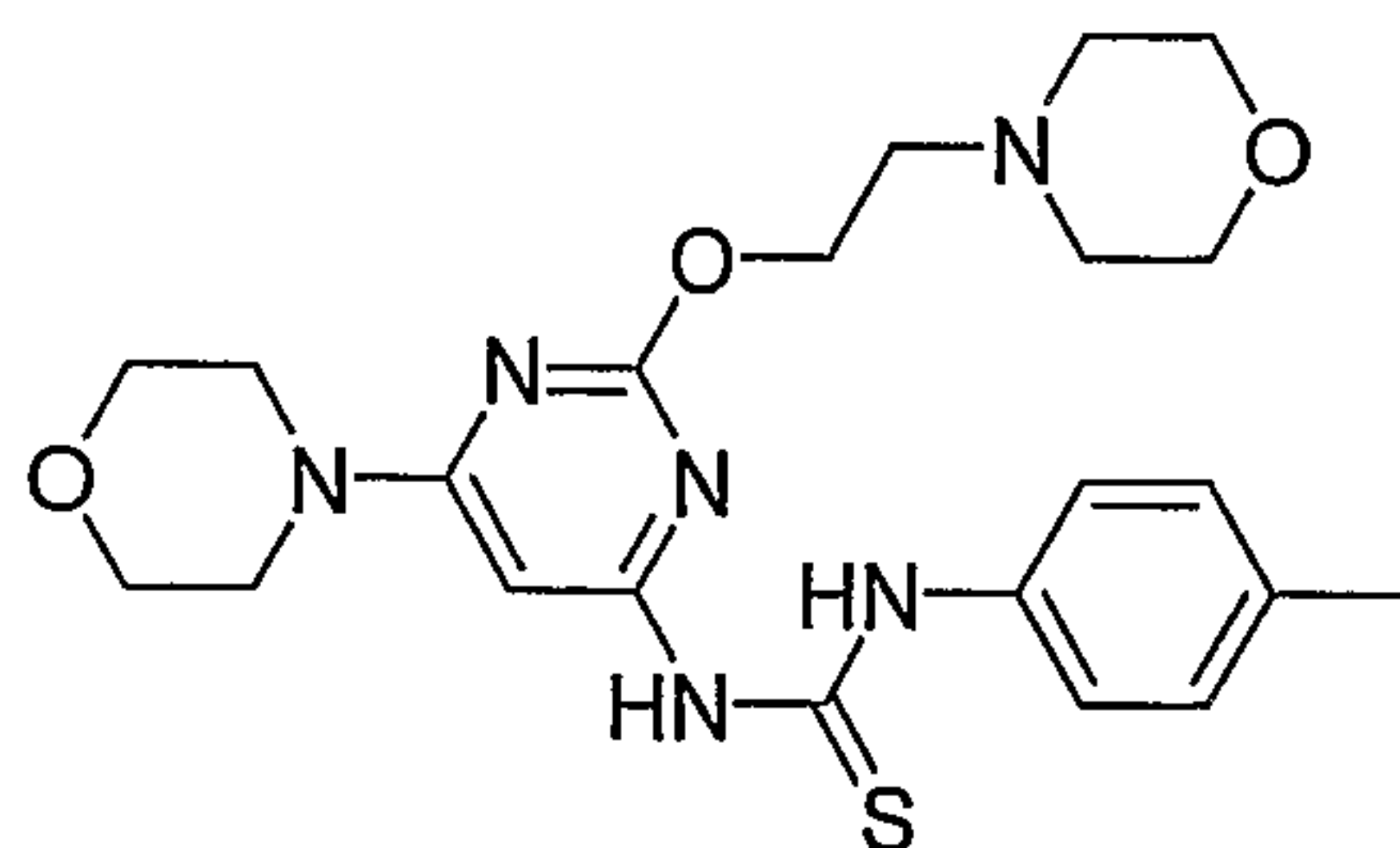
1-[6-Morpholin-4-yl-2-(2-morpholin-4-yl-ethoxy)-pyrimidin-4-yl]-3-p-tolyl-thiourea
