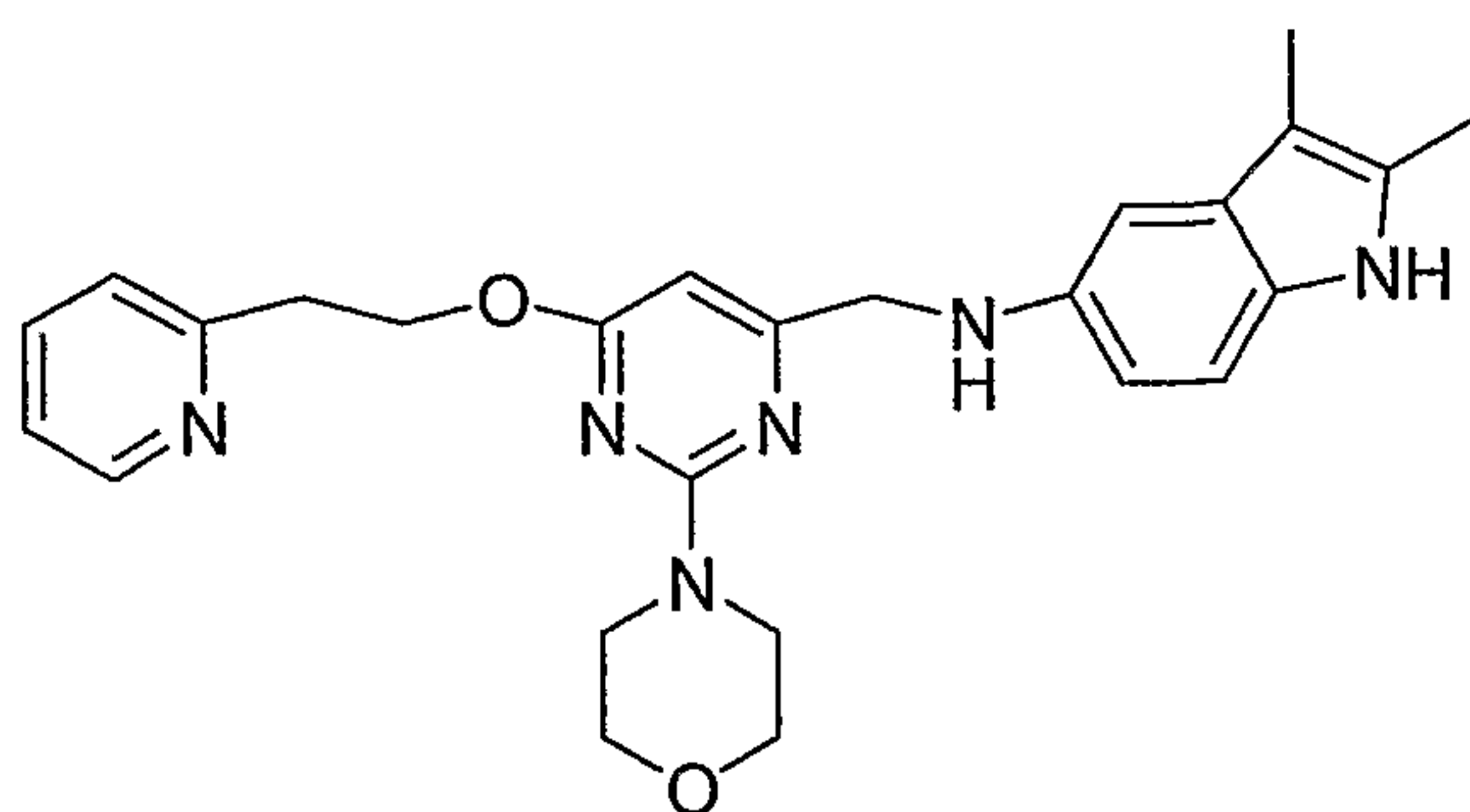
(2,3-Dimethyl-1H-indol-5-yl)-[2-morpholin-4-yl-6-(2-pyridin-2-yl-ethoxy)-pyrimidin-4-ylmethyl]-amine
