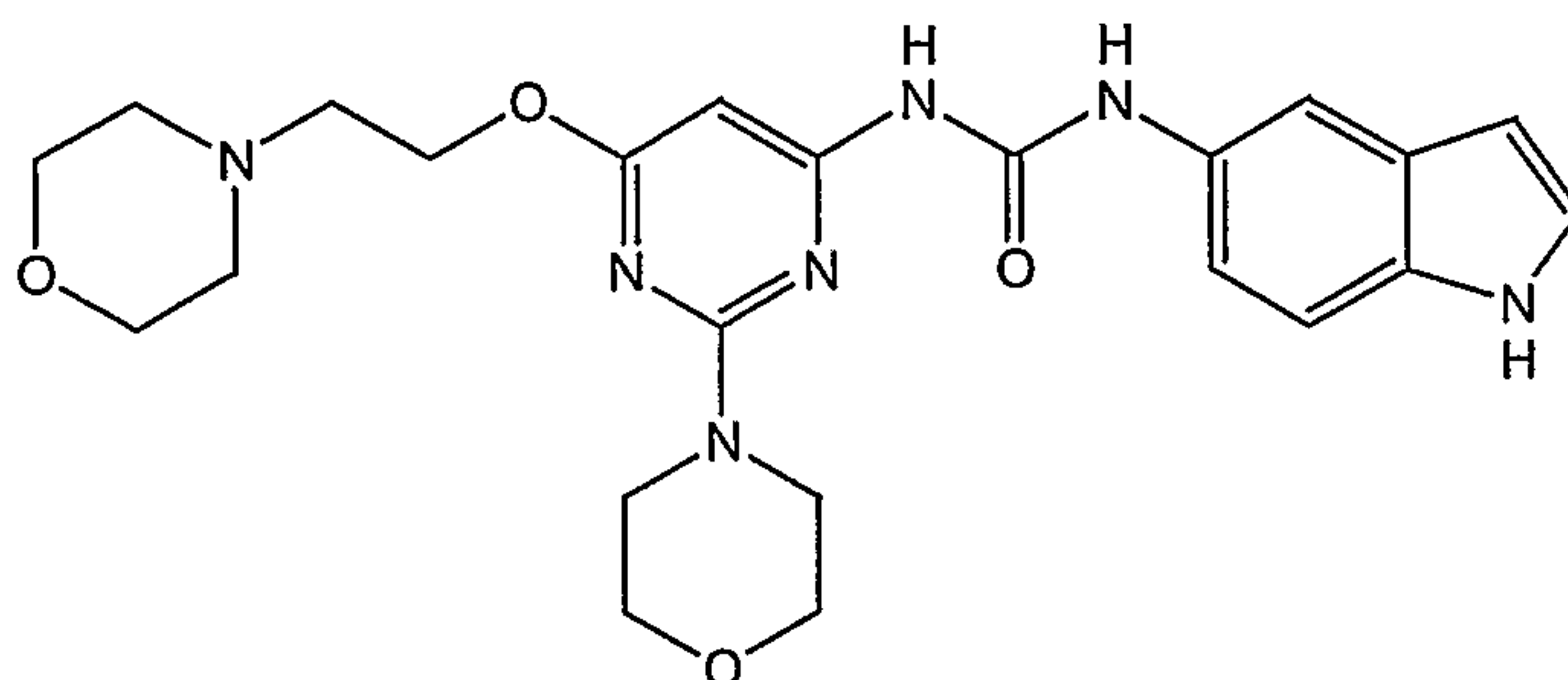
1-(1H-Indol-5-yl)-3-[2-morpholin-4-yl-6-(2-morpholin-4-yl-ethoxy)-pyrimidin-4-yl]-urea
