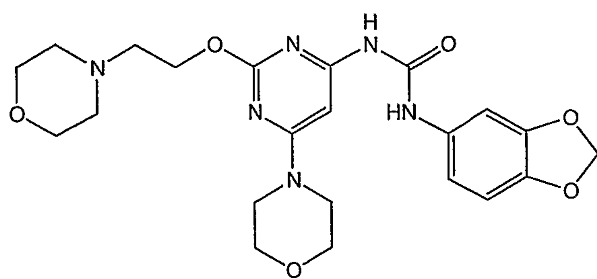
1-Benzo[1,3]dioxol-5-yl-3-[6-morpholin-4-yl-2-(2-morpholin-4-yl-ethoxy)-pyrimidin-4-yl]-urea
