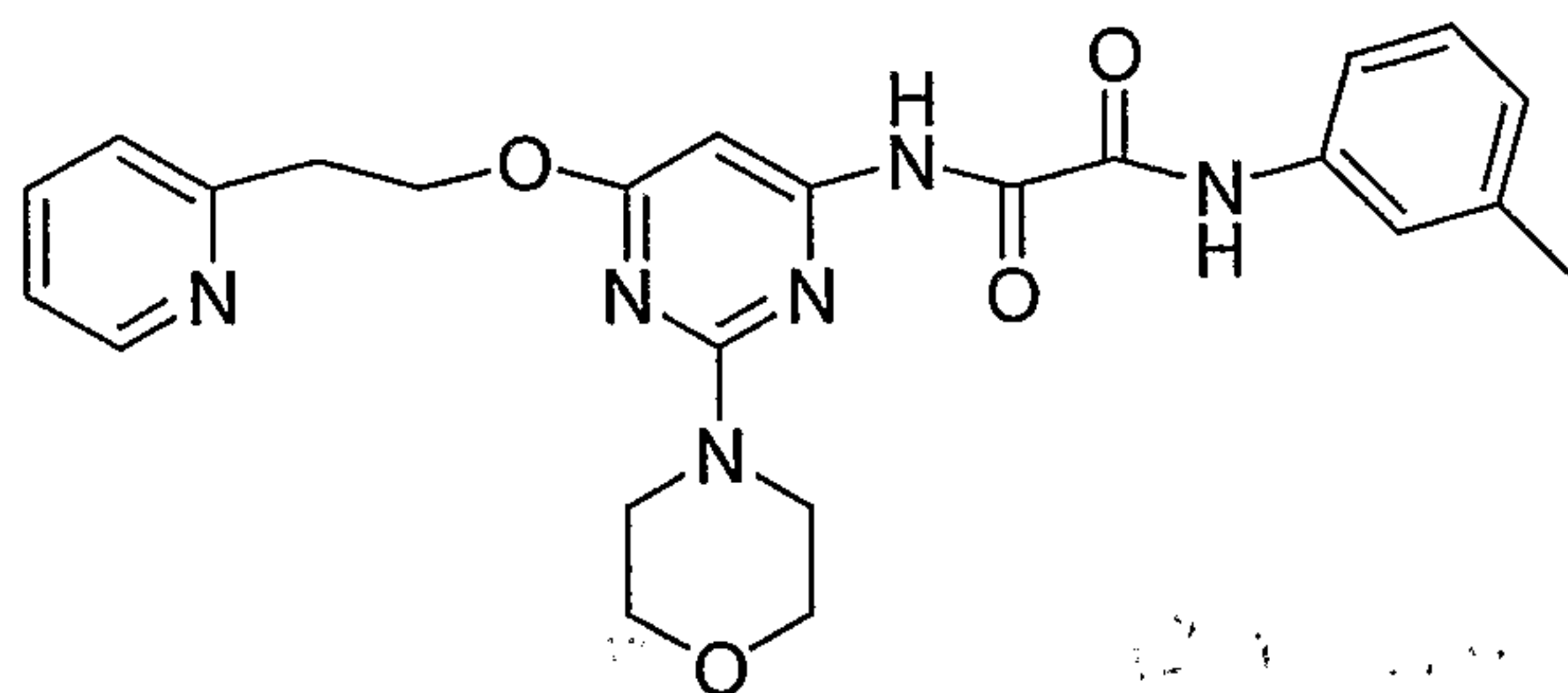
N-[2-Morpholin-4-yl-6-(2-pyridin-2-yl-ethoxy)-pyrimidin-4-yl]-N'-m-tolyl-oxalamide
