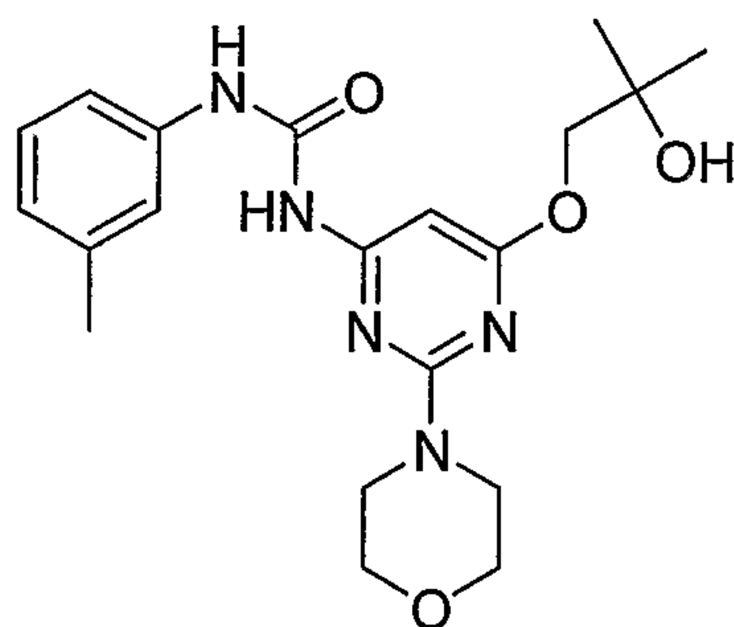
1-[6-(2-Hydroxy-2-methyl-propoxy)-2-morpholin-4-yl-pyrimidin-4-yl]-3-m-tolyl-urea
