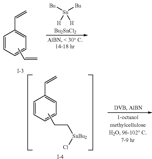
Scheme 6
