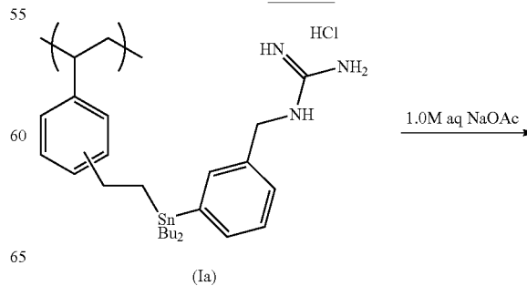
Scheme 9
