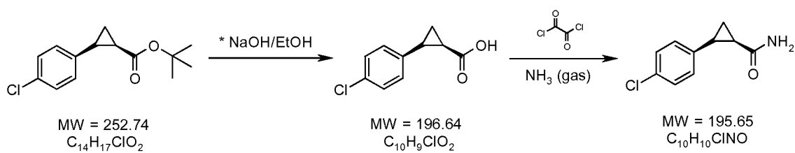
Scheme 14:
