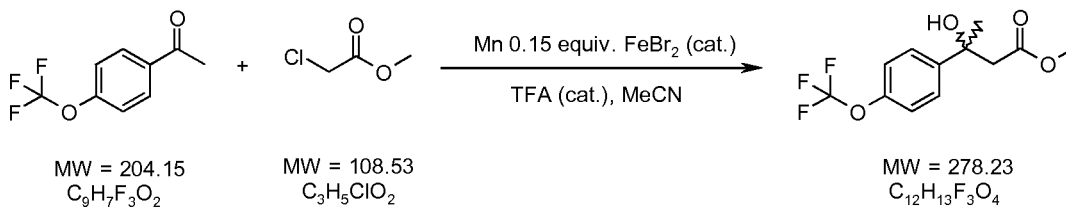
Scheme 12:
