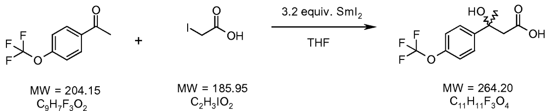
Scheme 11:
