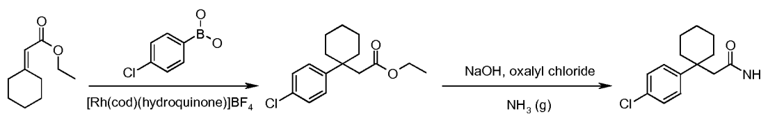
Scheme 4:
