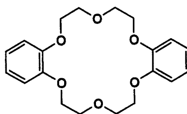
S-19
