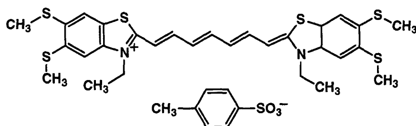
Infrared-sensitizing dye 1
