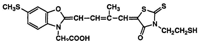
Panchromatic sensitizing dye 5
