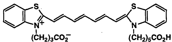
Infrared-sensitizing dye 8
