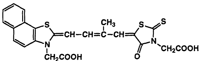
Panchromatic sensitizing dye 6
