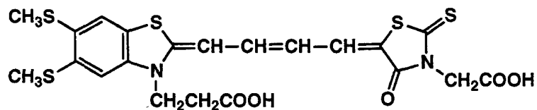
Panchromatic sensitizing dye 3
