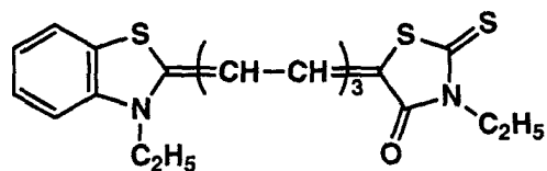
Infrared-sensitizing dye 5
