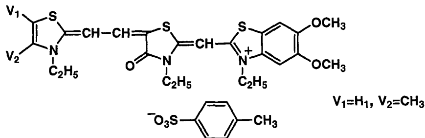
Panchromatic sensitizing dye 10
