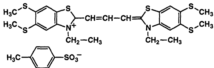
Panchromatic sensitizing dye 7
