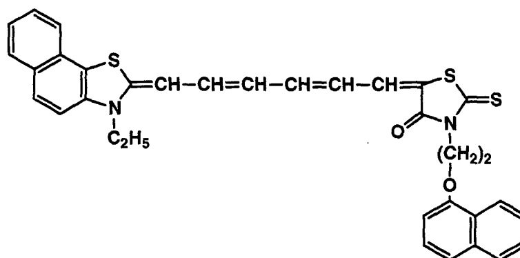
Infrared-sensitizing dye 7
