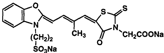
Panchromatic sensitizing dye 8
