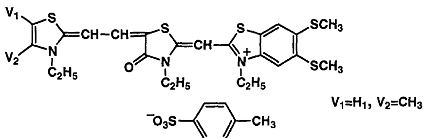
Panchromatic sensitizing dye 9
