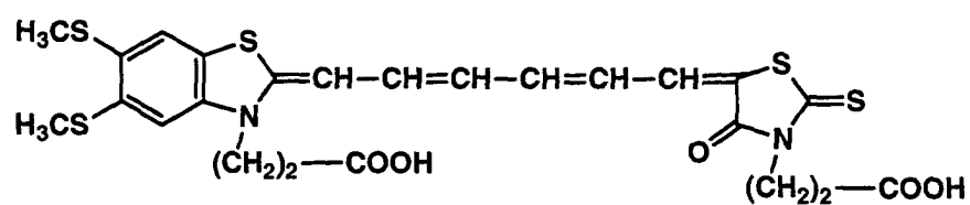
Infrared-sensitizing dye 4
