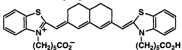
Infrared-sensitizing dye 9
