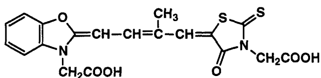
Panchromatic sensitizing dye 4
