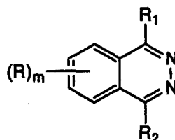
formula (1)
