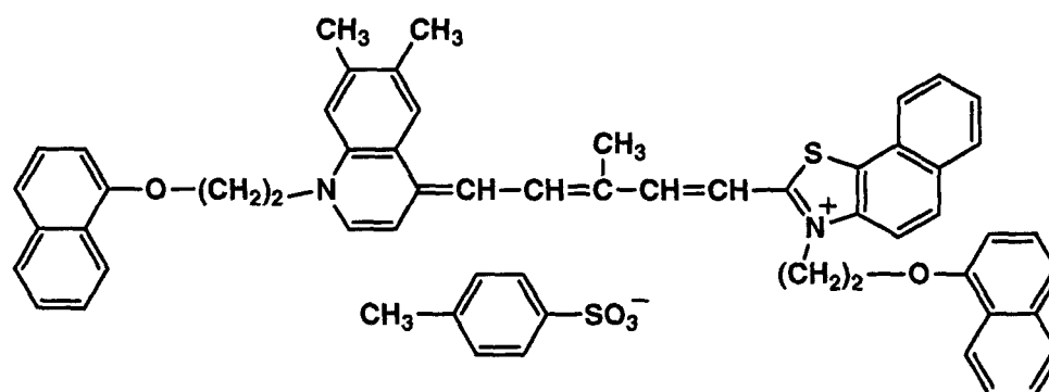
Infrared-sensitizing dye 6
