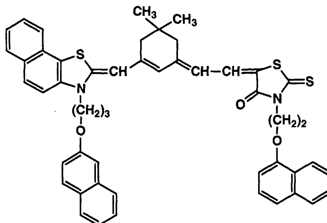
Infrared-sensitizing dye 3
