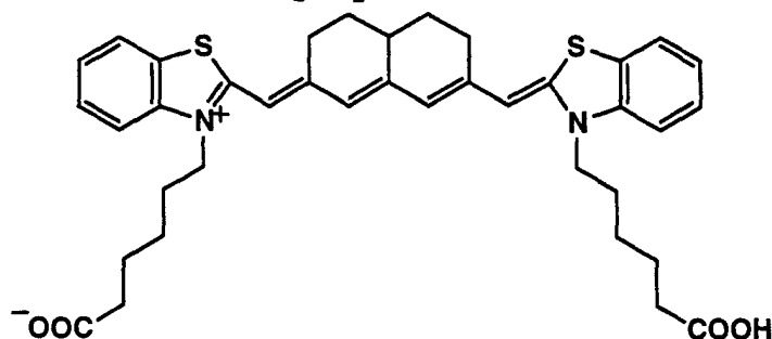
Infrared-sensitizing dye 2
