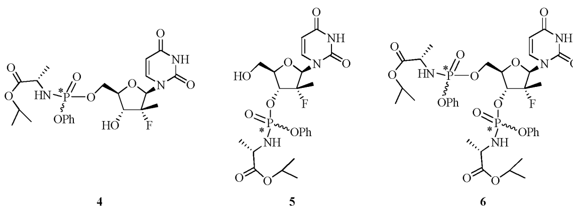
5'-O-phosphoramidate (2 diastereomers)
