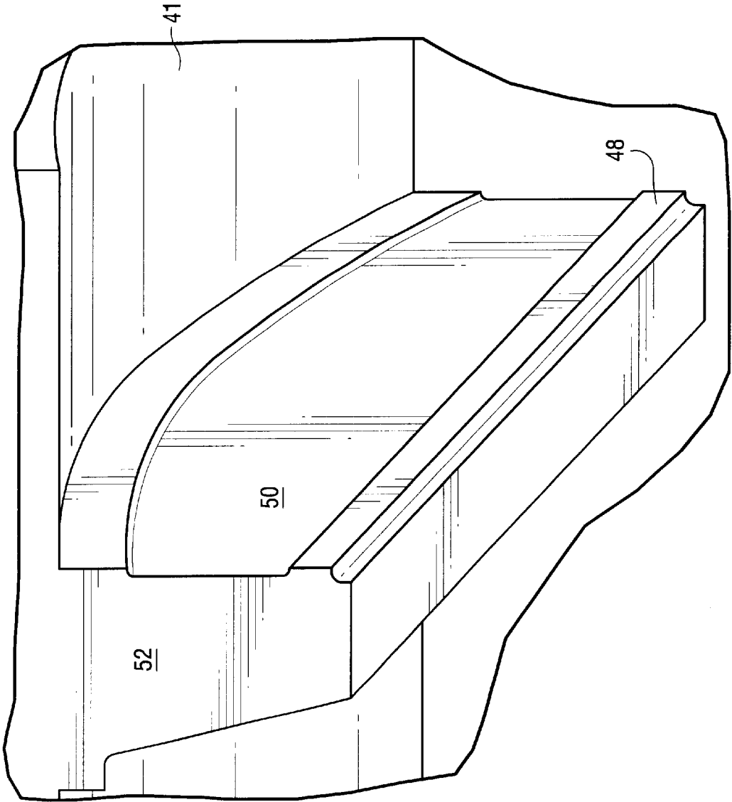
Fig. 3 (Prior Art)
