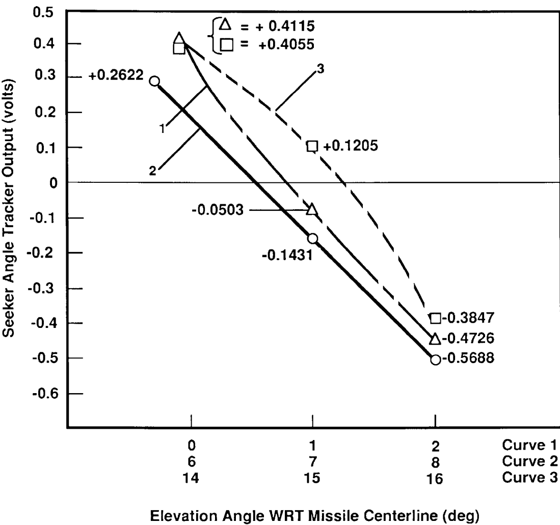
Figure 1. Transfer Characteristics
