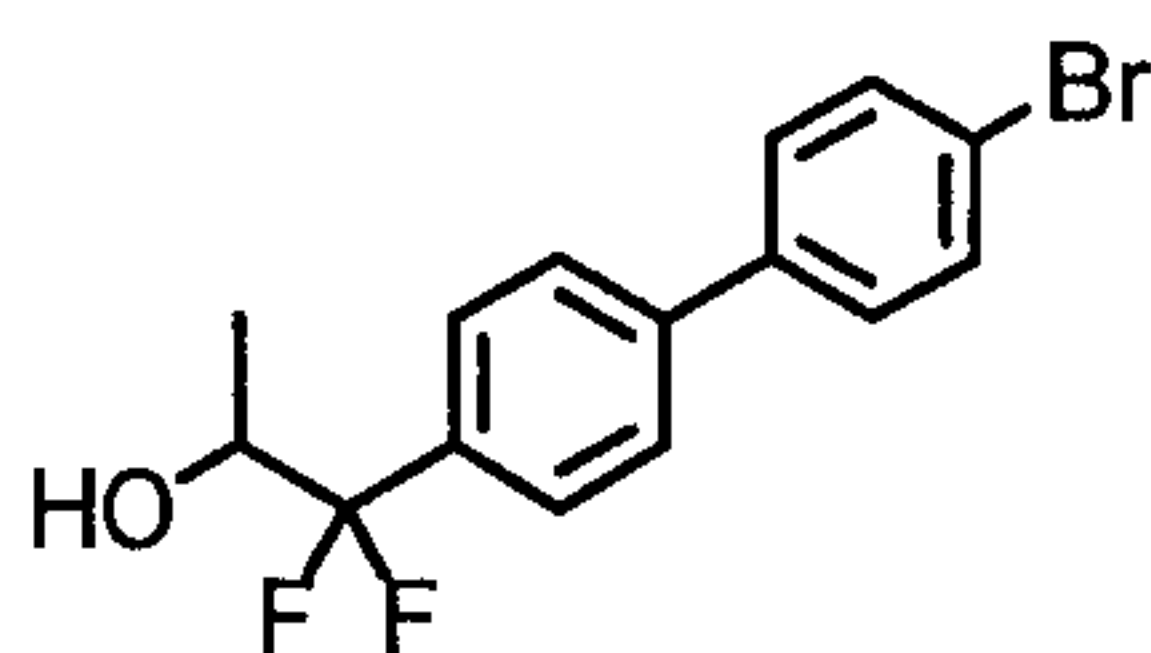
(1) 1-(4'-Bromobiphenyl-4-yl)-1,1-difluoropropan-2-ol [Chemical 108]
