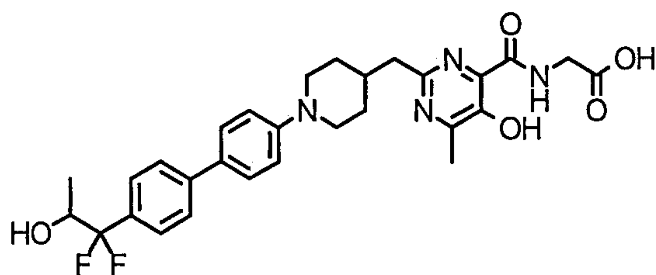
(1) 1-(4'-Bromobiphenyl-4-yl)-1,1-difluoropropan-2-ol [Chemical 108]
