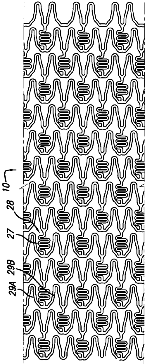
FIG. 4 PRIOR ART
