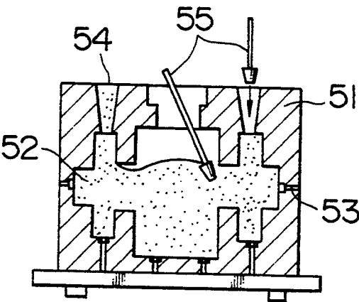
FIG. 17 PRIOR ART
