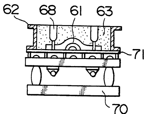
FIG. 20 PRIOR ART
