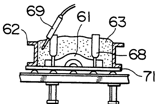
FIG. 19 PRIOR ART
