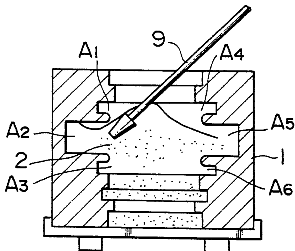
FIG. 13 PRIOR ART
