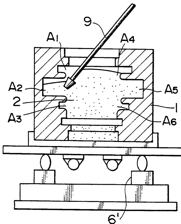
FIG. 14 PRIOR ART
