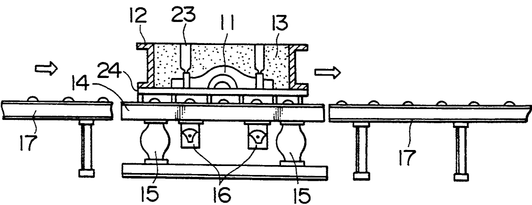
FIG. 16 PRIOR ART
