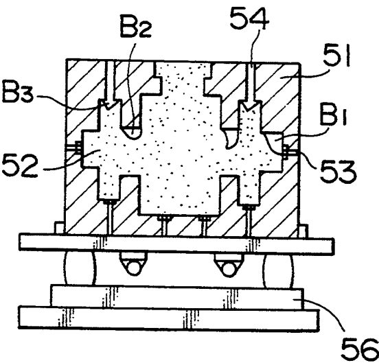
FIG. 18 PRIOR ART
