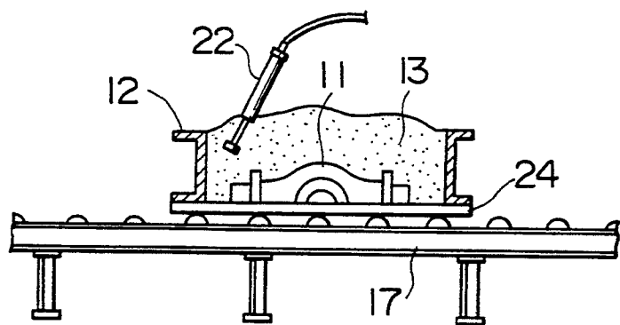
FIG. 15 PRIOR ART
