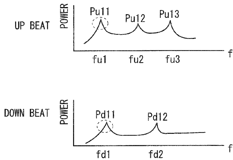
FIG. 2C FFT PROCESSING RESULT OF RECEIVING ANTENNA A1 (FREQUENCY SPECTRUM)
