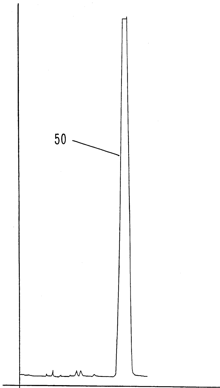
GLC PROFILE FOR EXAMPLE I(B).
