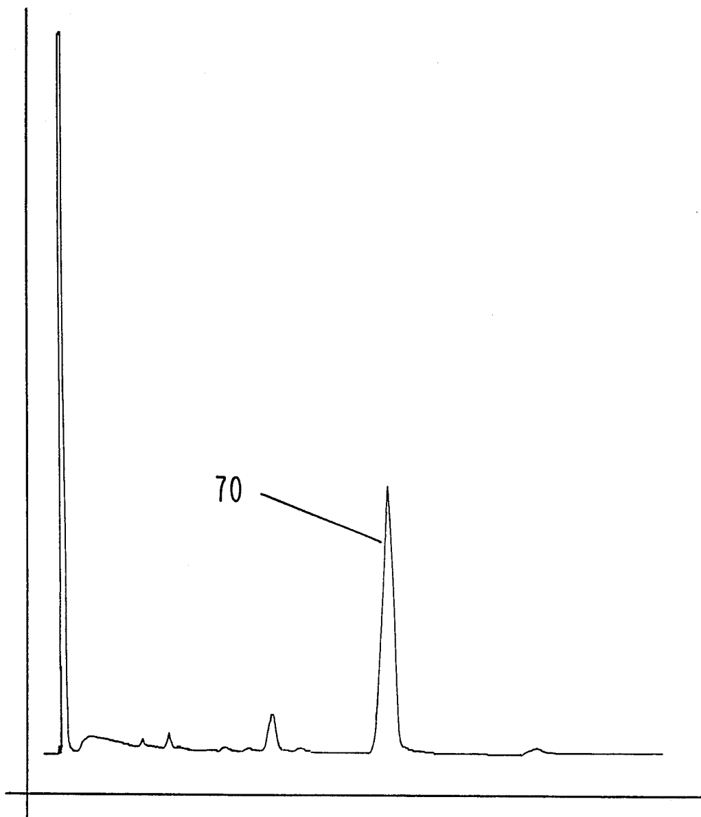
GLC PROFILE FOR EXAMPLE II.
