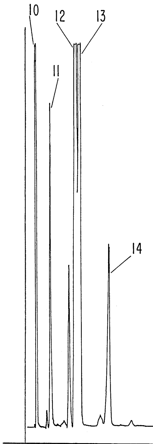
GLC PROFILE FOR EXAMPLE I(A).
