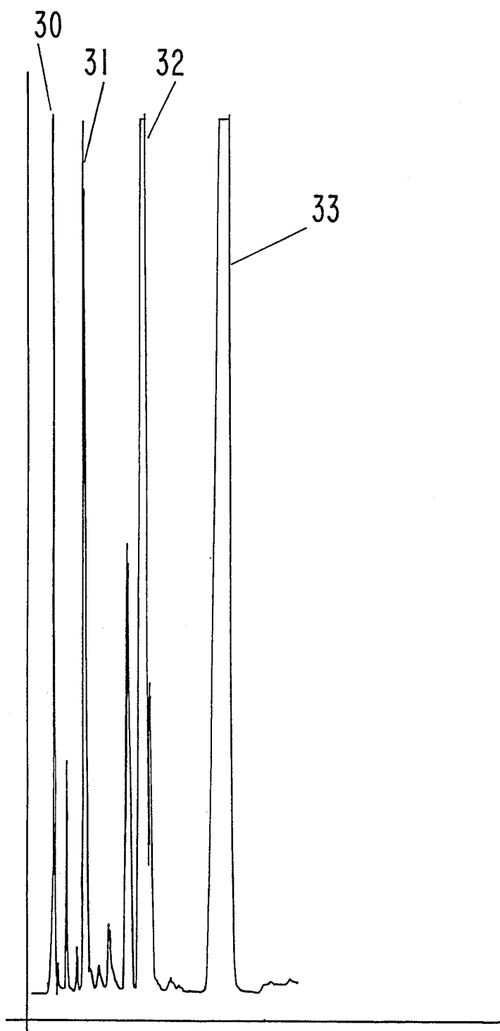
GLC PROFILE FOR EXAMPLE I(A).
