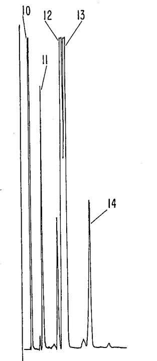
GLC PROFILE FOR EXAMPLE I(A).
