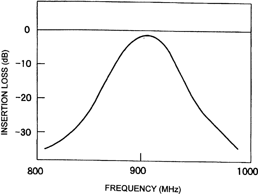
FIG. 18 PRIOR ART
