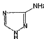
3-Amino-1,2,4-triazole
