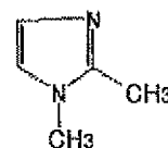
1,2-Dimethylimidazole
