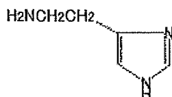
Histamine
