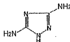
3,5-Diamino-1,2,4-triazole
