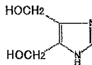
4,5-Bis(hydroxymethyl)imidazole
