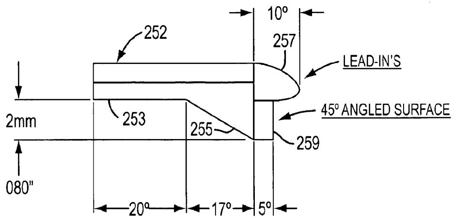
CAM SECTION
