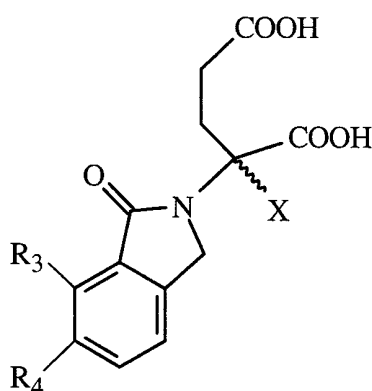
2-Phthalimidinoglutaric acid analogs
