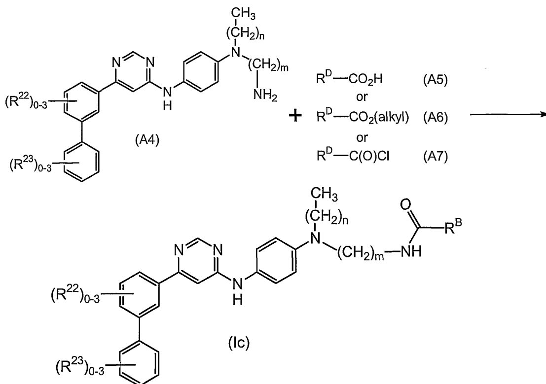
Scheme 3
