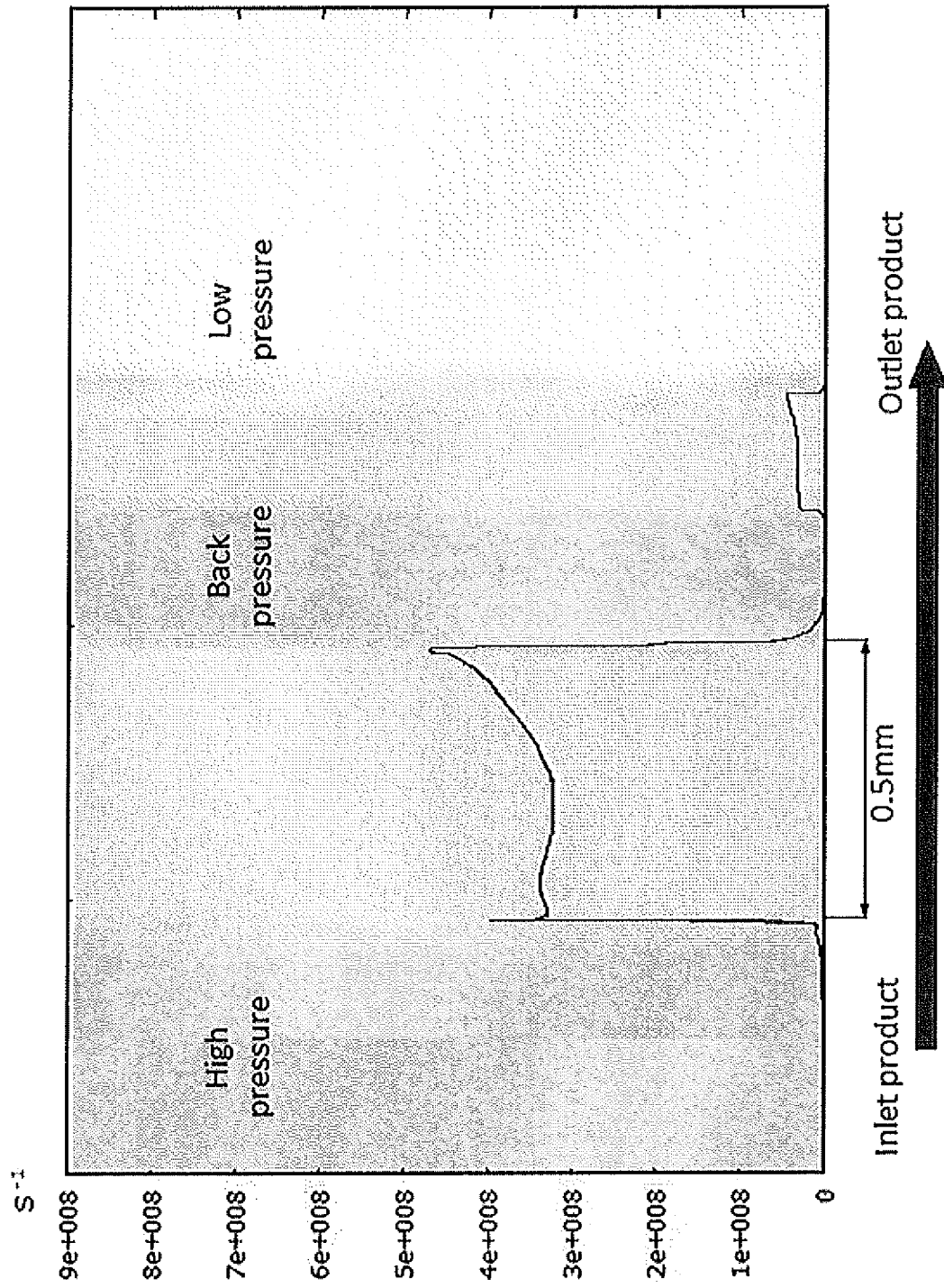
Fig.3C Pattern of shear rate new version C
