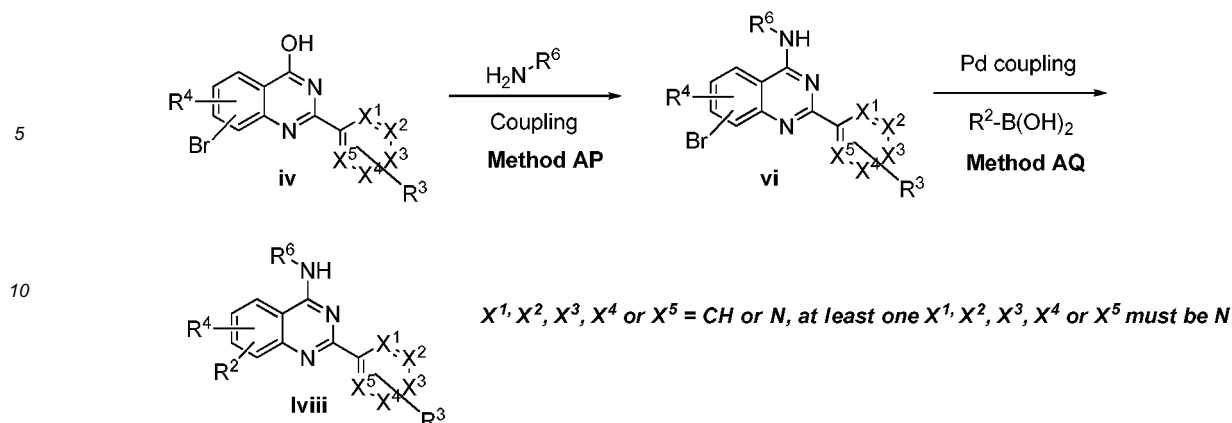
Scheme 75: Representative synthesis of compounds of formula lviii (see Scheme 74)
