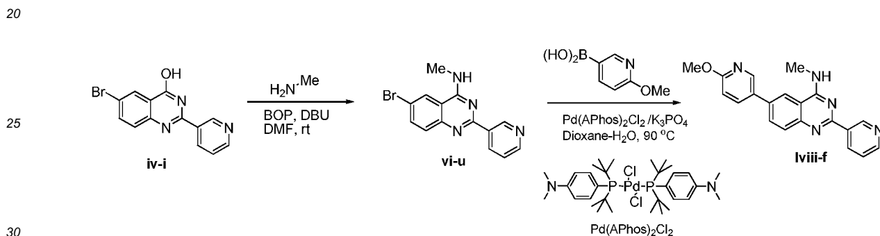
Scheme 75: Representative synthesis of compounds of formula lviii (see Scheme 74)
