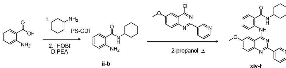
Scheme 28: Representative synthesis of compounds of formula xiv (see Scheme 27)
