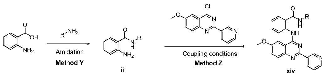
Scheme 28: Representative synthesis of compounds of formula xiv (see Scheme 27)
