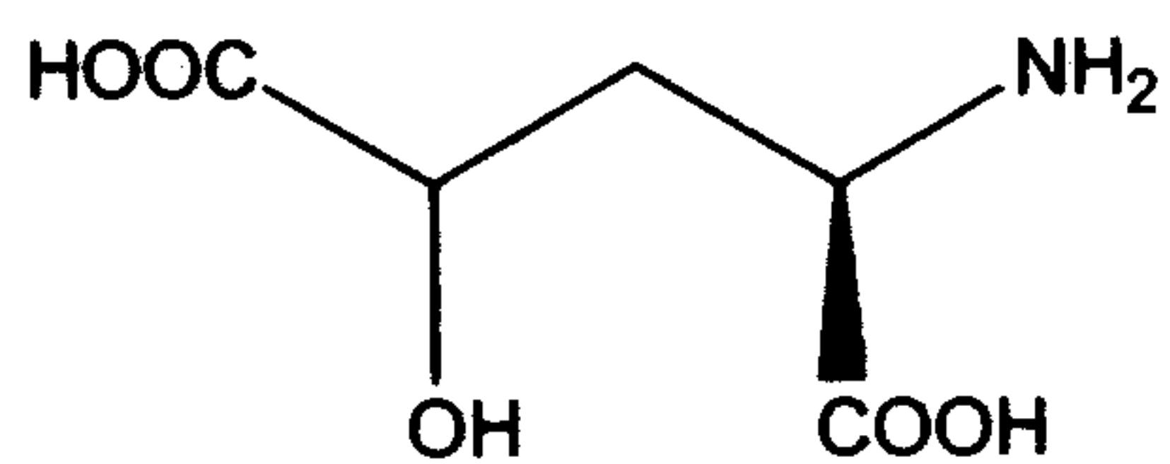
D-gamma-hydroxy glutamate
