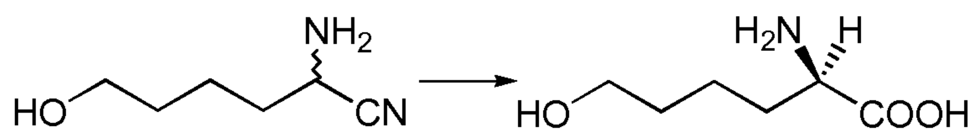
5-hydroxypentanal aminonitrile
