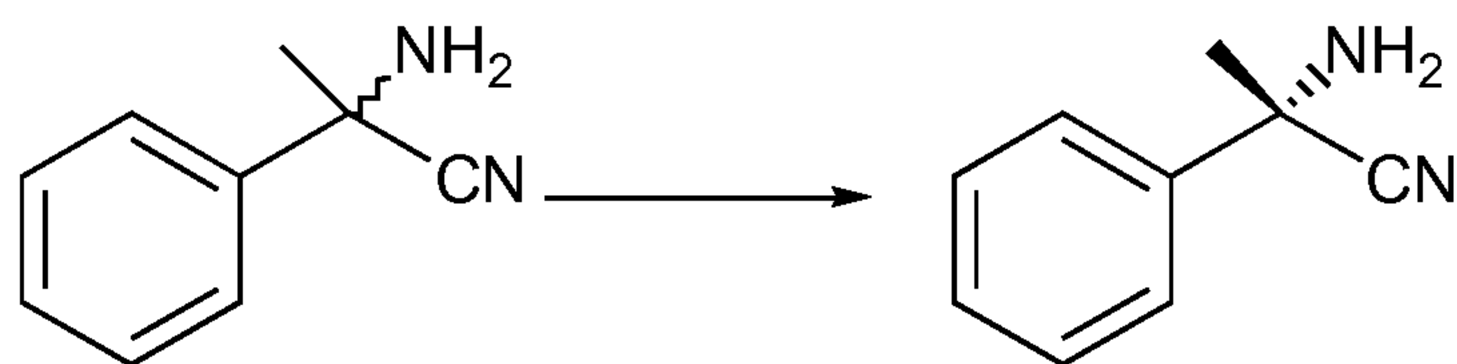
2-methylphenylglycinonitrile
