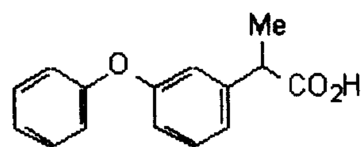
Fenoprofen
