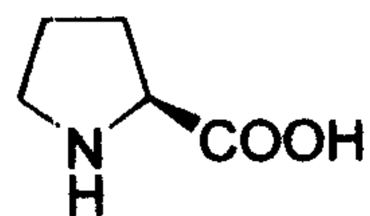
2-carboxy-cyclobutyl amine
