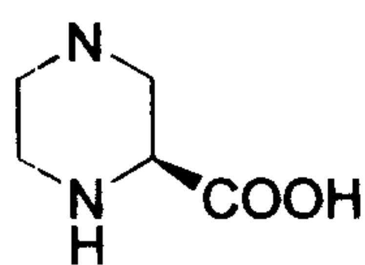
2-carboxy-piperazine
