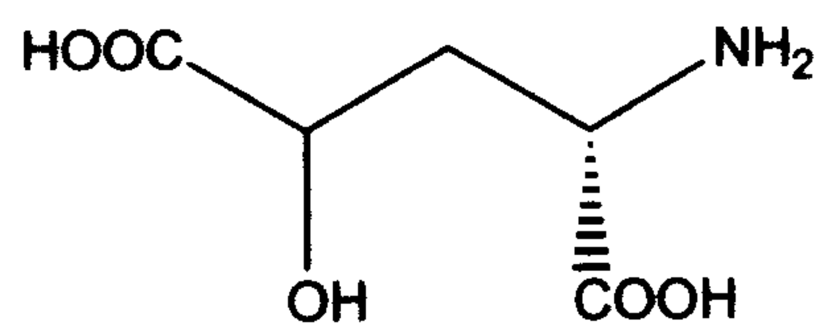
L-gamma-hydroxy glutamate
