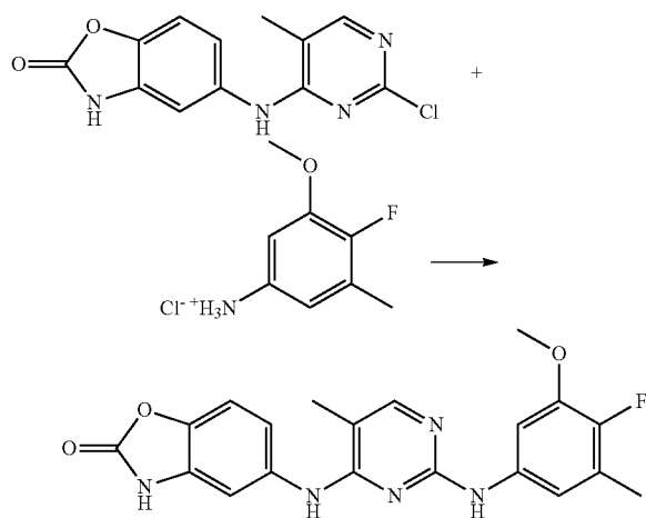
5-(2-(4-fluoro-3-methoxy-5-methylphenylamino)-5-methylpyrimidin-4-ylamino)benzo[d]oxazol-2(3H)-one
