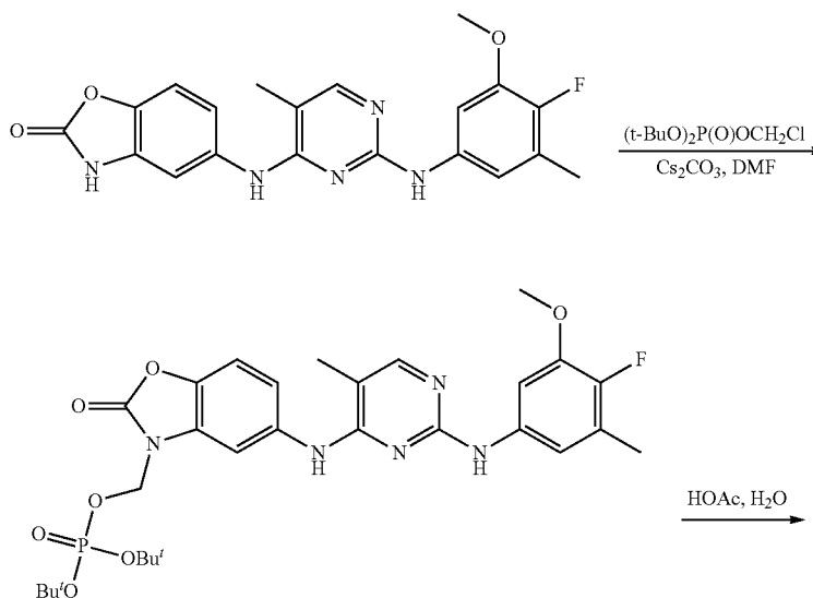
Scheme (XI)
