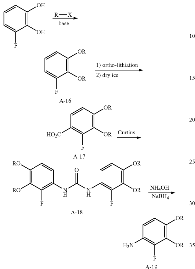
Scheme (III)
