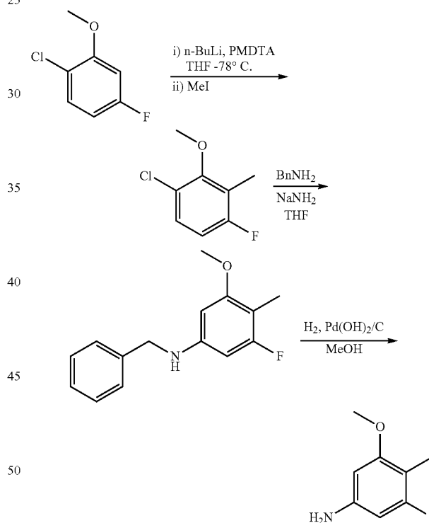
Scheme (IX)
