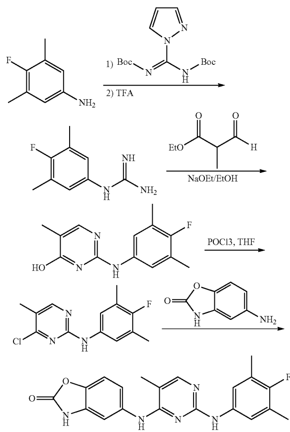
Scheme (X)
