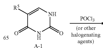
Scheme (I)
