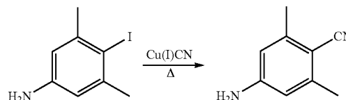
Scheme (VI)
