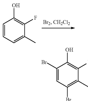
Scheme (VII)
