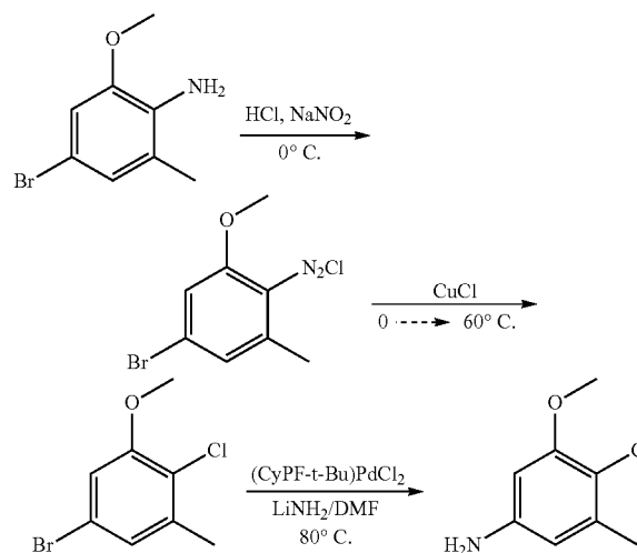
Scheme (VIII)
