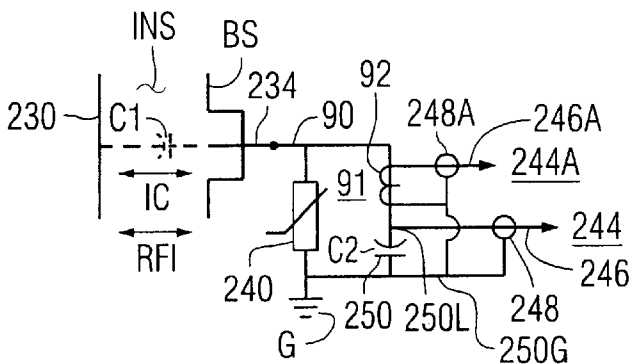
FIG. 25 PRIOR ART
