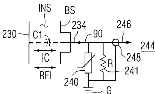
FIG. 22 PRIOR ART
