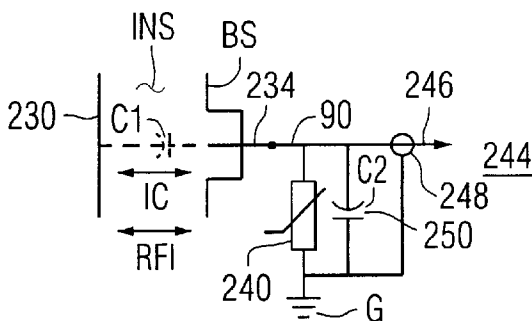
FIG. 23 PRIOR ART
