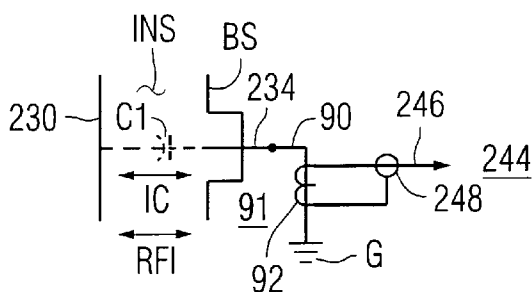
FIG. 21 PRIOR ART
