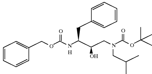
Preparation of N-[[3S-(phenylmethylcarbamoyl)amino]-2R-hydroxy-4-phenyl]-1-[(2-methylpropyl)amino]-2-(1,1-dimethylethoxy)carbonyl]butane
