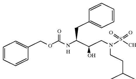
Preparation of phenylmethyl [2R-hydroxy-3-[(3-methylbutyl) (methylsulfonyl)amino]-1S-(phenylmethyl) propyl]carbamate
