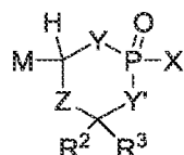
[0038] (Ib)
