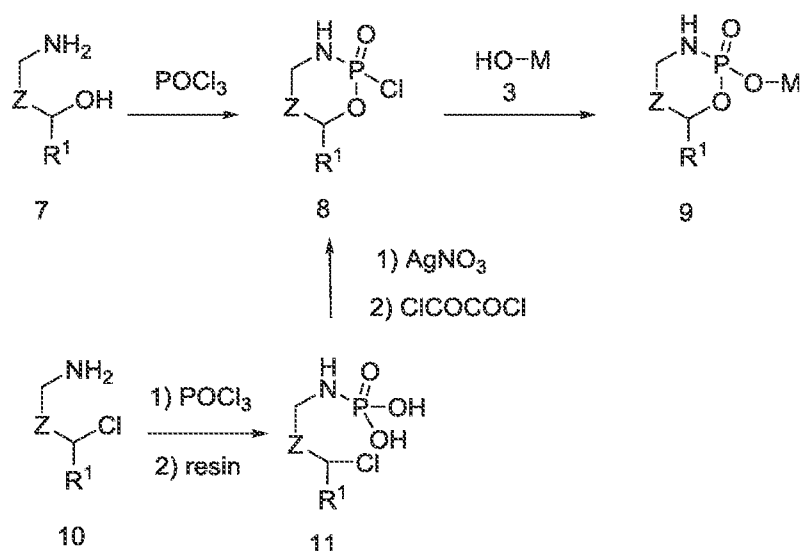
Scheme II
