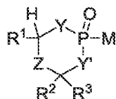
[0024] (Ia)
