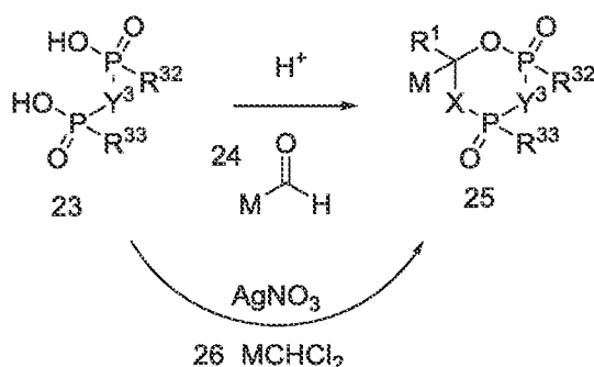
[0393] Scheme V
