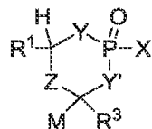
[0051] (Ic)
