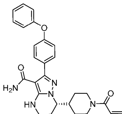
15 Compound 1
