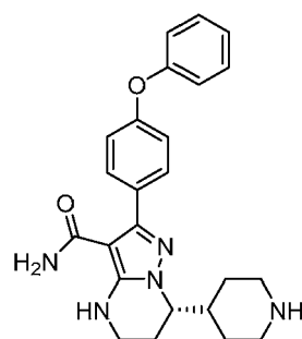
Formula 1f
