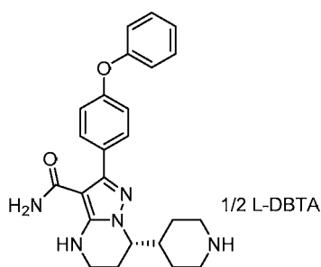
BG-13
