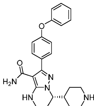
BG-12.
