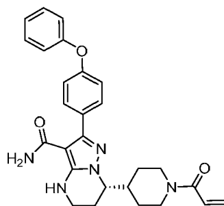
Compound 1 .
