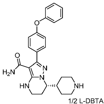
Compound BG-13 .
