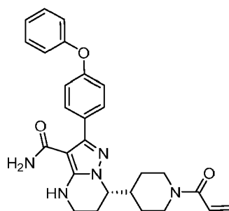
Compound 1
