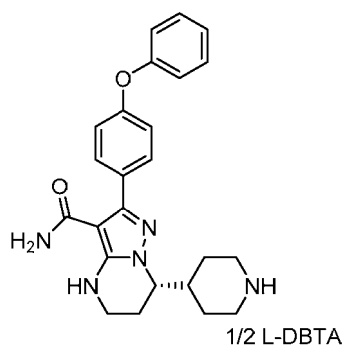
Compound BG-13
