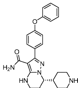
BG-12
