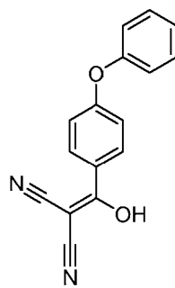
BG-2
