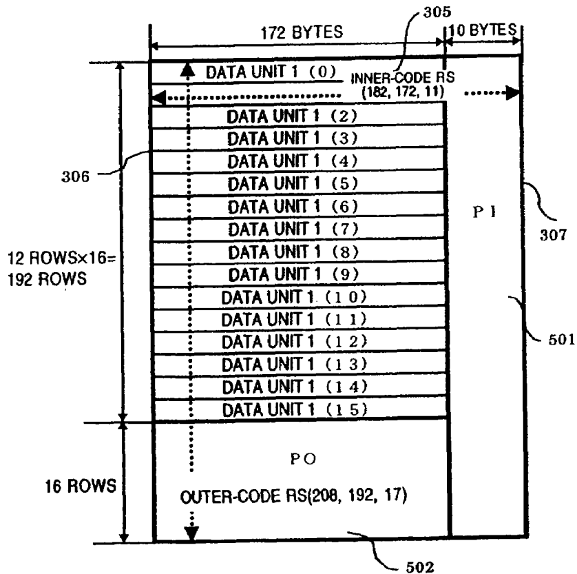
FIG. 6 (Prior Art)
