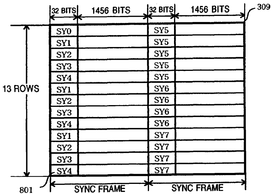
FIG. 8 (Prior Art)
