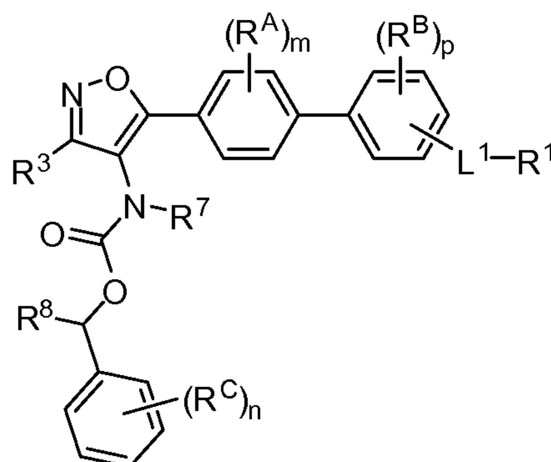
Formula (I)
