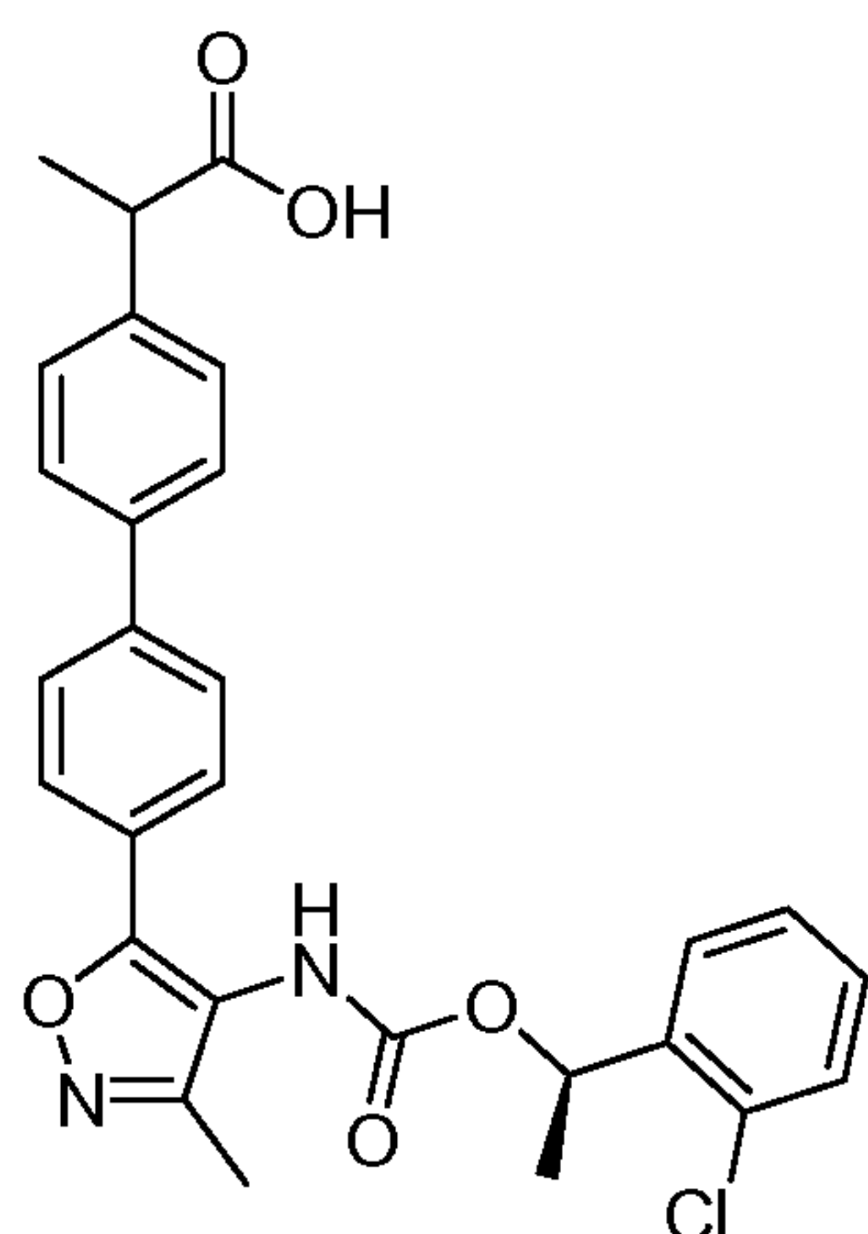
Compound 31
