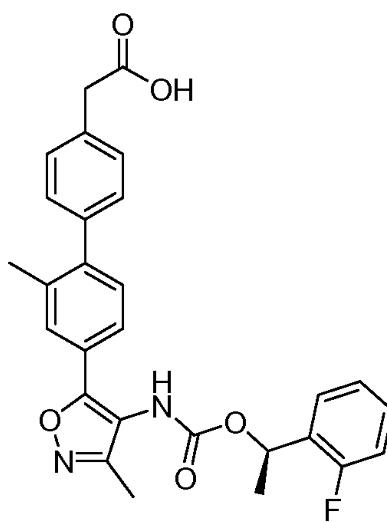
Compound 25
