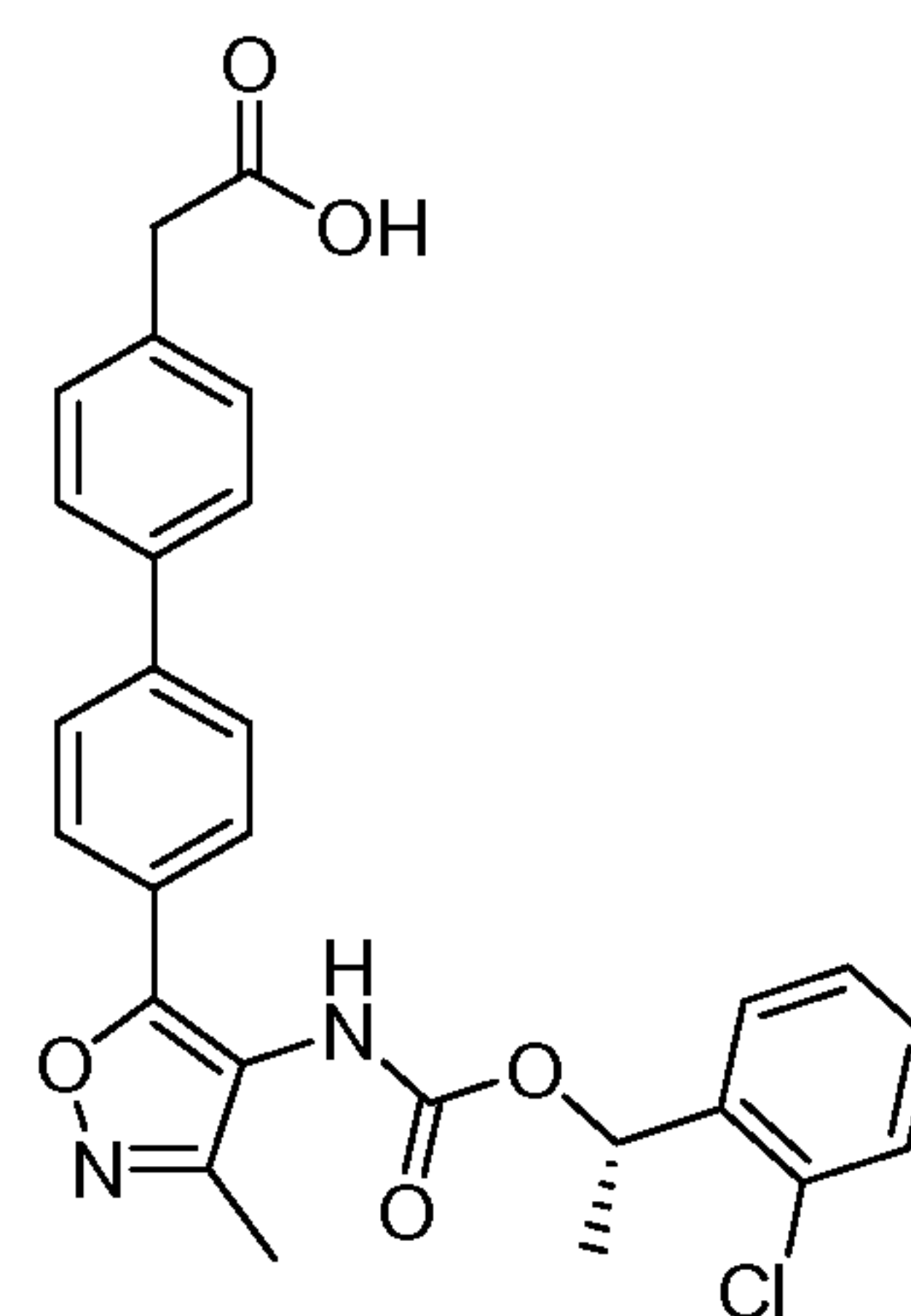
Compound 35
