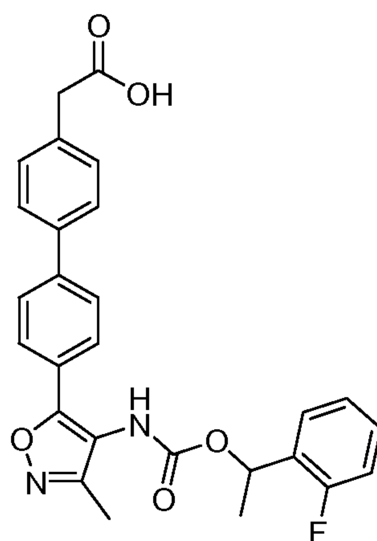
Compound 4
