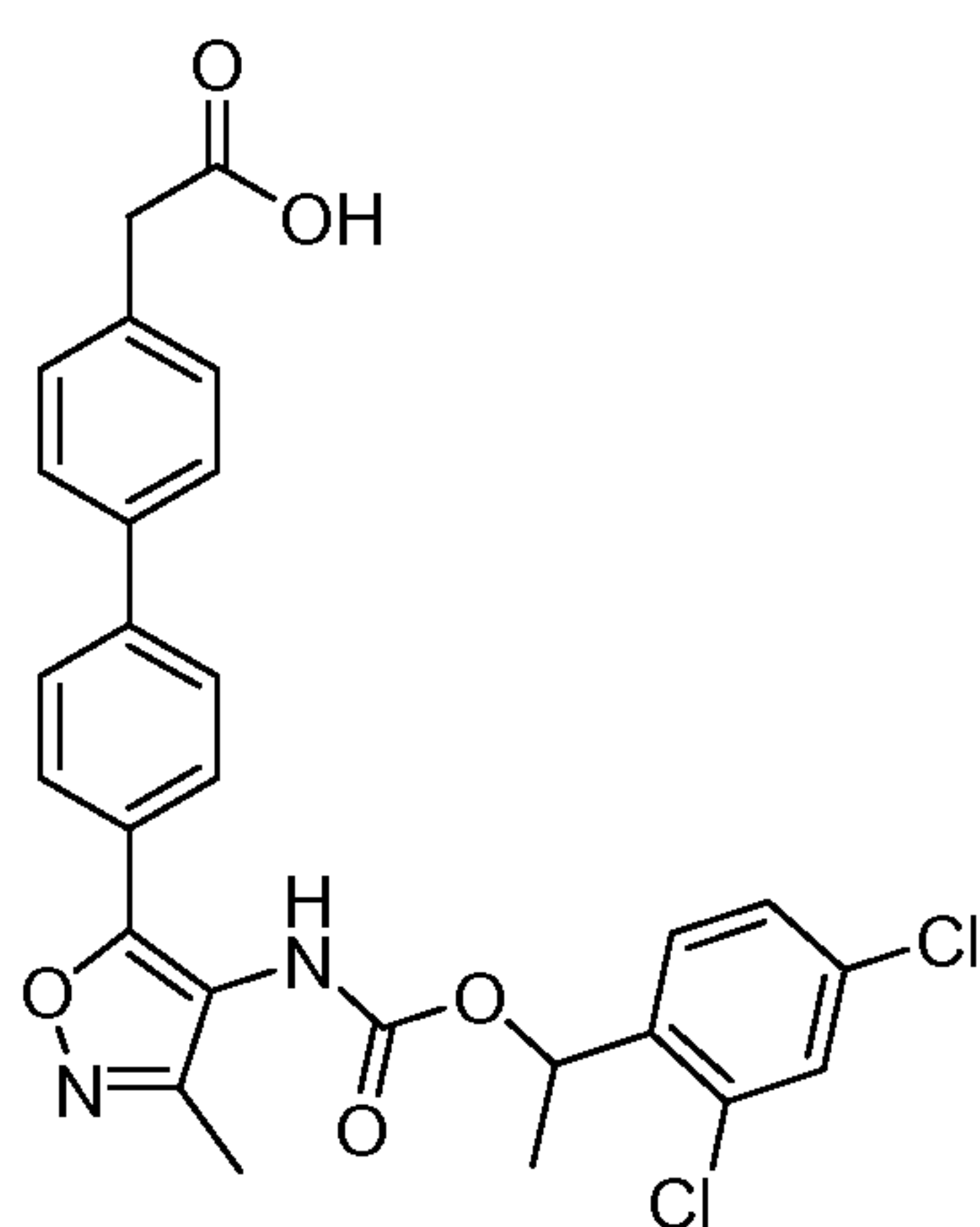
Compound 3
