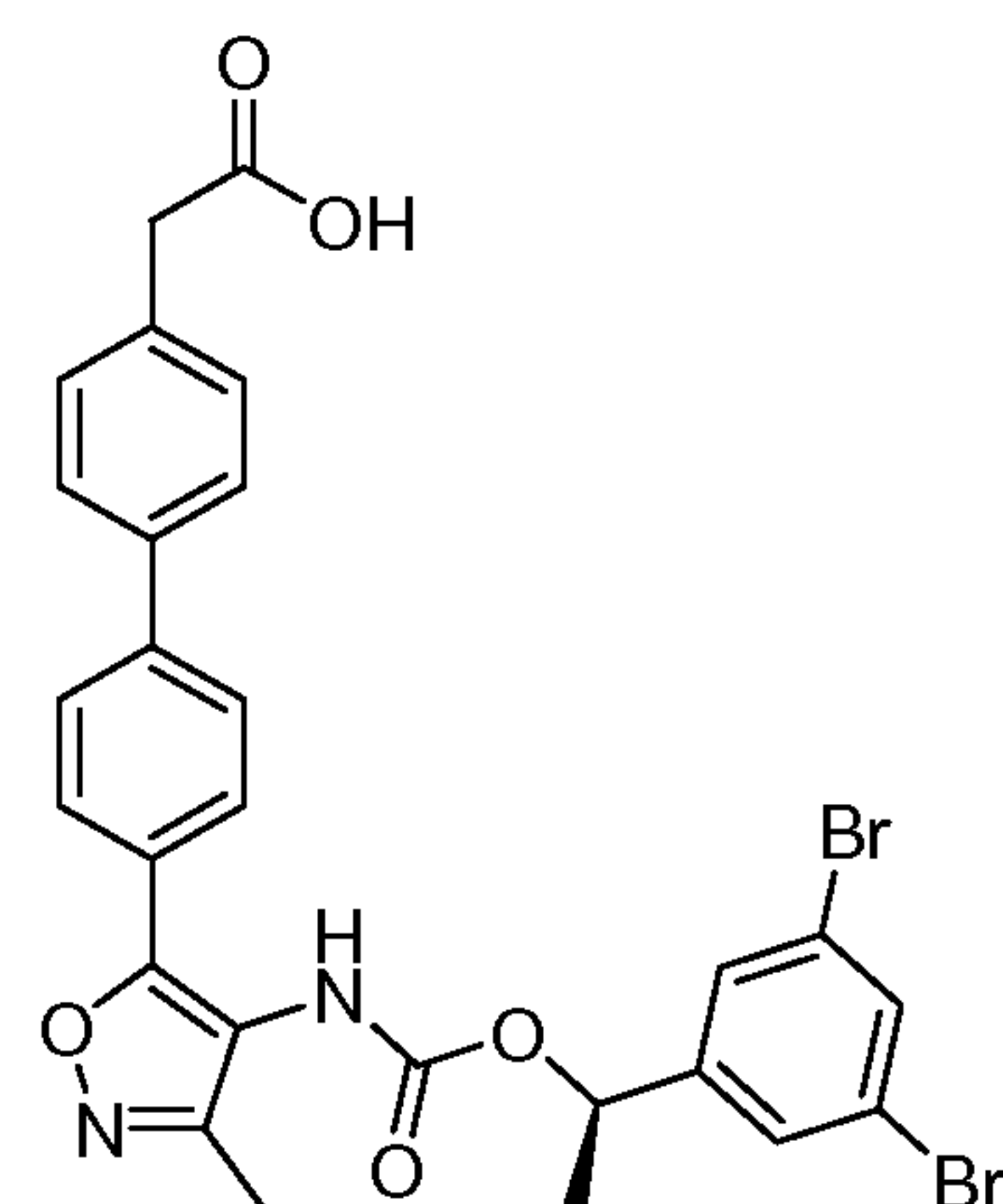
Compound 56
