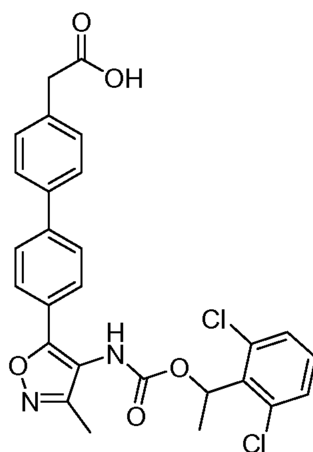
Compound 32
