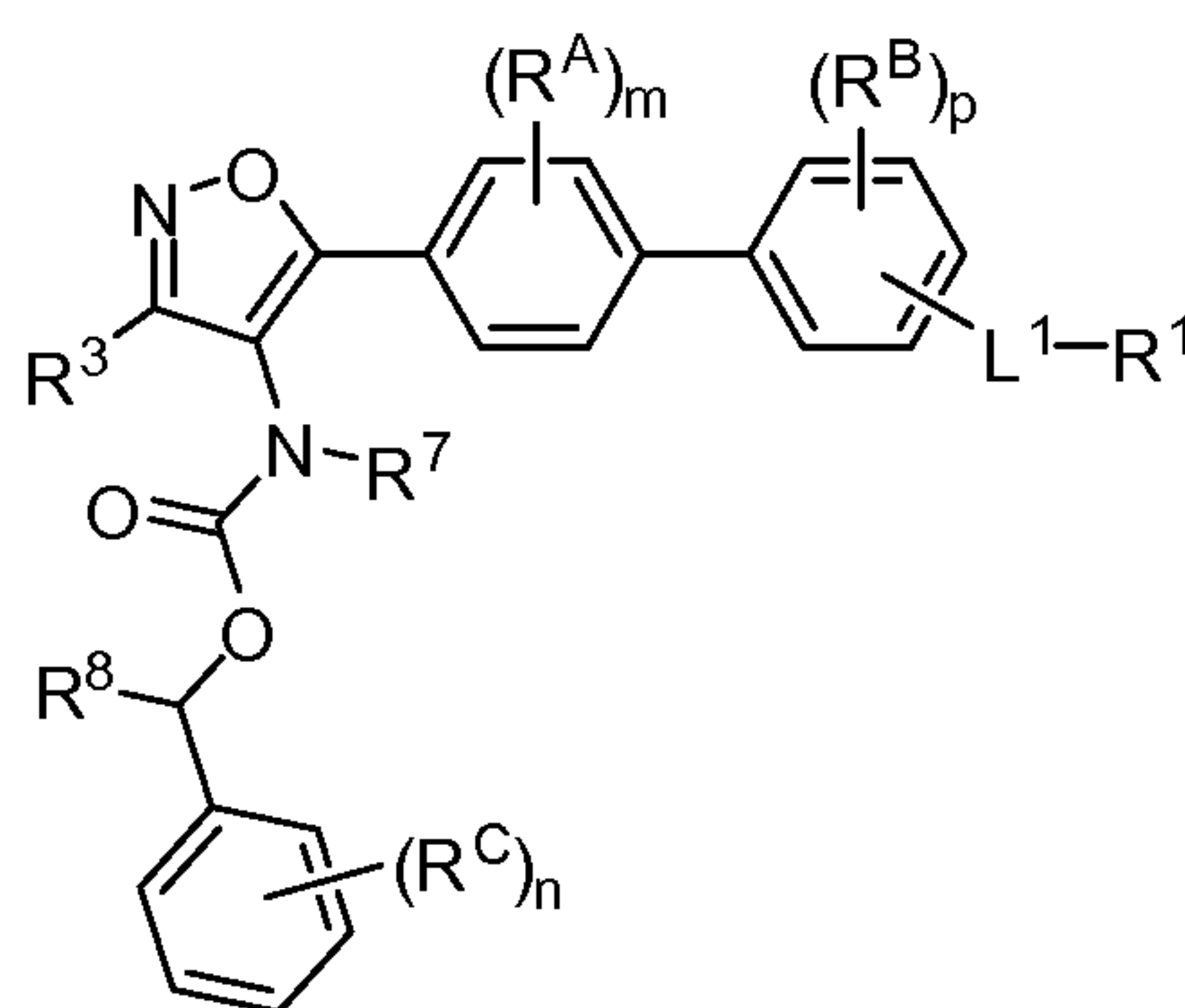
Formula (I)
