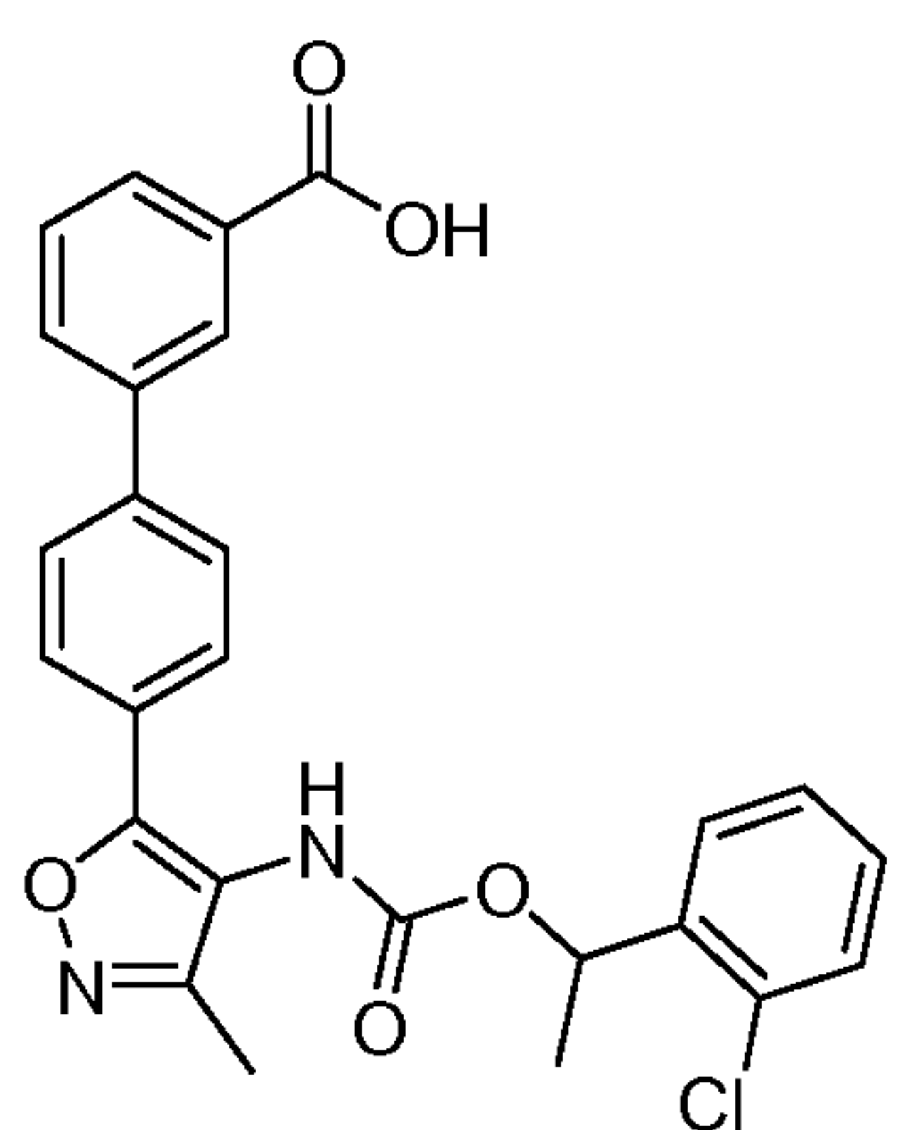
Compound 22
