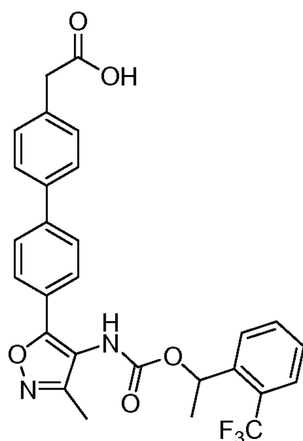
Compound 1
