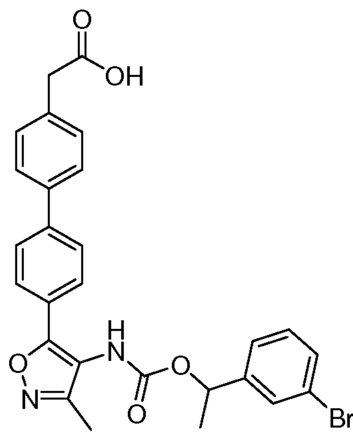
Compound 5
