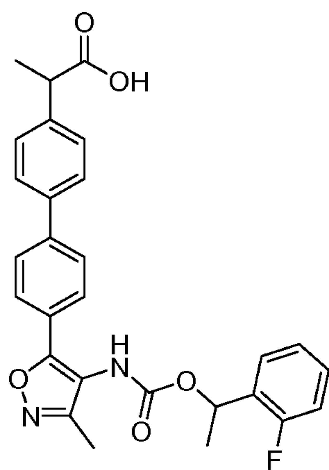
Compound 20
