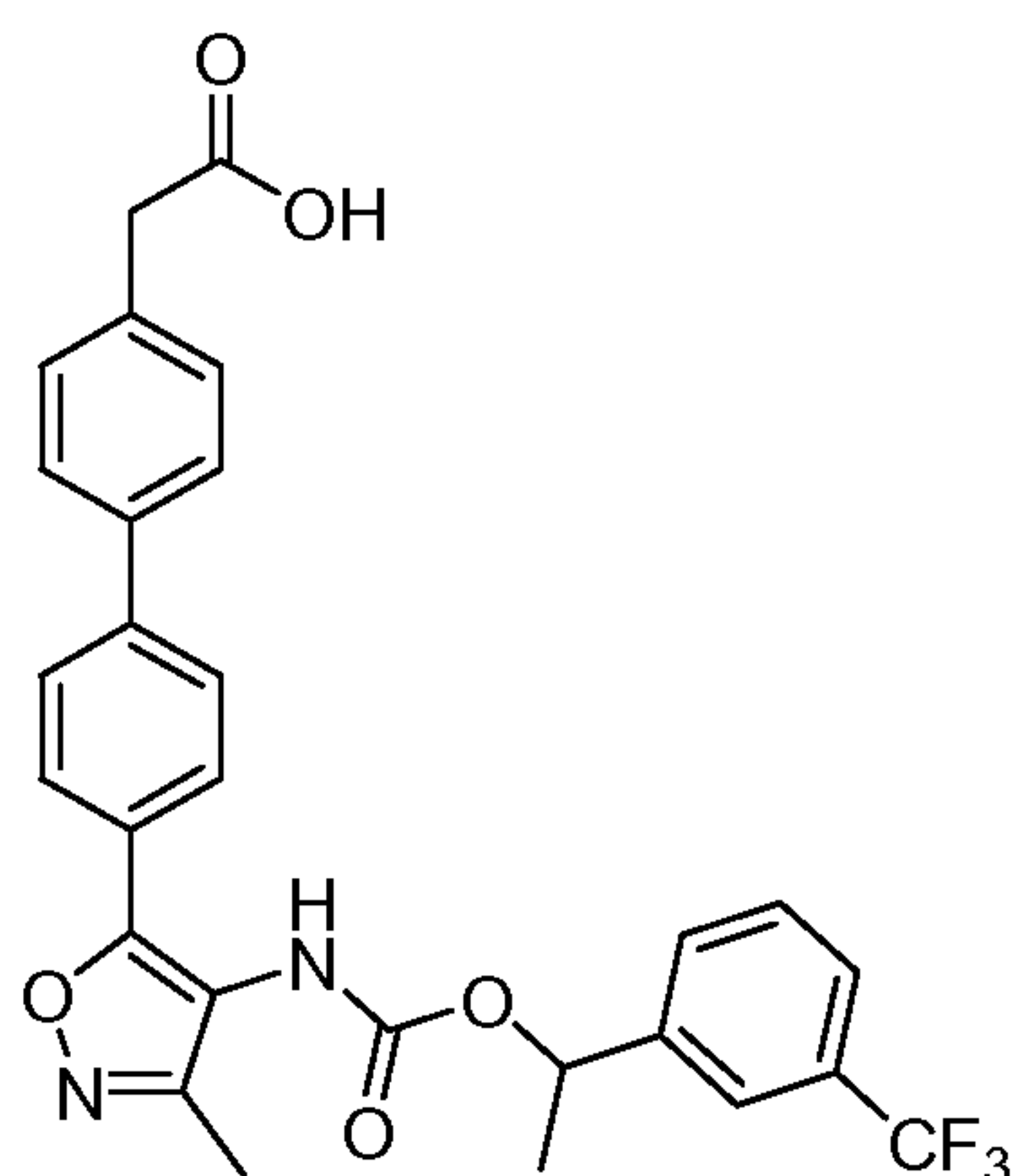
Compound 2
