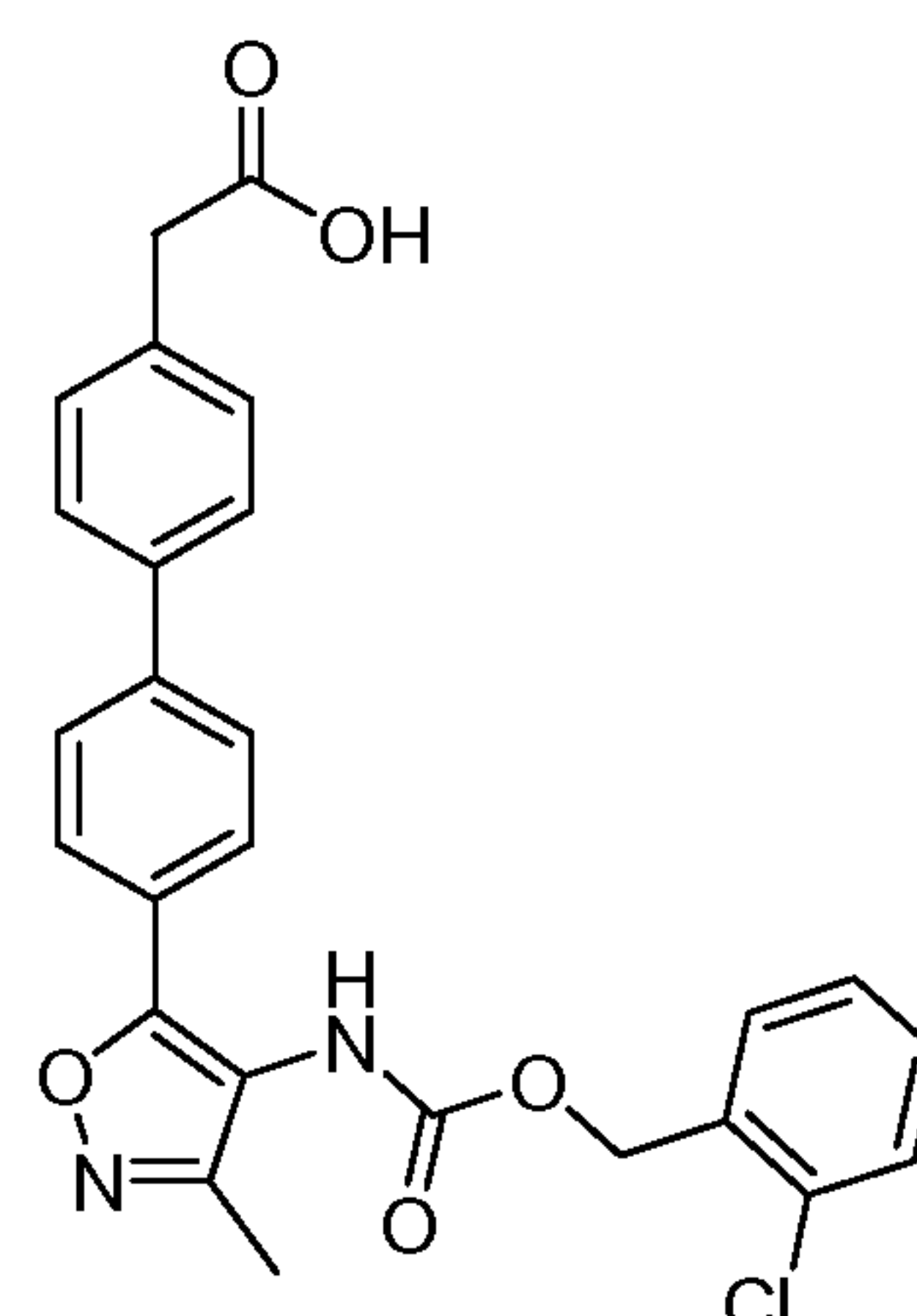
Compound 36
