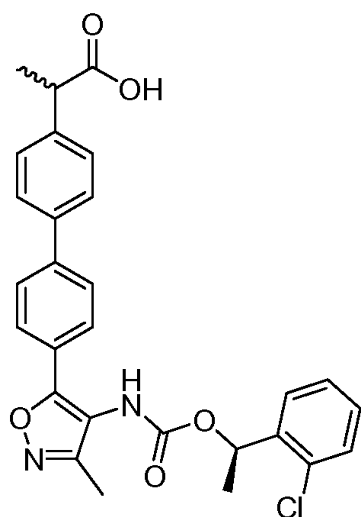
Compound 48
