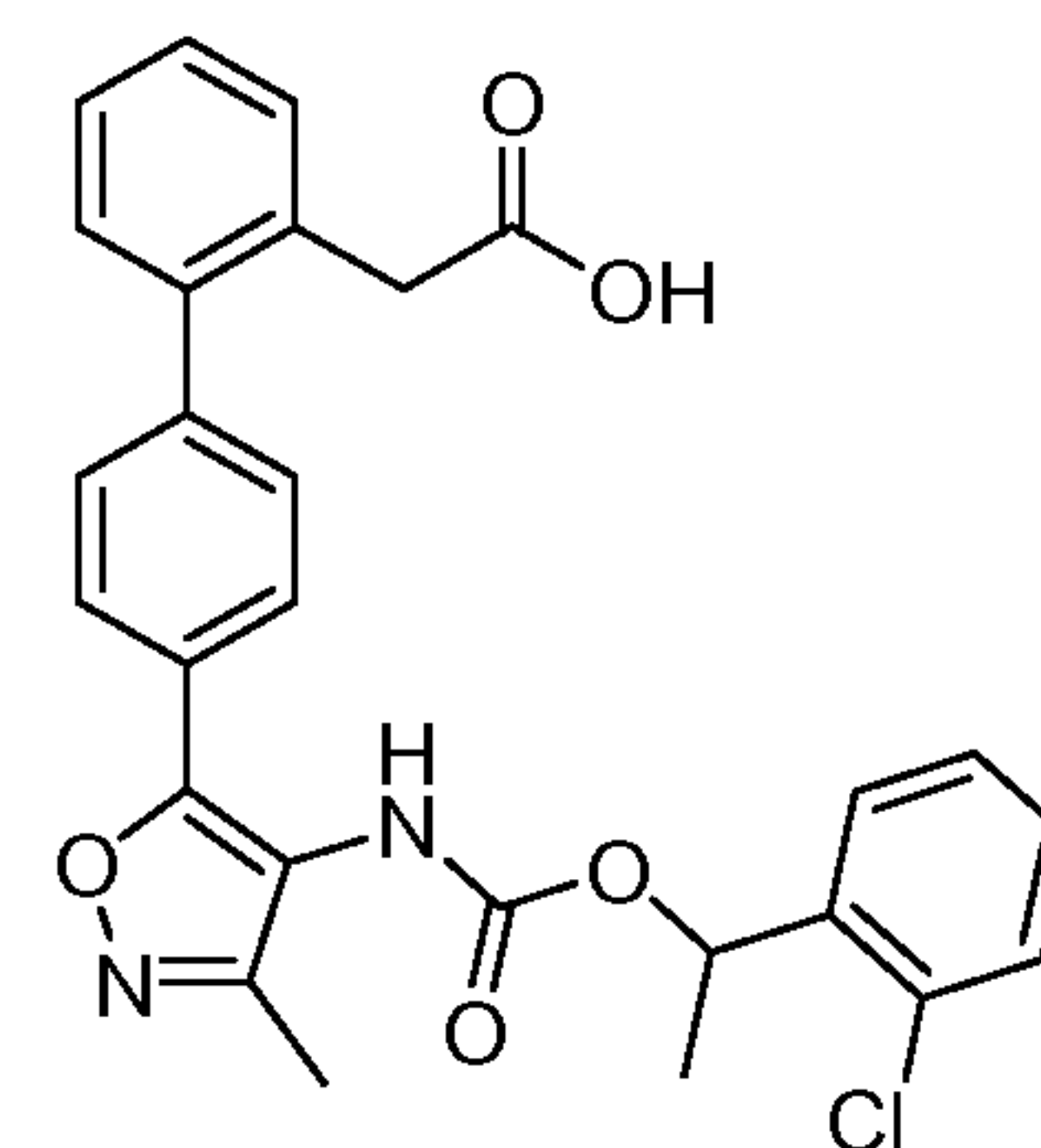
Compound 10
