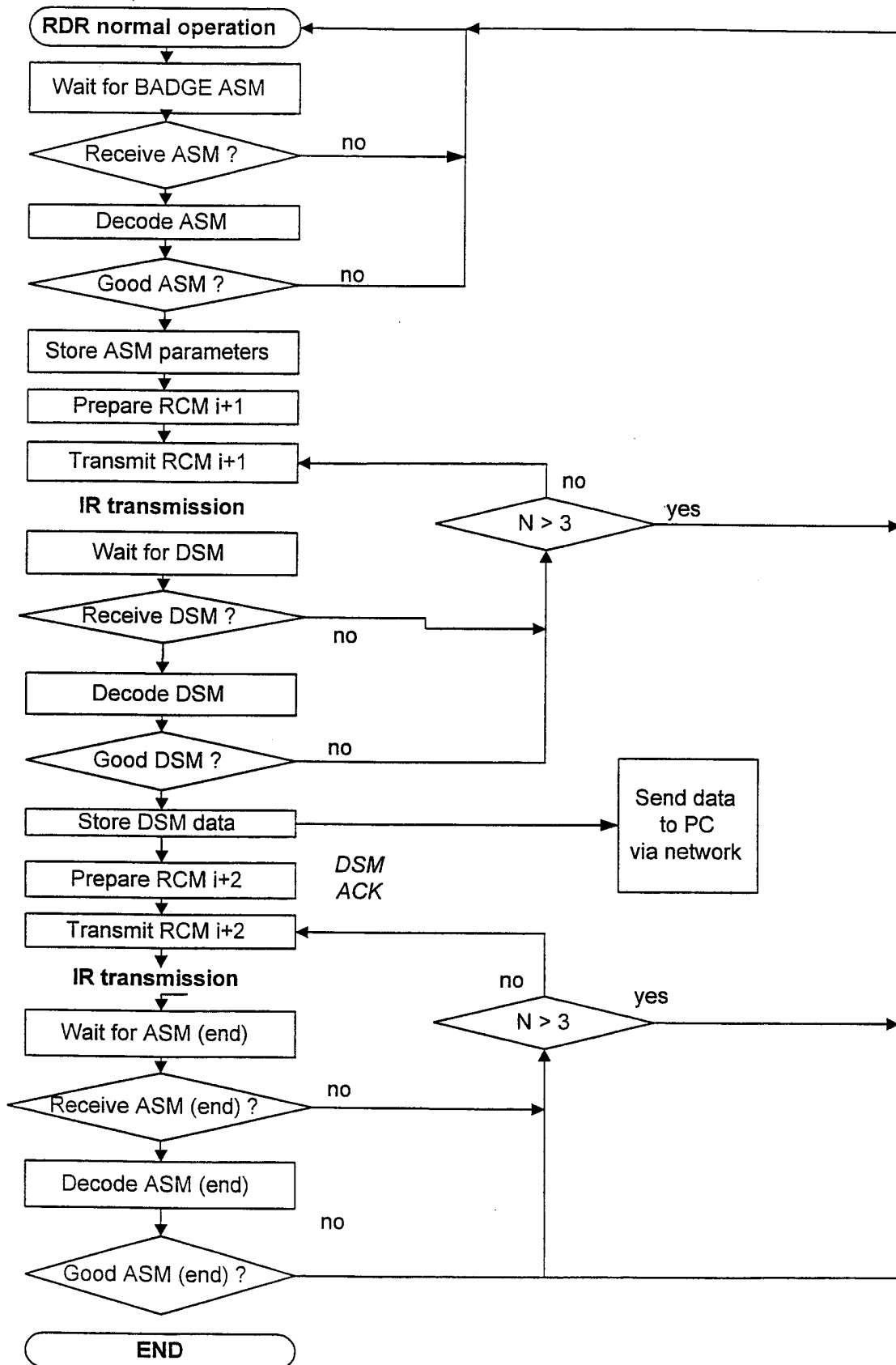
Fig 10a: Badge to RDR Long Message Transmission Protocol RDR Flow Chart
