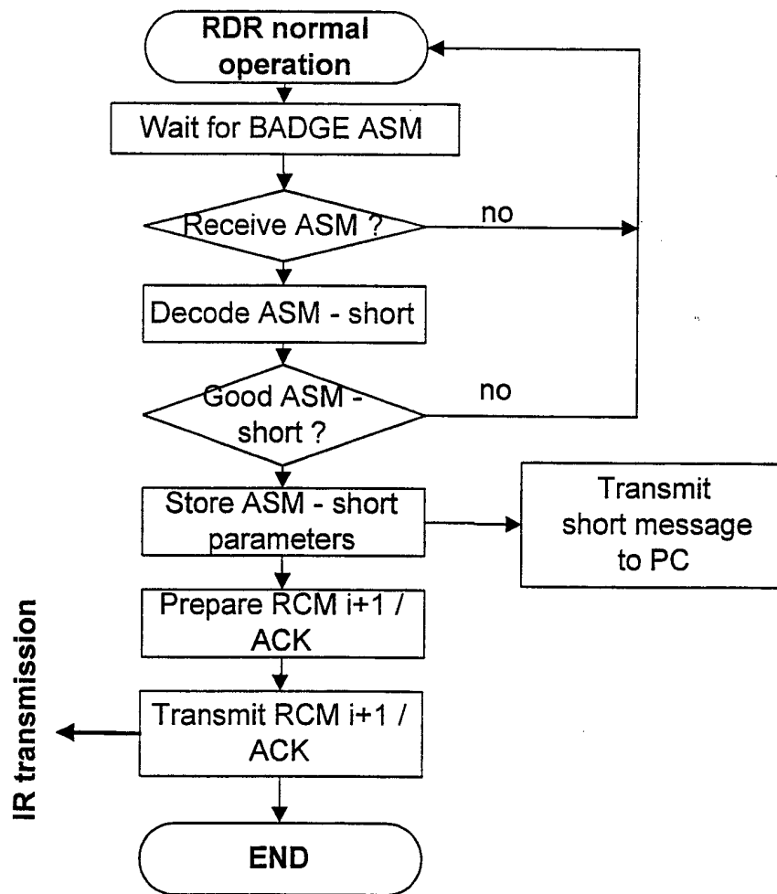
Fig 11a: Badge to RDR Short / Location Message Transmission Protocol RDR Flow Chart
