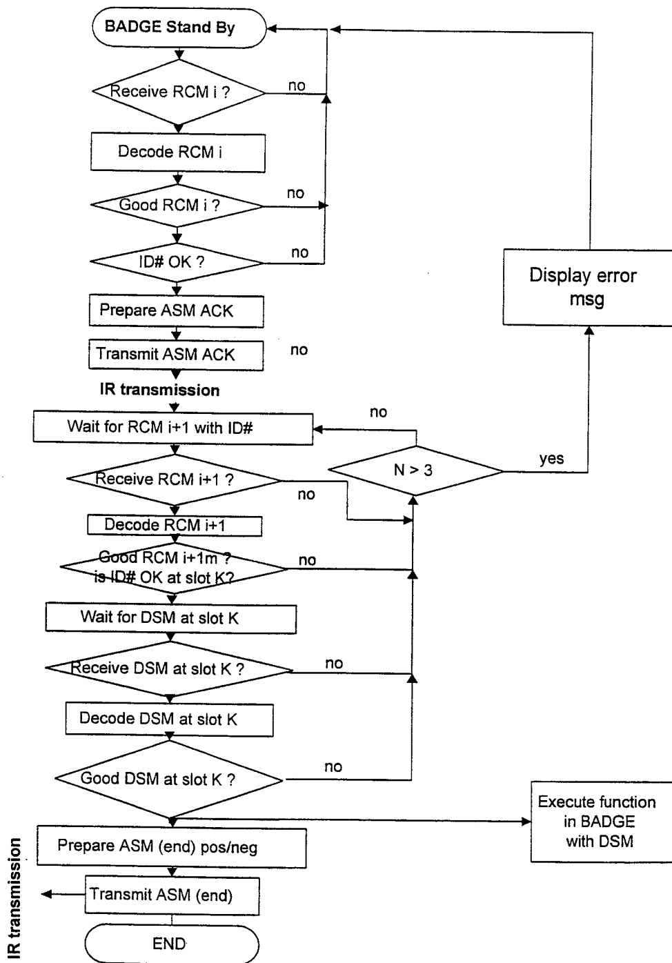
Fig 9b: RDR to BADGE Long Message Transmission Protocol BADGE Flow Chart
