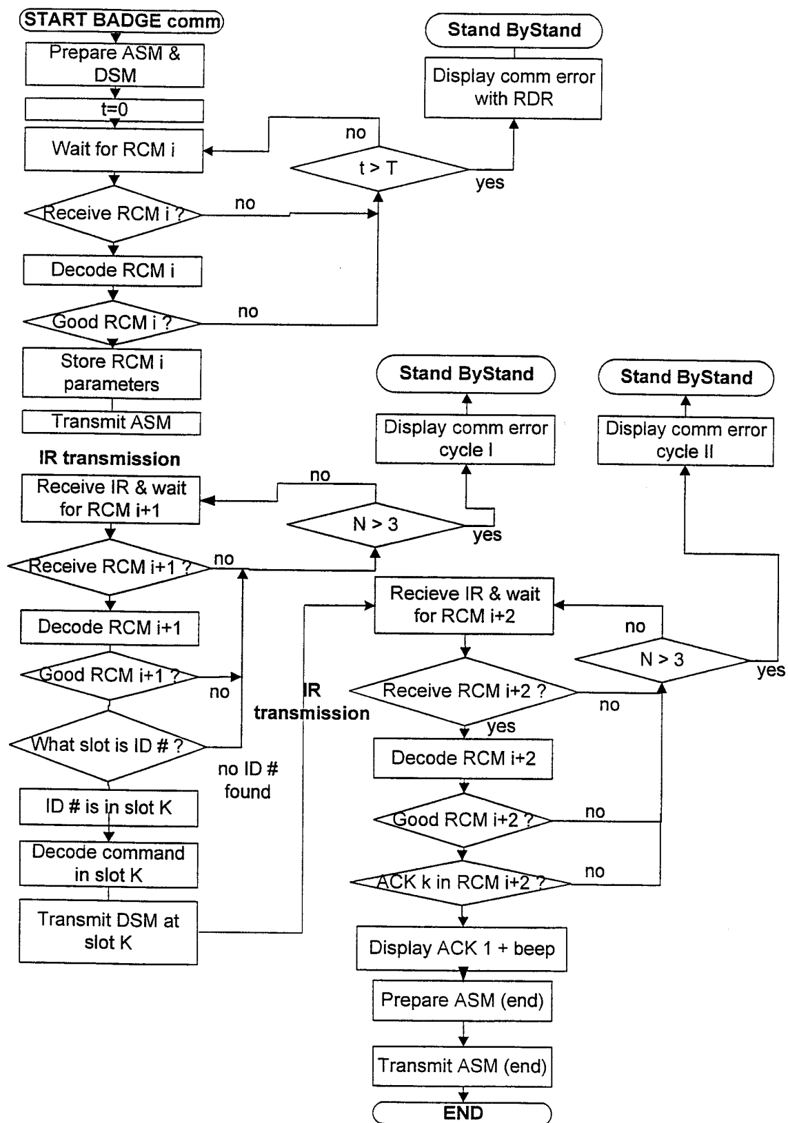
Fig 10b: Badge to RDR Long Message Transmission Protocol BADGE Flow Chart
