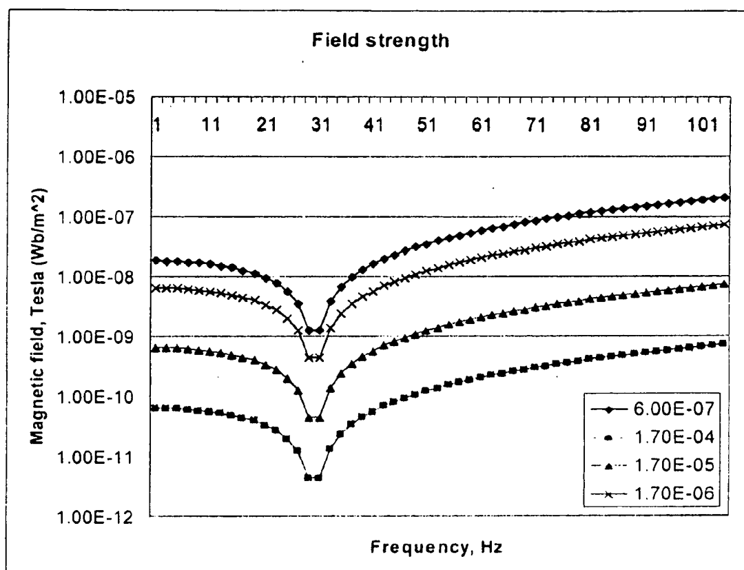
Fig. 9 Magnetic field strength required to create 15 nm displacement. Field is plotted as a function of driving frequency at various values of resting current.
