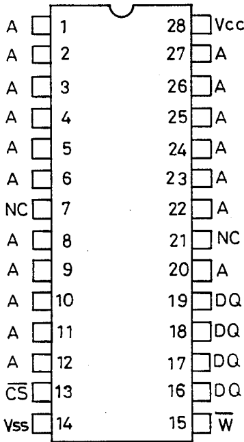
256K X 4 ORGANIZATION
