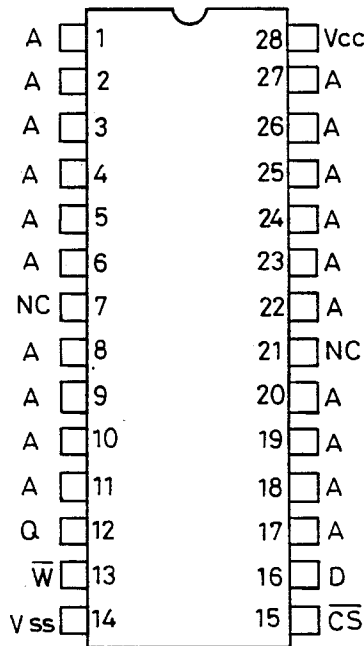
1M X 1 ORGANIZATION
