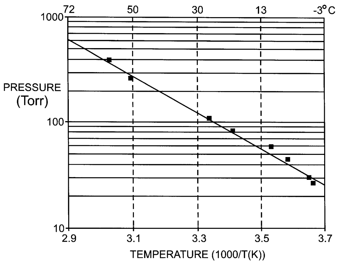
Hhfac VAPOR PRESSURE VS INVERSE TEMPERATURE
