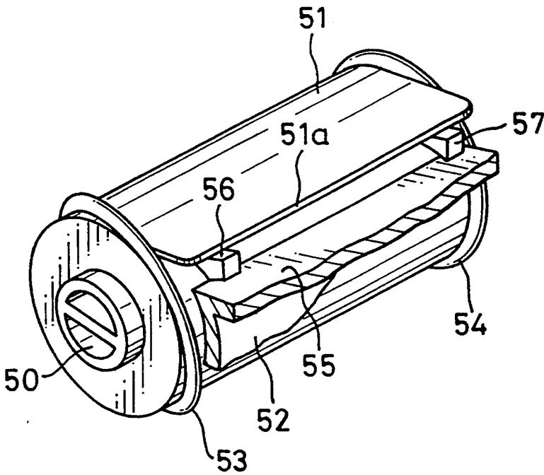
FIG. 12 (PRIOR ART)
