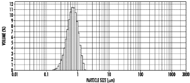
PARTICLE SIZE DISTRIBUTION -- 5% TP6S
